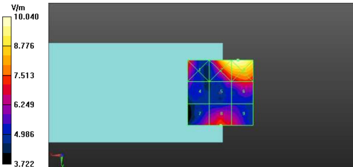
Fig A.17 HAC RF E-Field LTE-Band 41 High-2
