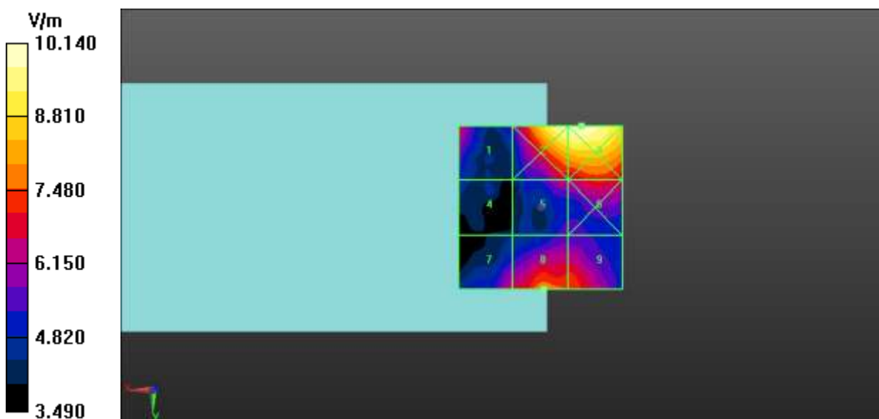
Fig A.18 HAC RF E-Field LTE-Band 41 Middle
