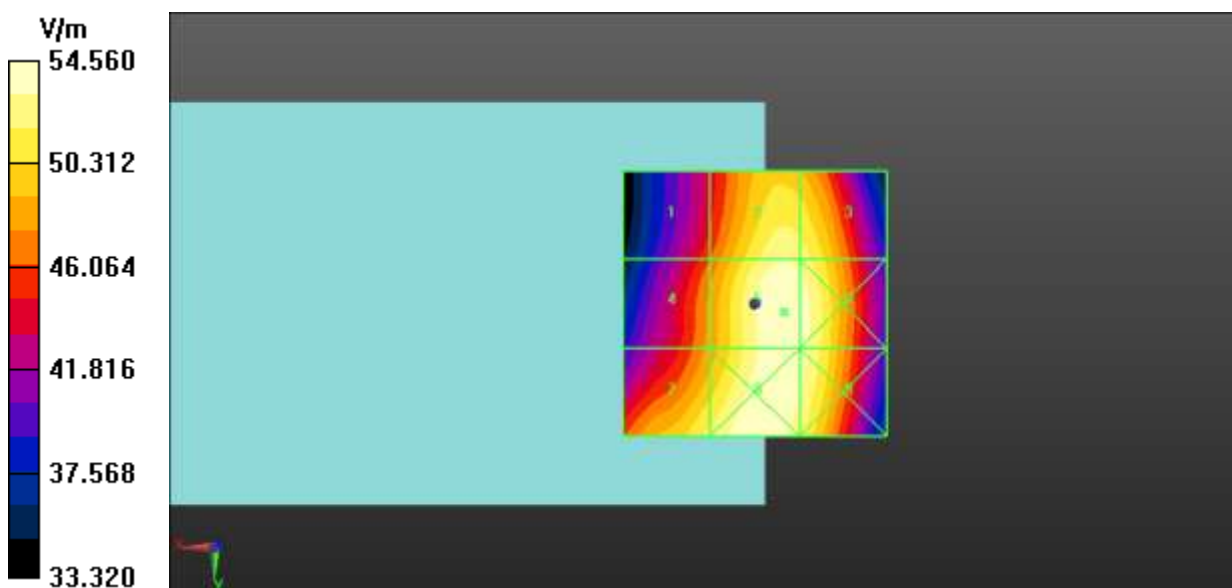
Fig A.14 HAC RF E-Field CDMA BC10
