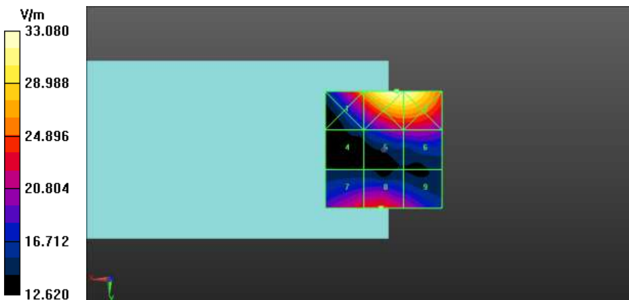
Fig A.11 HAC RF E-Field CDMA BC1
