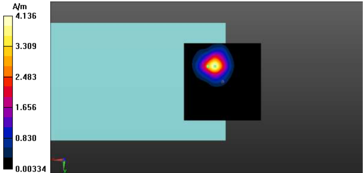
Fig A.33 T-Coil LTE-Band 2-Z
