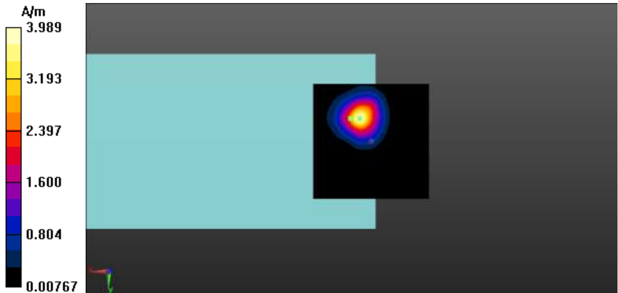
Fig A.41 T-Coil LTE-Band 41-Z
