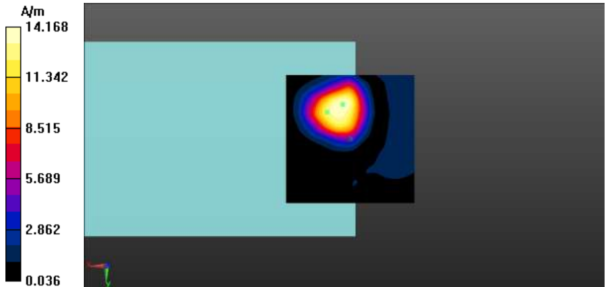
Fig A.12 T-Coil LTE-Band 7-Z
