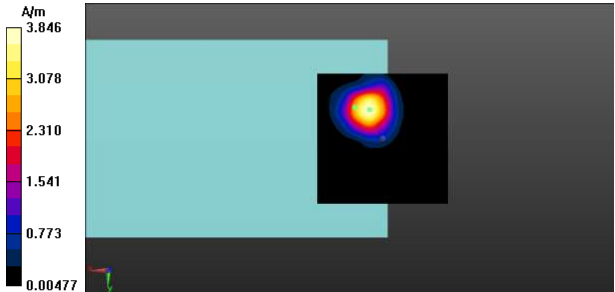
Fig A.38 T-Coil LTE-Band 13-Z
