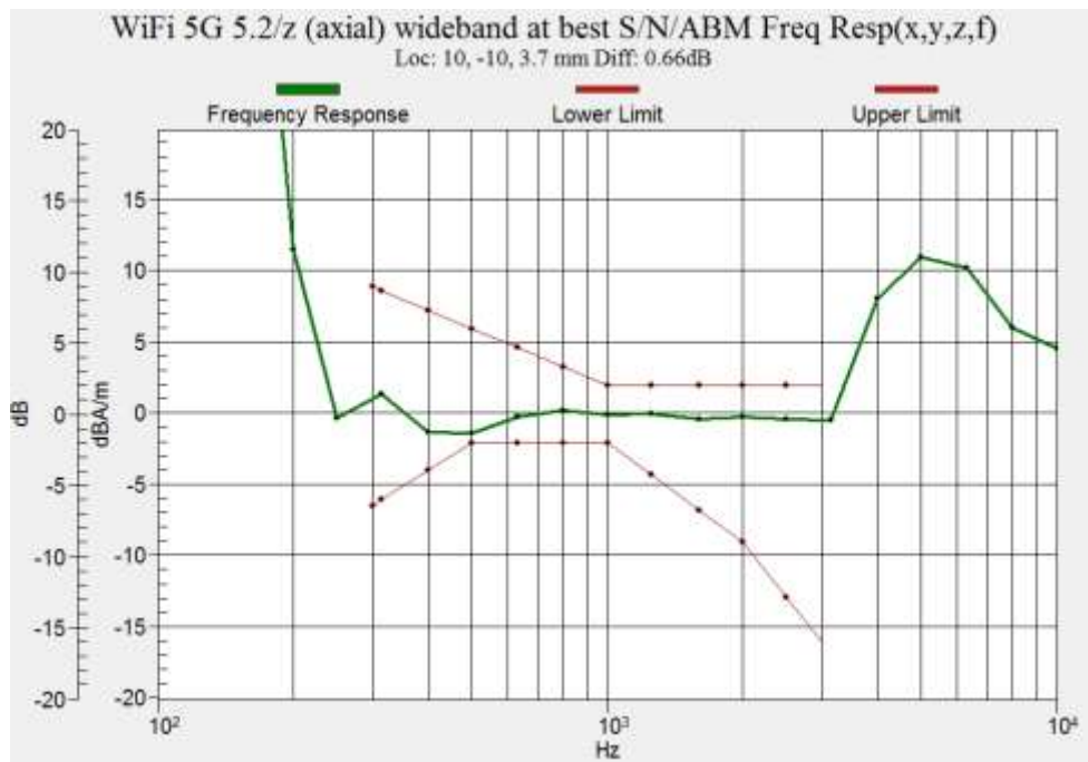
Figure B.45 Frequency Response of WIFI 5.2G (Google Duo)
