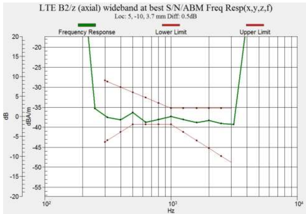
Figure B.33 Frequency Response of LTE B2 (Google Duo)
