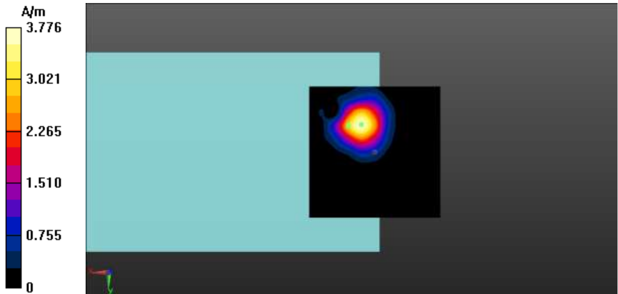
Fig A.35 T-Coil LTE-Band 5-Z
