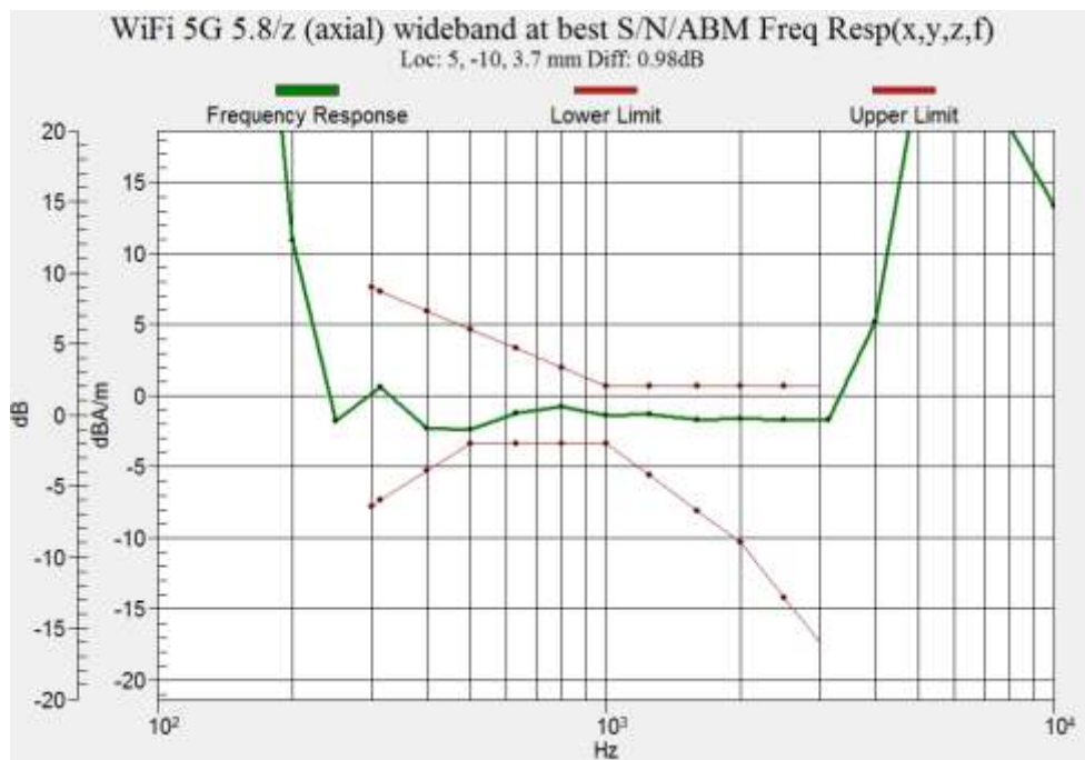
Figure B.48 Frequency Response of WIFI 5.8G (Google Duo)
