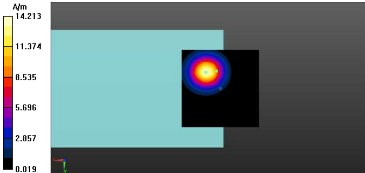
Fig A.16 T-Coil LTE-Band 26-Z
