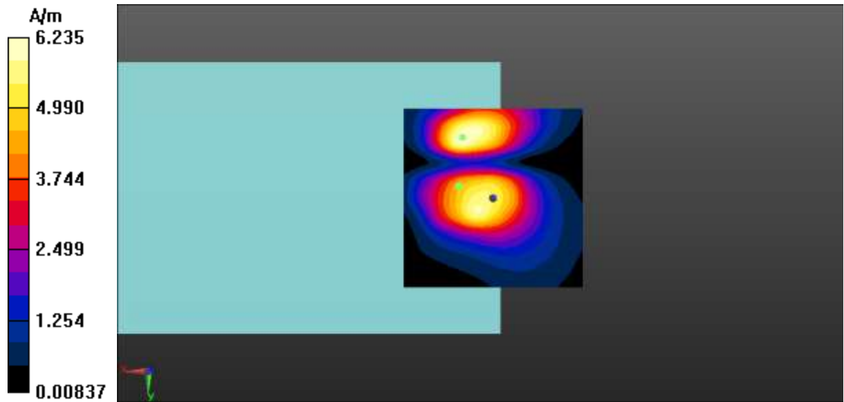
Fig A.16 T-Coil LTE-Band 26-Y
