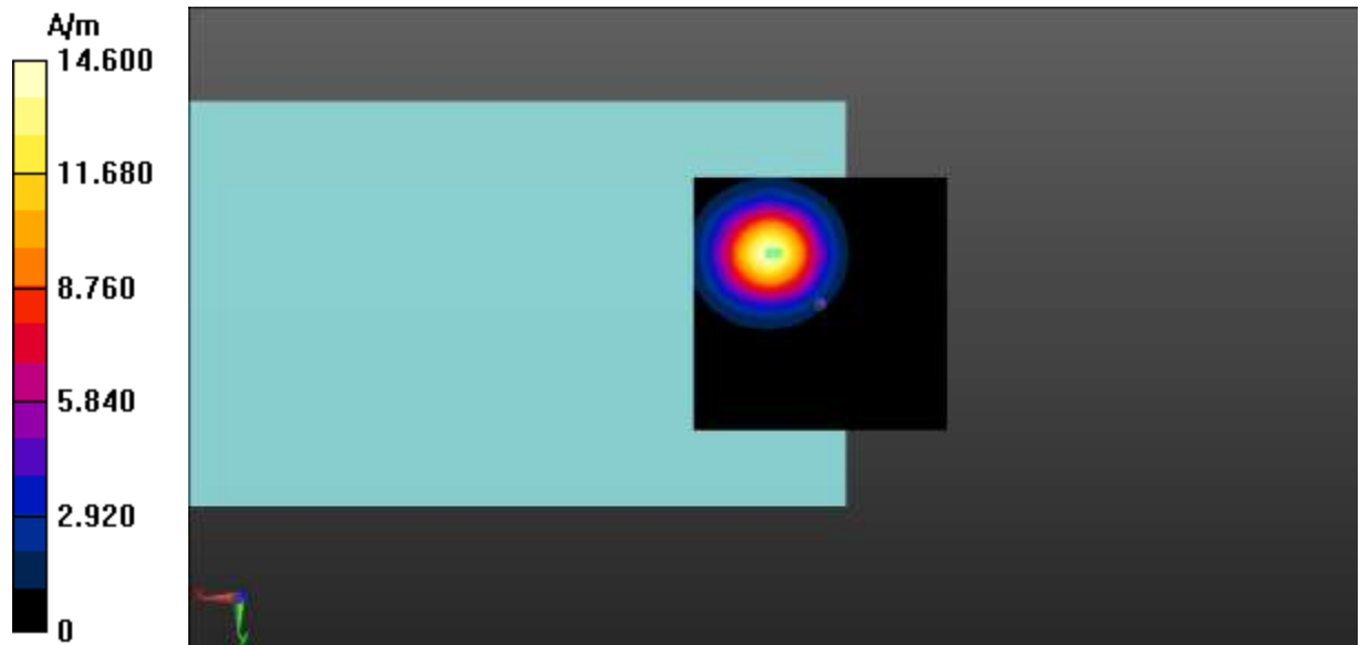
Fig A.3 T-Coil CDMA BC0-Z
