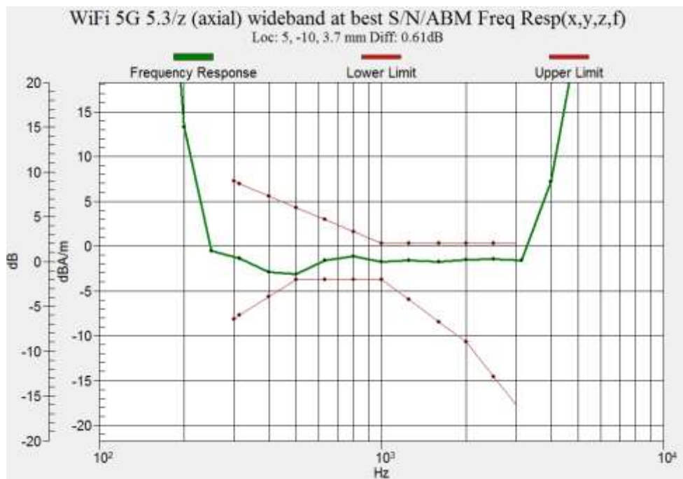
Figure B.46 Frequency Response of WIFI 5.3G (Google Duo)
