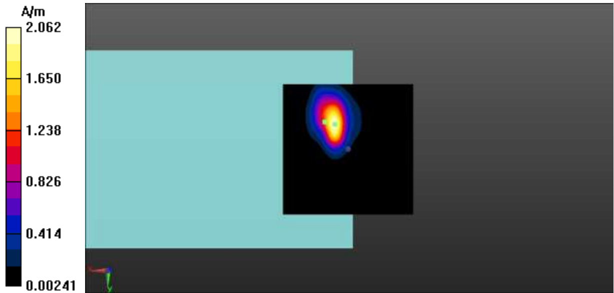
Fig A.20 T-Coil WIFI 2.4G-Z
