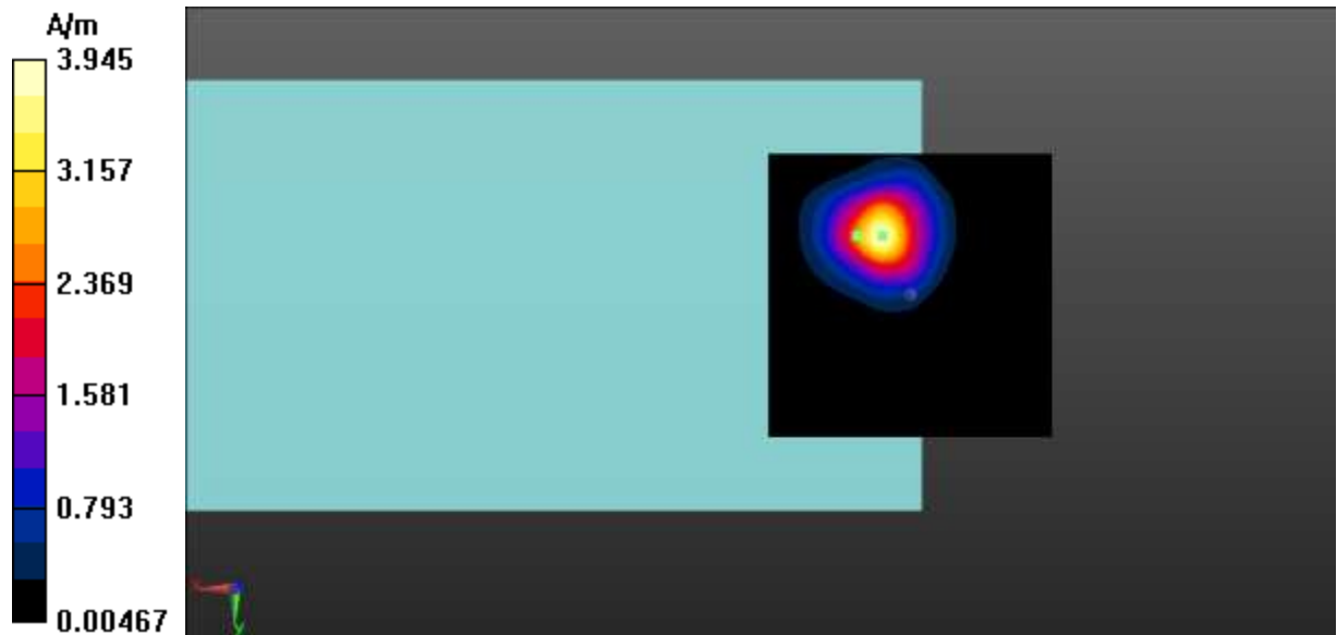
Fig A.42 T-Coil LTE-Band 66-Z
