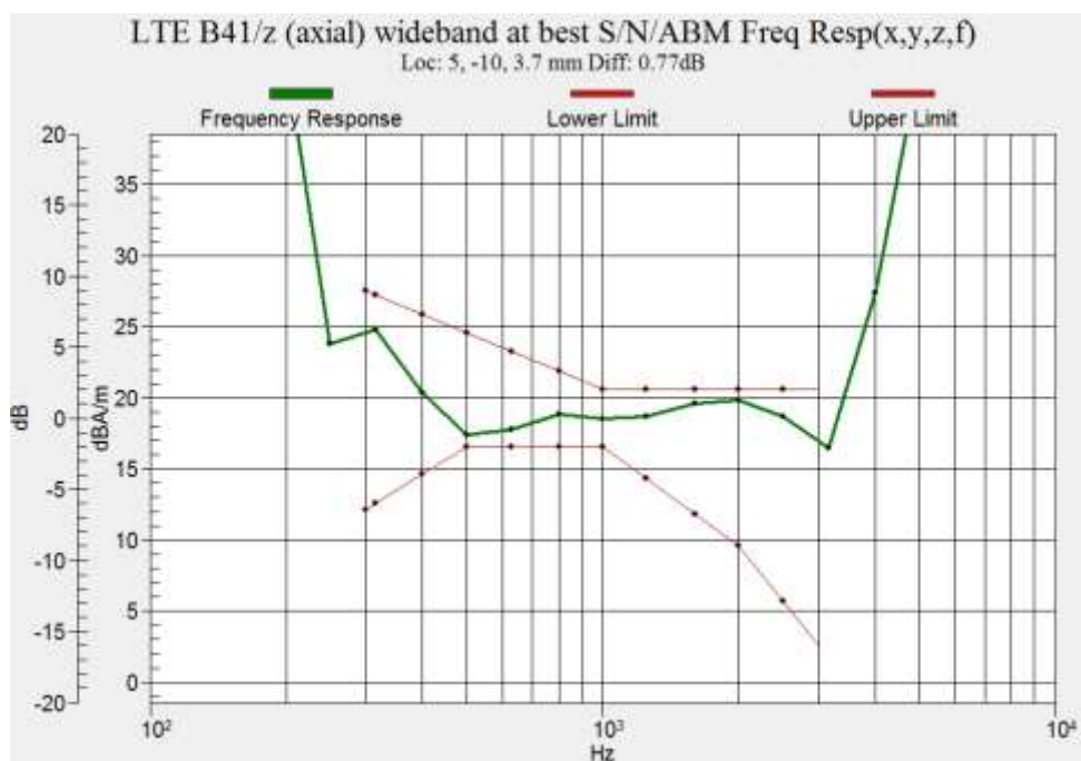
Figure B.41 Frequency Response of LTE B41 (Google Duo)
