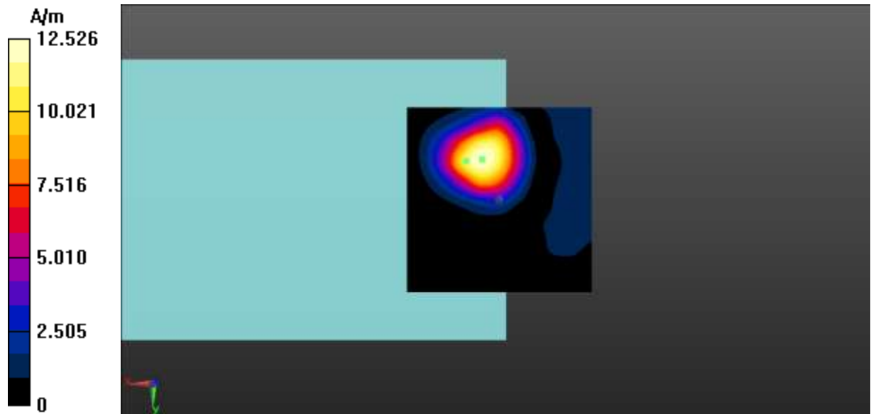
Fig A.18 T-Coil LTE-Band 71-Z
