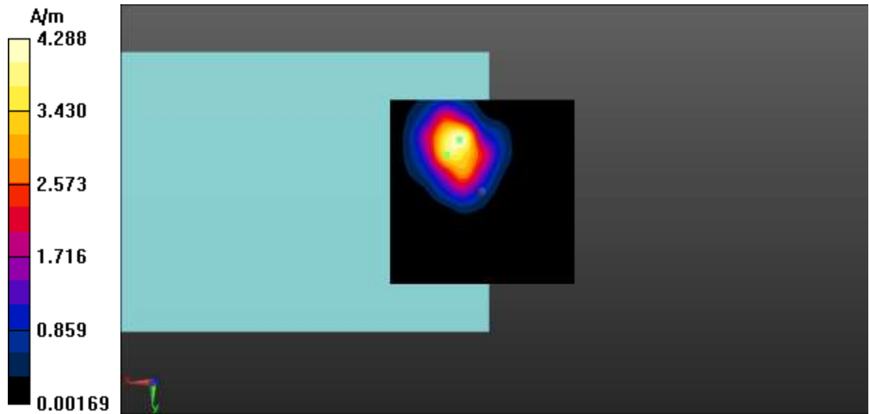
Fig A.44 T-Coil WIFI 2.4G-Z
