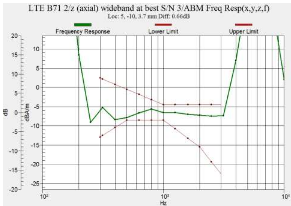
Figure B.43 Frequency Response of LTE B71 (Google Duo)
