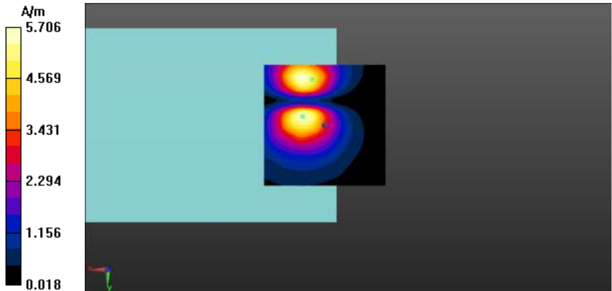
Fig A.4 T-Coil CDMA BC1-Y
