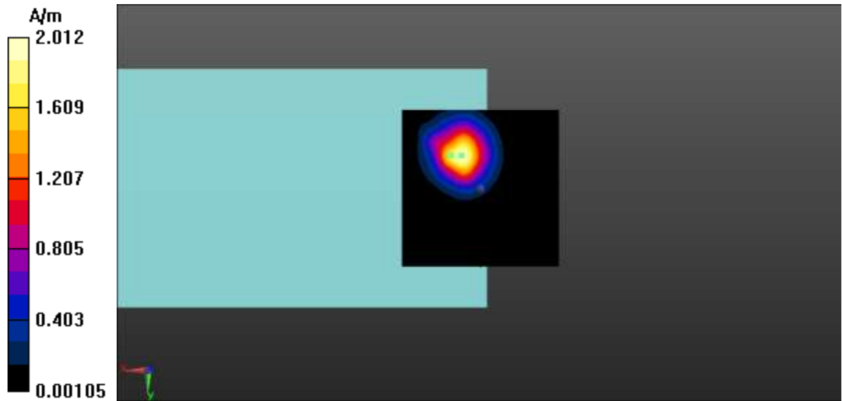
Fig A.23 T-Coil WIFI 5.5G-Z
