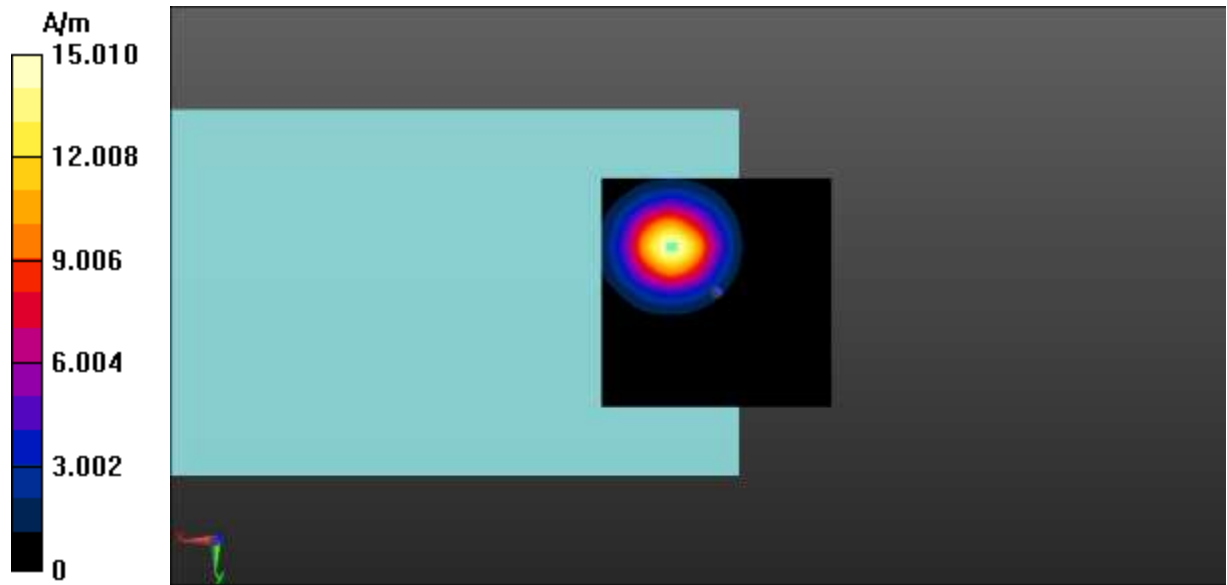
Fig A.4 T-Coil CDMA BC1-Z
