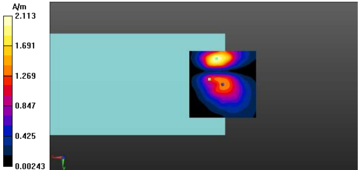
Fig A.35 T-Coil LTE-Band 5-Y
