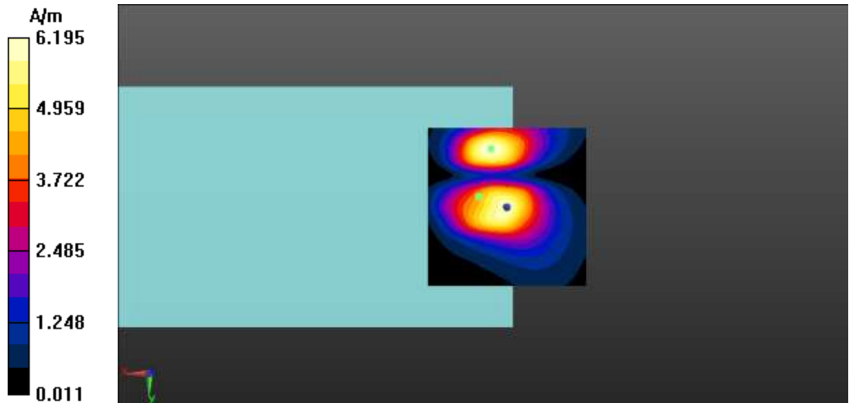
Fig A.19 T-Coil LTE-Band 41-Y
