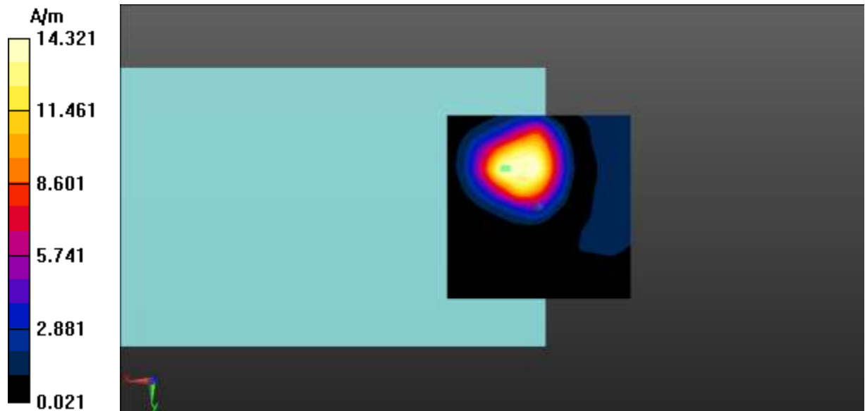
Fig A.14 T-Coil LTE-Band 13-Z
