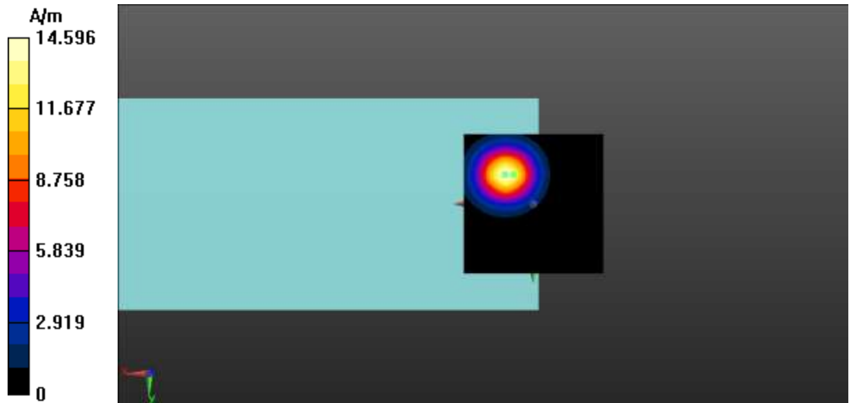
Fig A.26 T-Coil GSM 1900-Z
