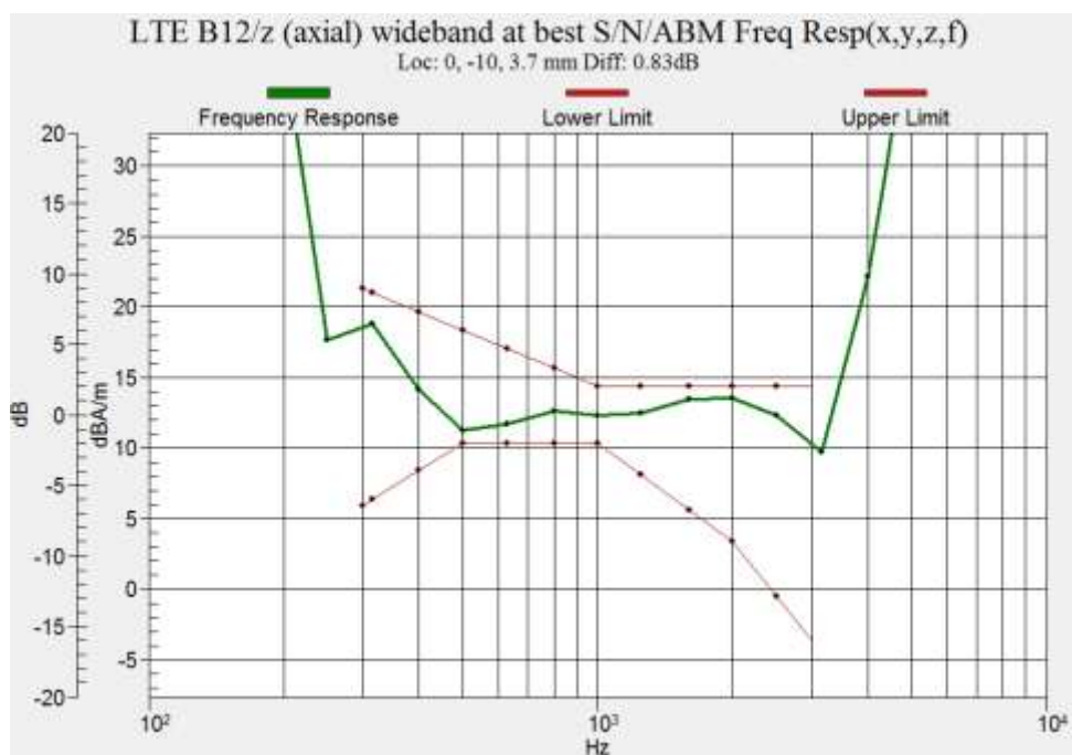
Figure B.13 Frequency Response of W LTE B12
