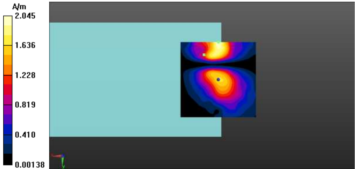
Fig A.48 T-Coil WIFI 5.8G-Y
