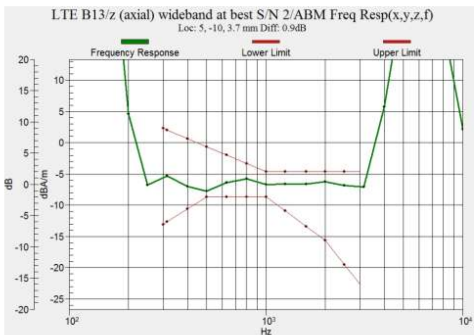
Figure B.38 Frequency Response of LTE B13 (Google Duo)
