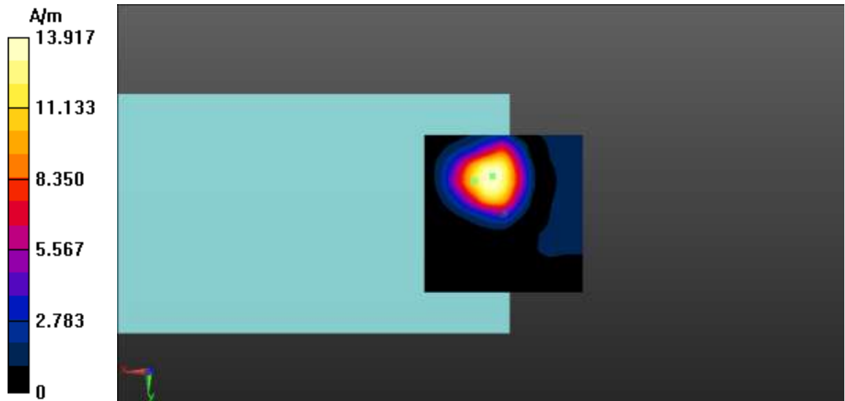
Fig A.17 T-Coil LTE-Band 66-Z
