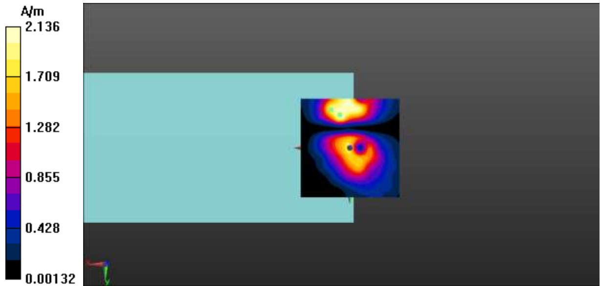
Fig A.46 T-Coil WIFI 5.3G-Y
