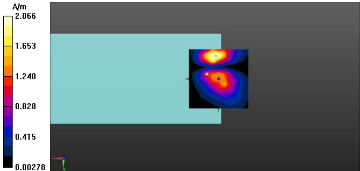
Fig A.34 T-Coil LTE-Band 4-Y
