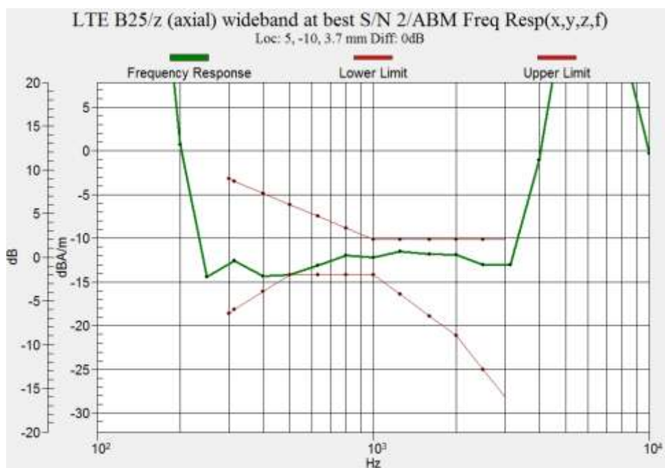
Figure B.39 Frequency Response of LTE B25 (Google Duo)
