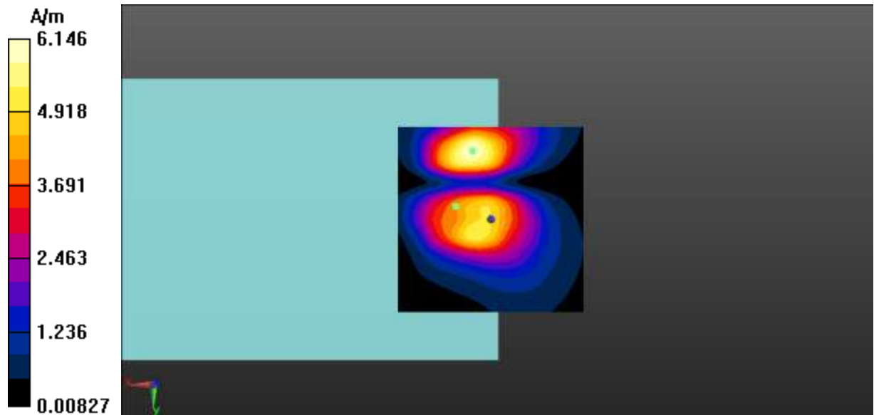
Fig A.15 T-Coil LTE-Band 25-Y
