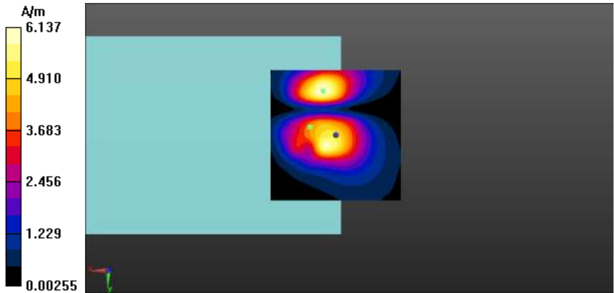
Fig A.9 T-Coil LTE-Band 2-Y
