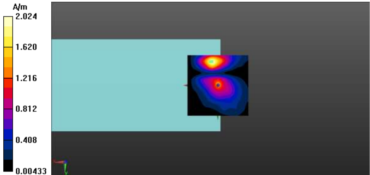
Fig A.40 T-Coil LTE-Band 26-Y
