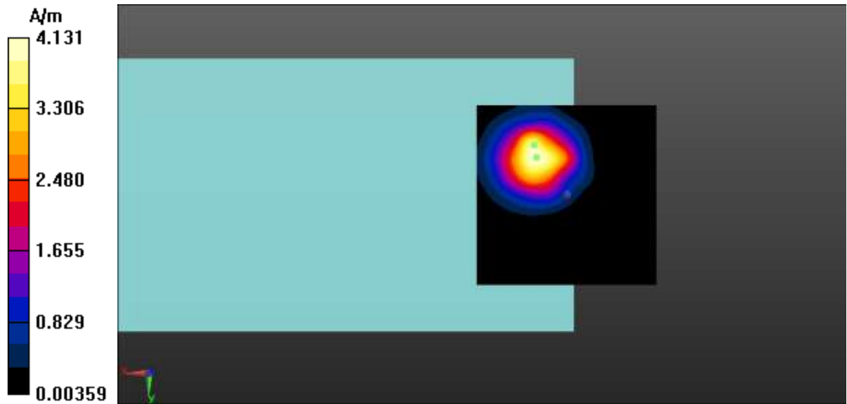
Fig A.47 T-Coil WIFI 5.5G-Z
