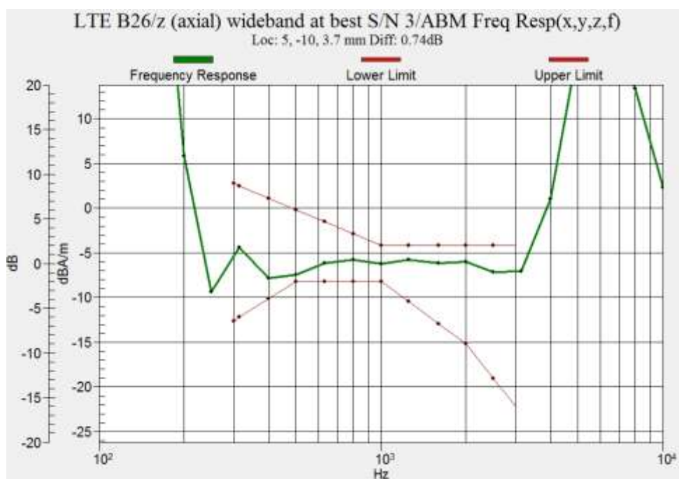
Figure B.40 Frequency Response of LTE B26 (Google Duo)
