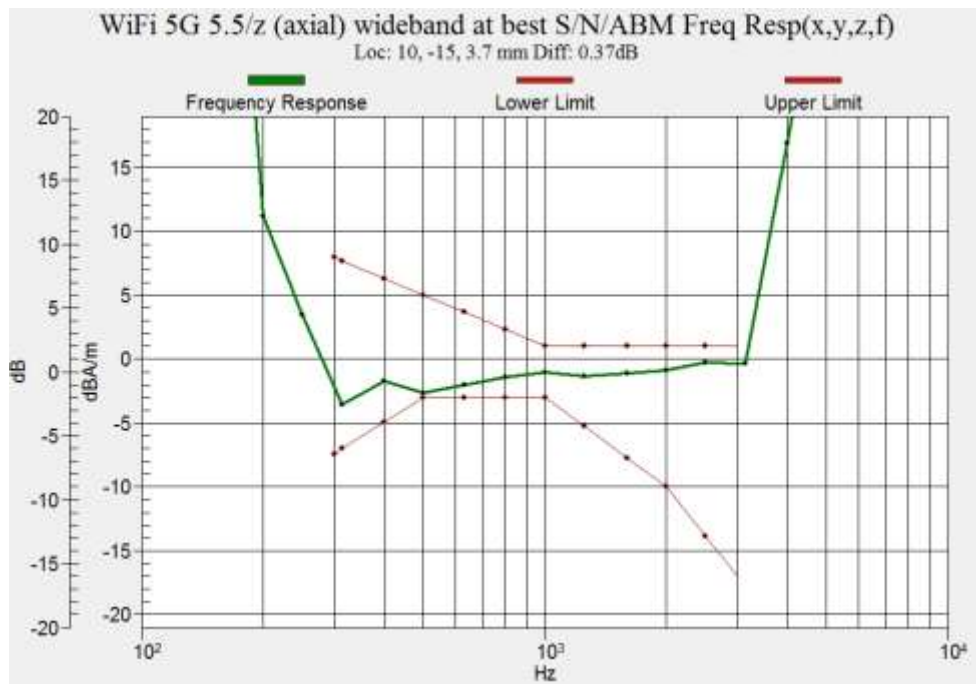
Figure B.47 Frequency Response of WIFI 5.5G (Google Duo)
