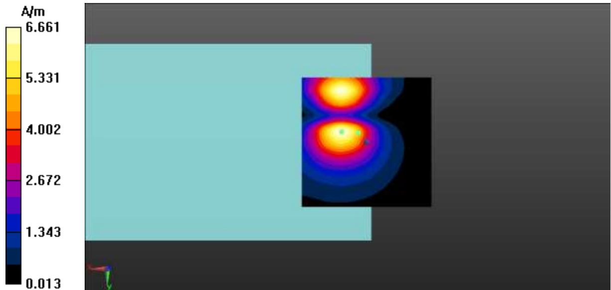
Fig A.2 T-Coil GSM 1900-Y
