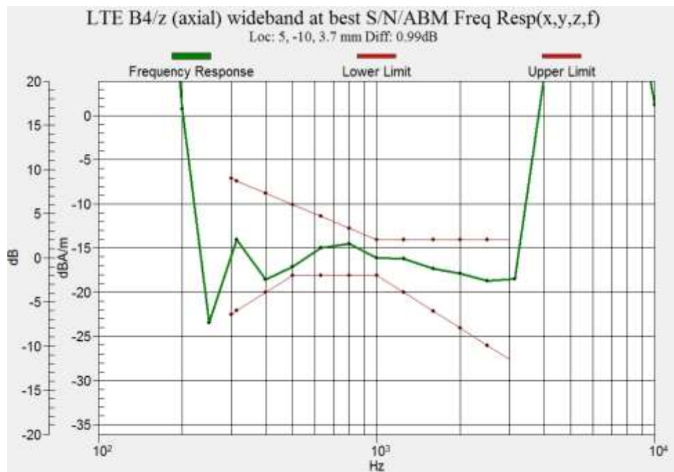
Figure B.34 Frequency Response of LTE B4 (Google Duo)
