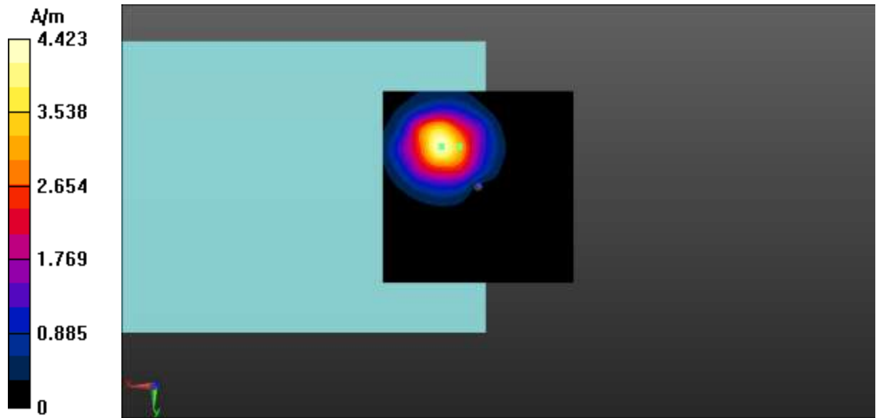
Fig A.40 T-Coil LTE-Band 26-Z
