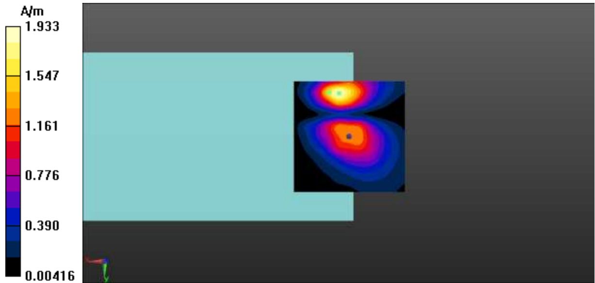
Fig A.41 T-Coil LTE-Band 41-Y
