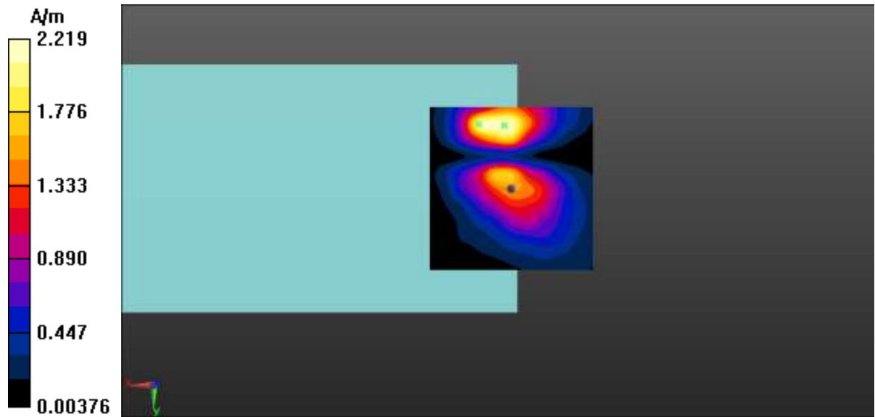
Fig A.38 T-Coil LTE-Band 13-Y
