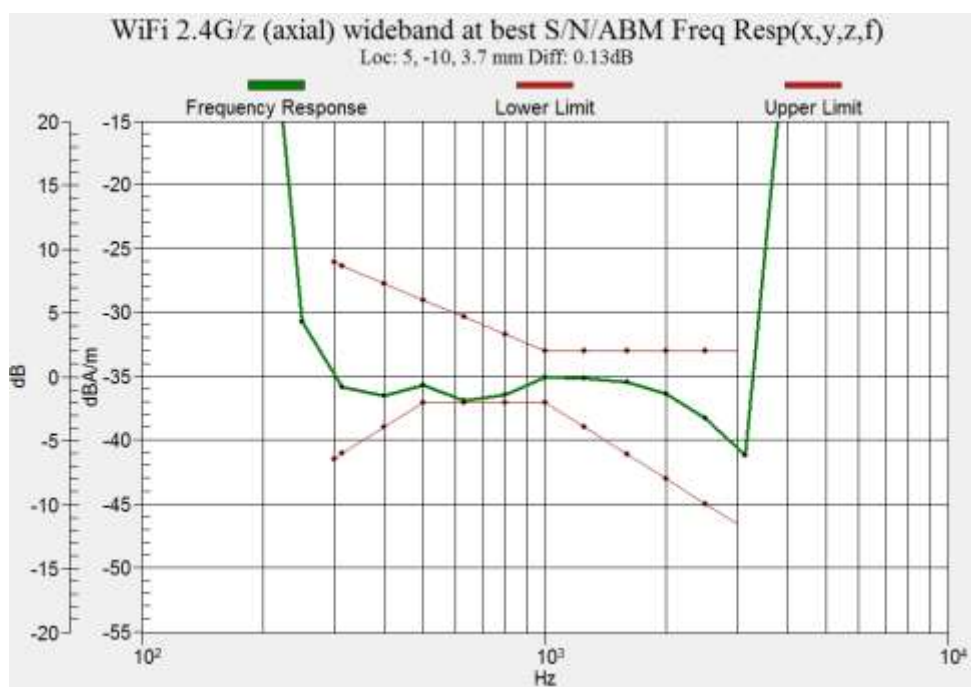
Figure B.20 Frequency Response of WIFI 2.4G
