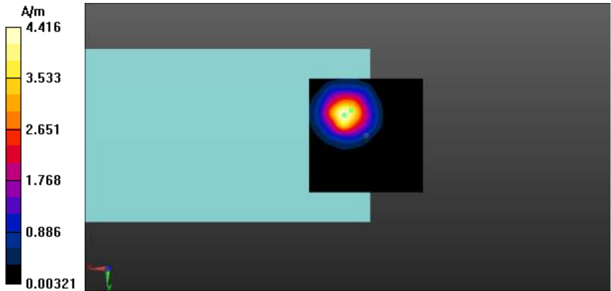
Fig A.48 T-Coil WIFI 5.8G-Z
