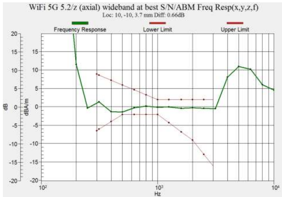
Figure B.21 Frequency Response of WIFI 5.2G
