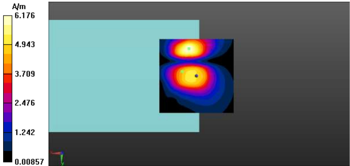
Fig A.14 T-Coil LTE-Band 13-Y
