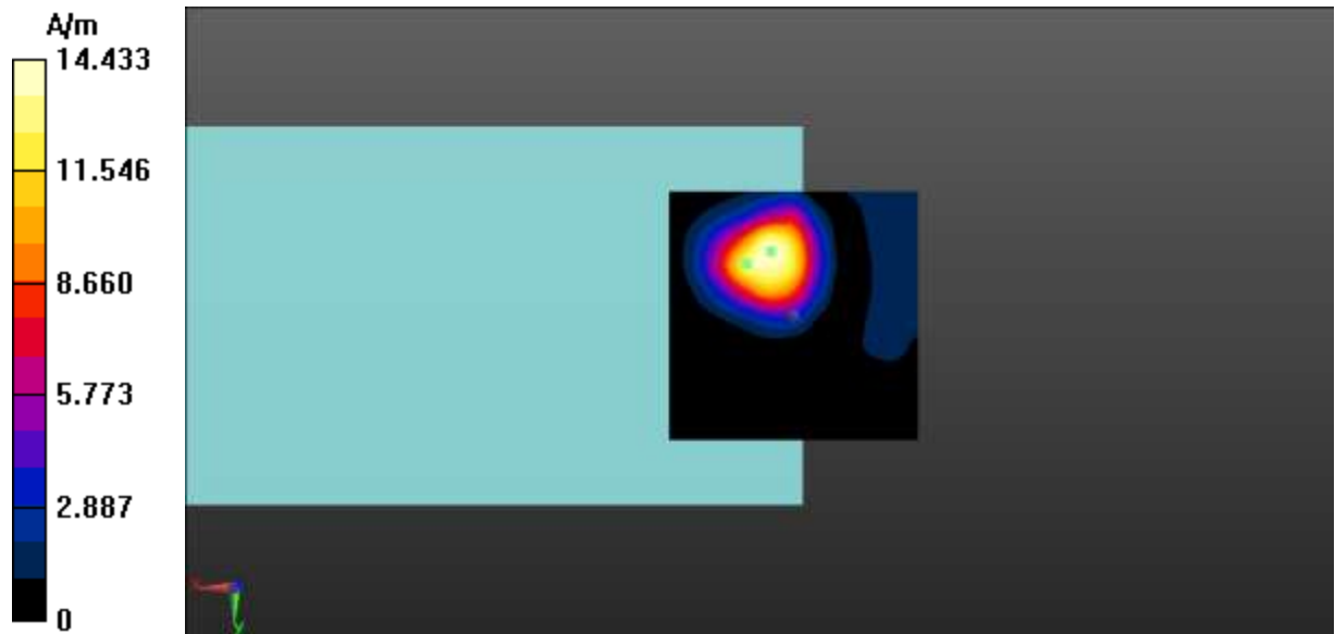
Fig A.9 T-Coil LTE-Band 2-Z
