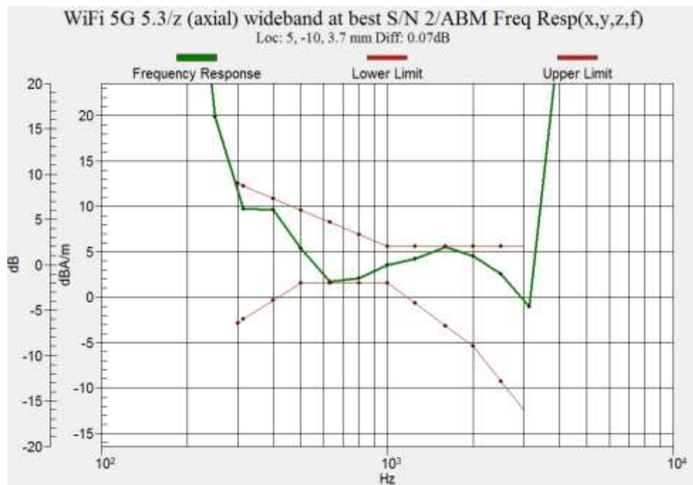
Figure B.22 Frequency Response of WIFI 5.3G
