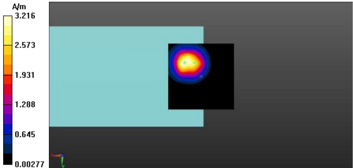
Fig A.36 T-Coil LTE-Band 7-Z
