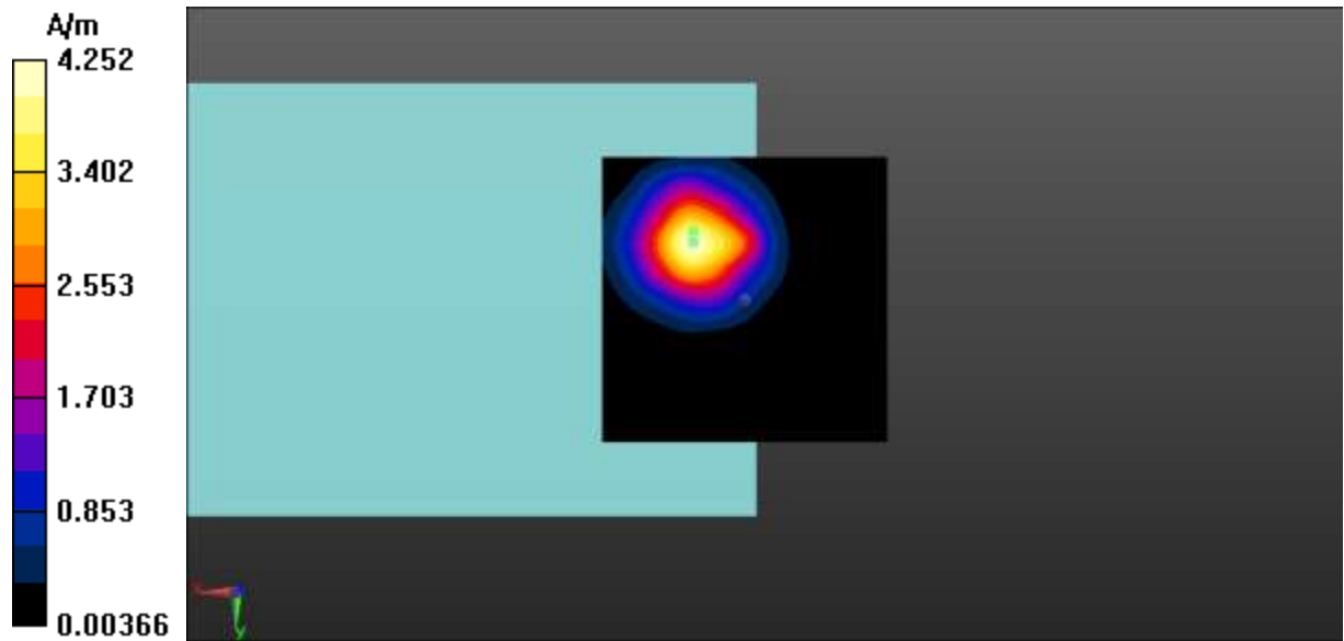
Fig A.45 T-Coil WIFI 5.2G-Z
