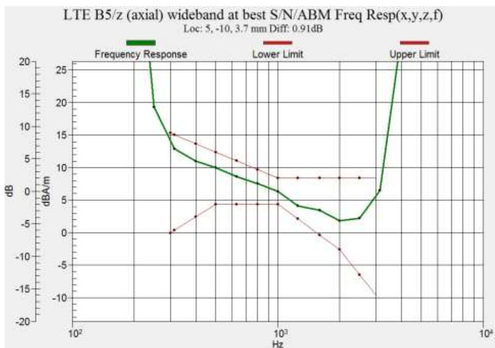
Figure B.35 Frequency Response of LTE B5 (Google Duo)
