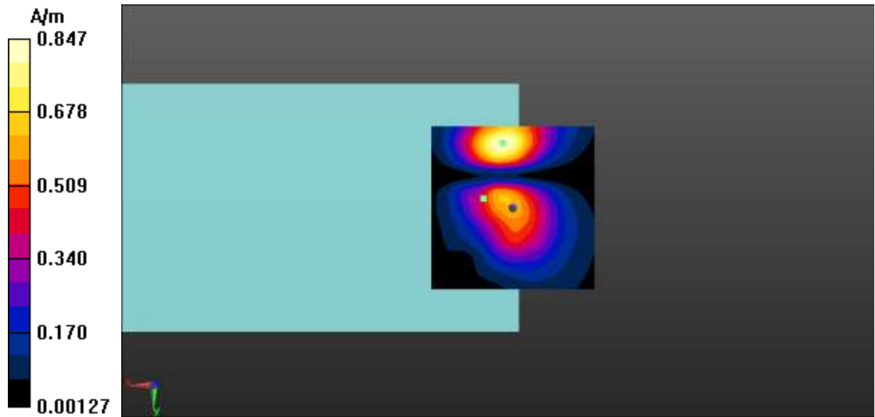
Fig A.21 T-Coil WIFI 5.2G-Y
