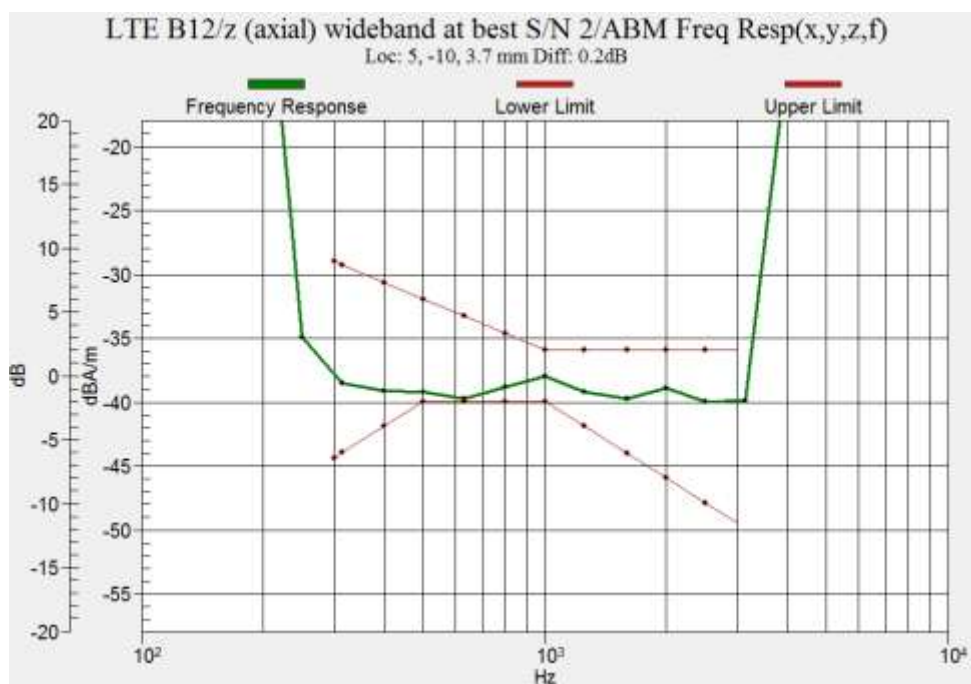
Figure B.37 Frequency Response of W LTE B12 (Google Duo)
