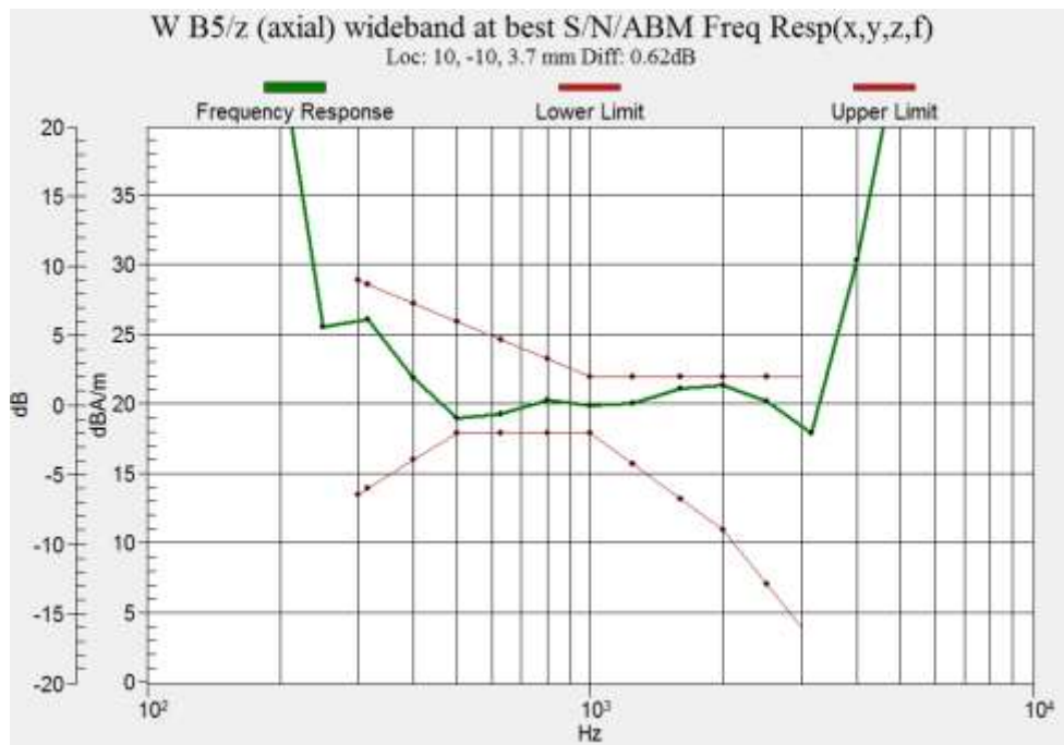
Figure B.32 Frequency Response of L WCDMA B5 (Google Duo)
