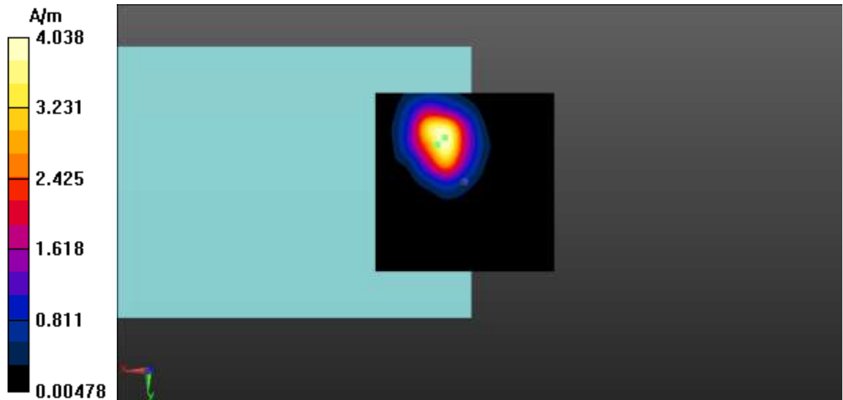
Fig A.46 T-Coil WIFI 5.3G-Z
