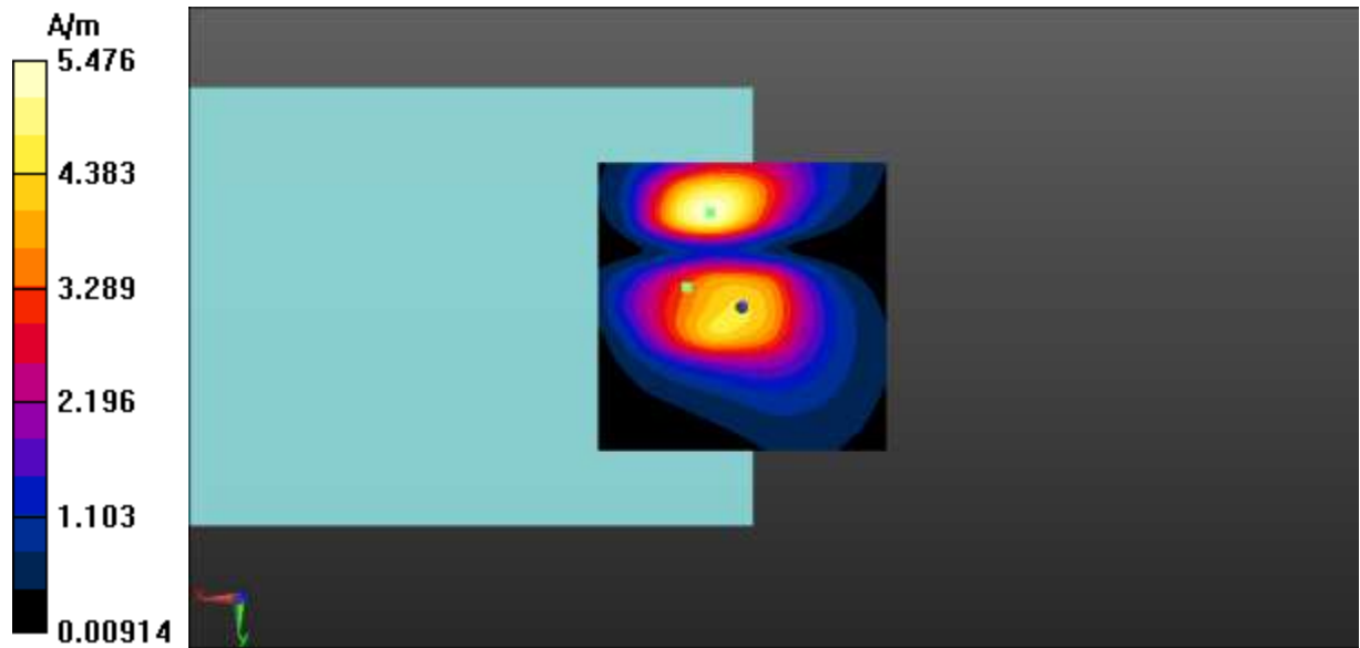
Fig A.18 T-Coil LTE-Band 71-Y
