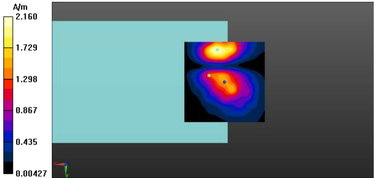
Fig A.39 T-Coil LTE-Band 25-Y
