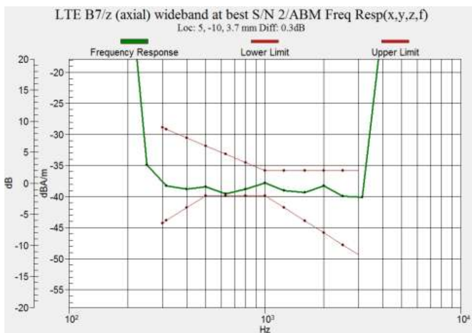
Figure B.36 Frequency Response of LTE B7 (Google Duo)
