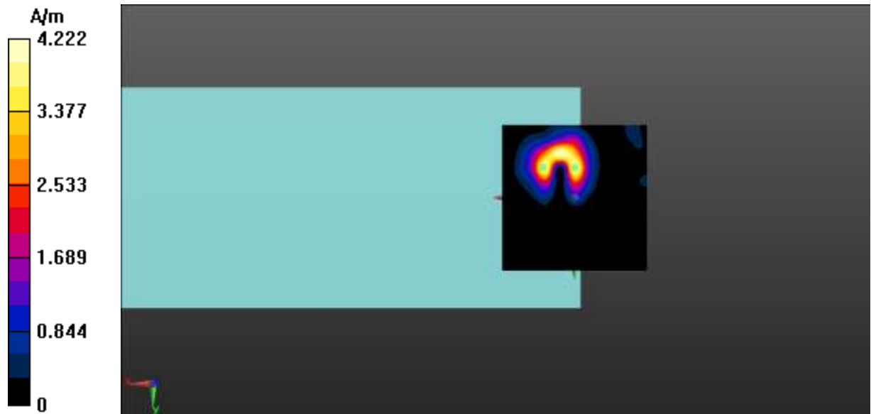
Fig A.43 T-Coil LTE-Band 71-Z
