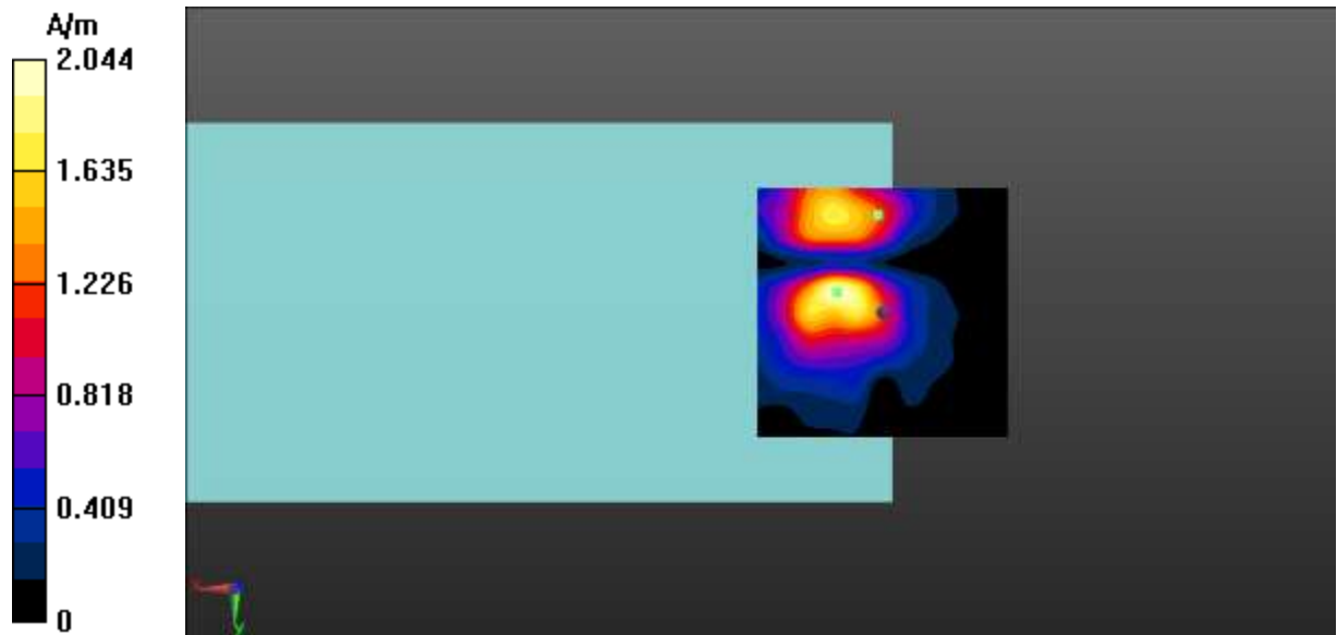
Fig A.33 T-Coil LTE-Band 2-Y
