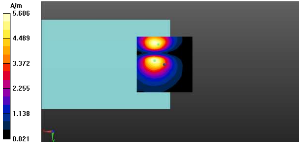
Fig A.29 T-Coil CDMA BC10-Y
