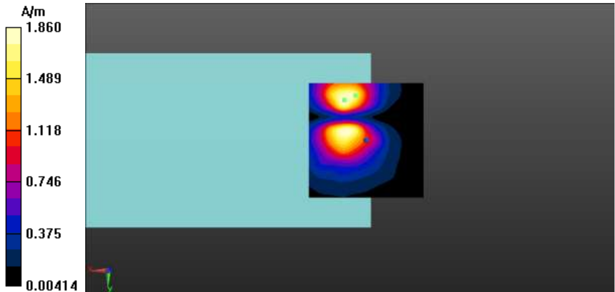
Fig A.42 T-Coil LTE-Band 66-Y
