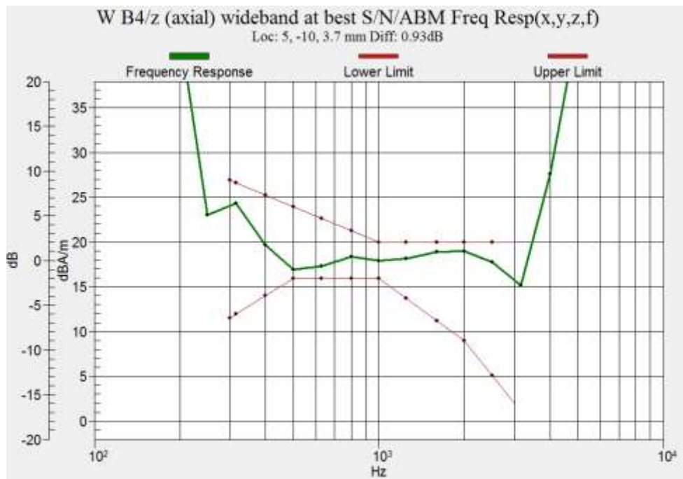
Figure B.31 Frequency Response of WCDMA B4 (Google Duo)
