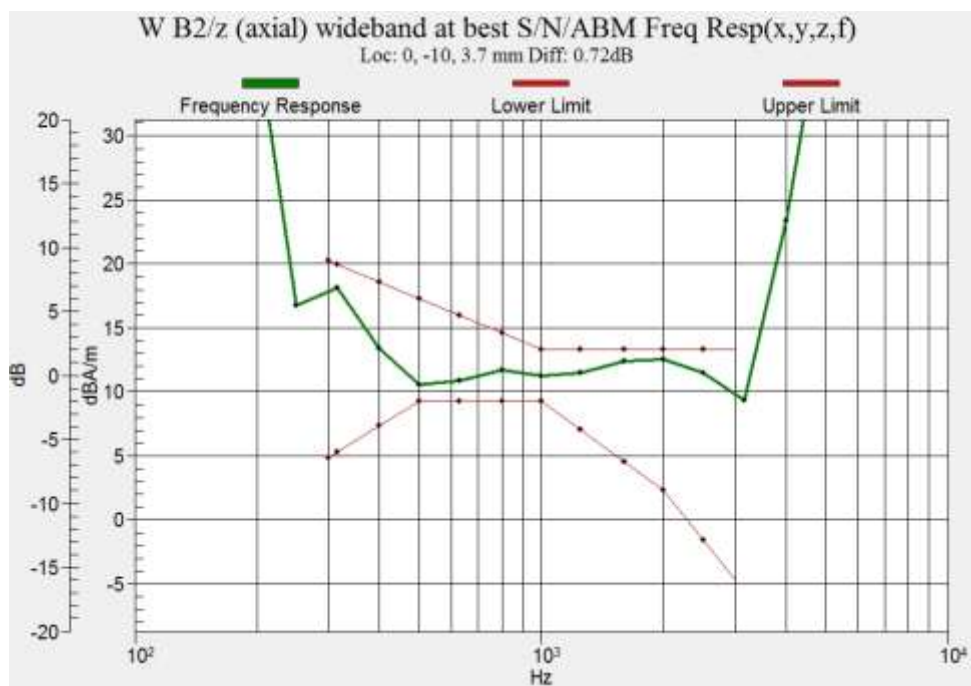
Figure B.30 Frequency Response of WCDMA B2 (Google Duo)
