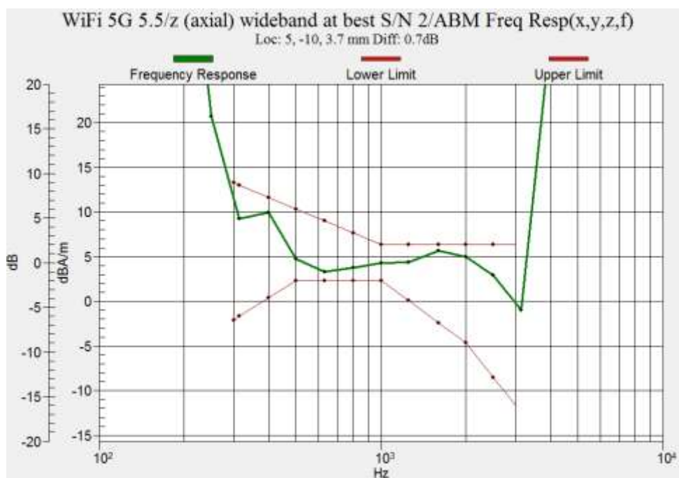
Figure B.23 Frequency Response of WIFI 5.5G
