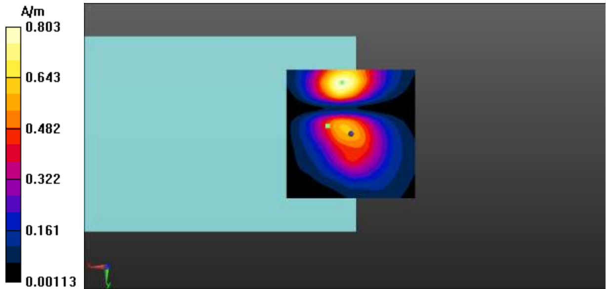
Fig A.22 T-Coil WIFI 5.3G-Y
