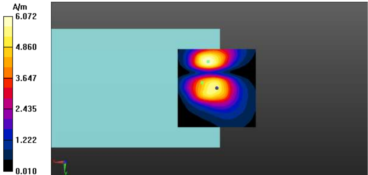
Fig A.17 T-Coil LTE-Band 66-Y
