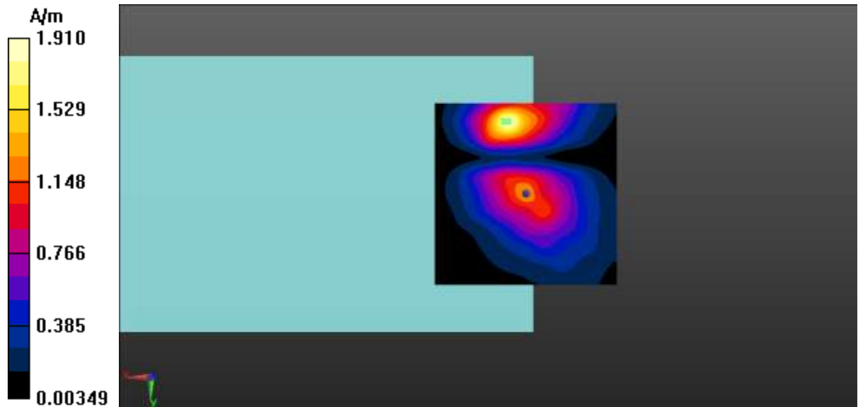
Fig A.37 T-Coil LTE-Band 12-Y
