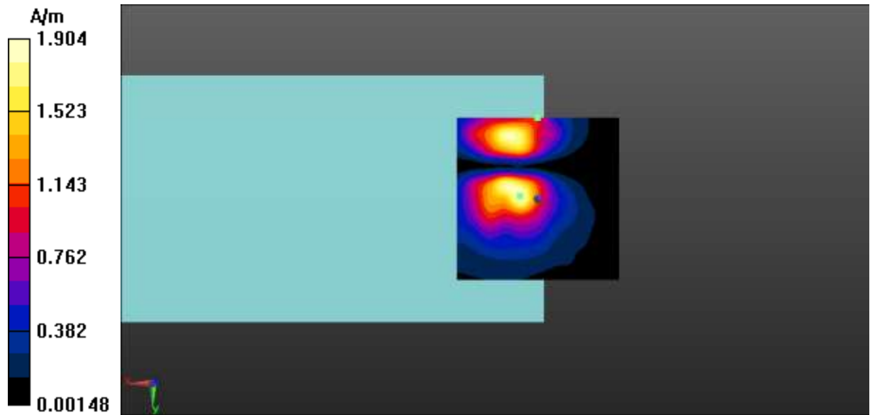
Fig A.47 T-Coil WIFI 5.5G-Y
