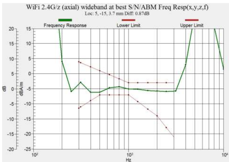
Figure B.44 Frequency Response of WIFI 2.4G (Google Duo)
