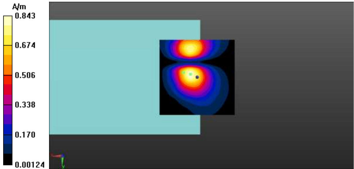
Fig A.23 T-Coil WIFI 5.5G-Y
