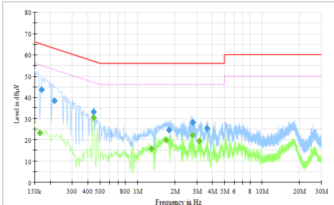
Figure B.11 Conducted Emission
