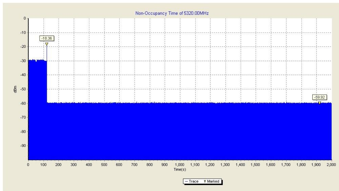
Fig.5 Non-Occupancy Period (HT20 Frequency Band: 5150MHz ~ 5350MHz)
