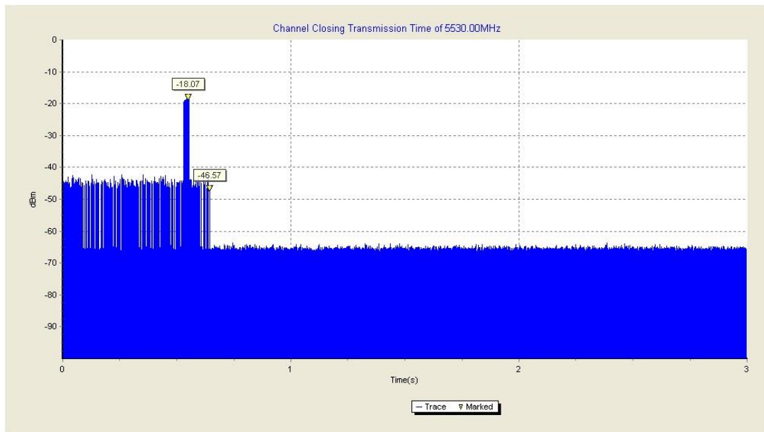
Fig.4 channel closing transmission time (HT80 Frequency Band: 5470MHz ~ 5725MHz)
