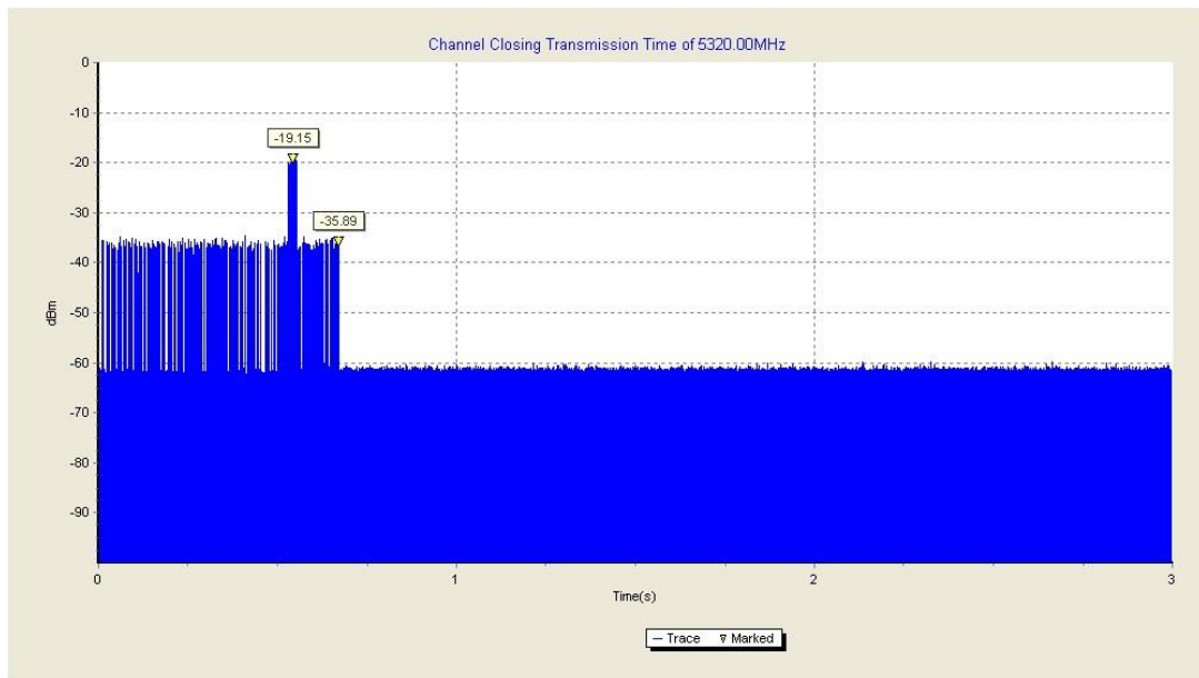
Fig.2 channel closing transmission time (HT20 Frequency Band: 5250MHz ~ 5350MHz)
