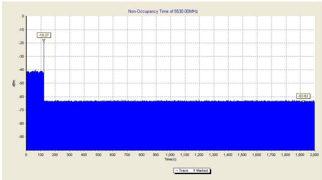
Fig.6 Non-Occupancy Period (HT80 Frequency Band: 5470MHz ~ 5725MHz)
