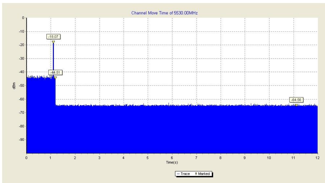
Fig.3 channel move time (HT80 Frequency Band: 5470MHz ~ 5725MHz)
