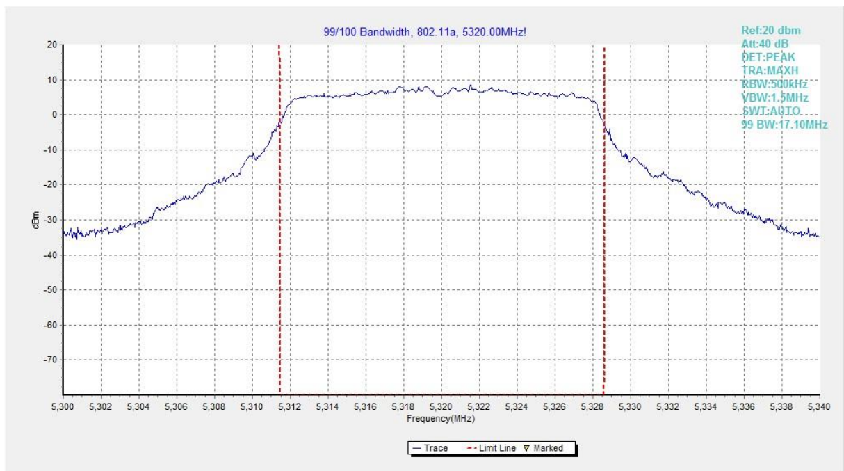
Fig. 44 99% Occupied Bandwidth (802.11a, 5320MHz)
