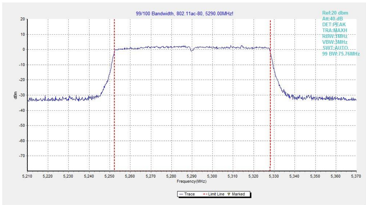
Fig. 65 99% Occupied Bandwidth (802.11ac-VHT80, 5290MHz)
