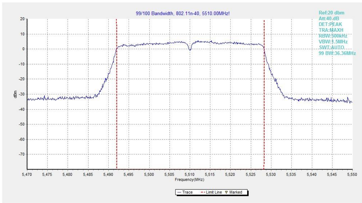
Fig. 61 99% Occupied Bandwidth (802. 11n-HT40, 5510MHz)
