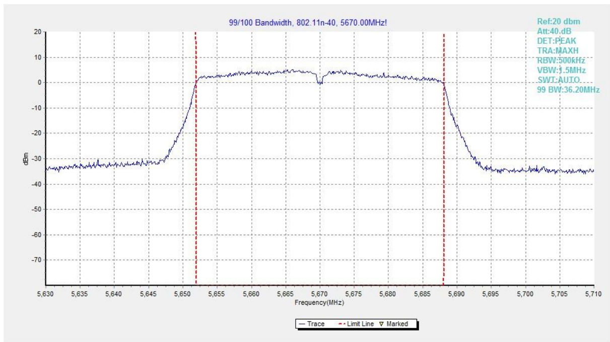
Fig. 63 99% Occupied Bandwidth (802.11n-HT40, 5670MHz)
