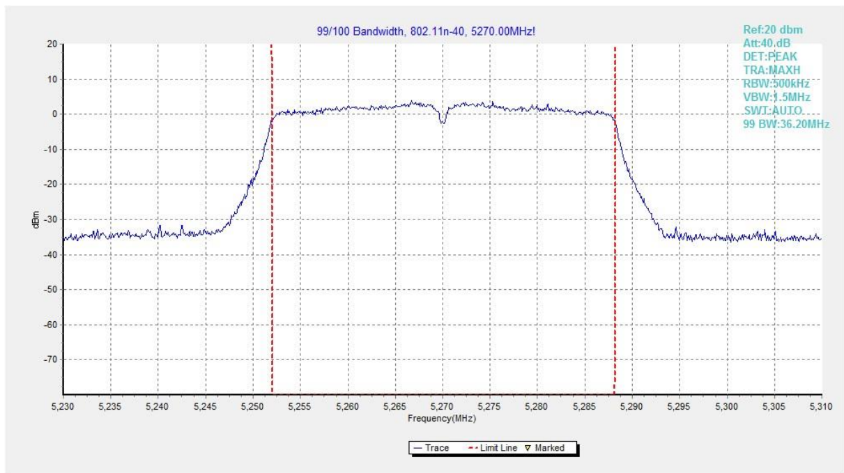
Fig. 59 99% Occupied Bandwidth (802.11n-HT40, 5270MHz)
