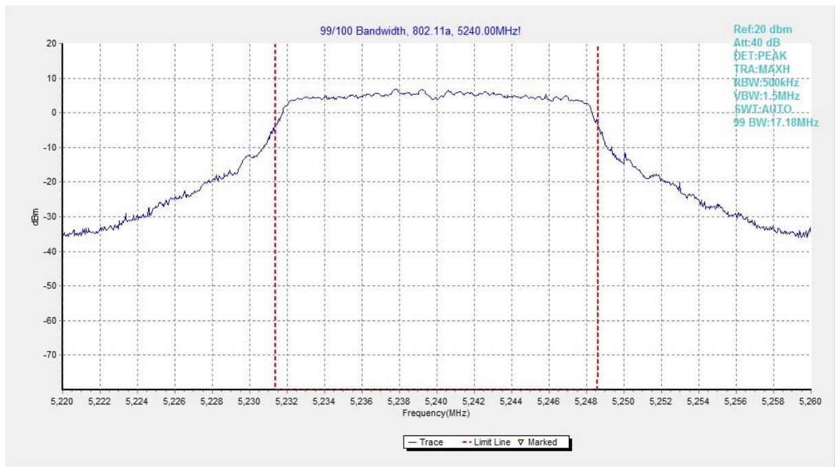
Fig. 41 99% Occupied Bandwidth (802.11a, 5240MHz)
