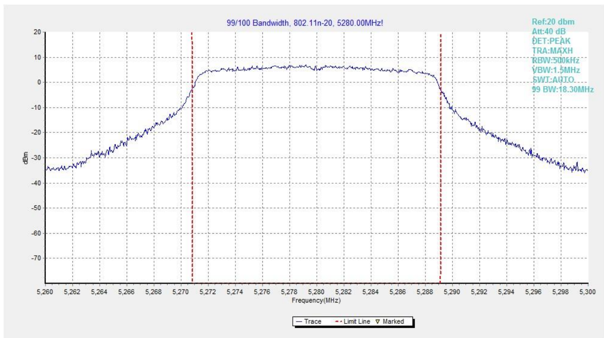
Fig. 52 99% Occupied Bandwidth (802.11n-HT20, 5280MHz)
