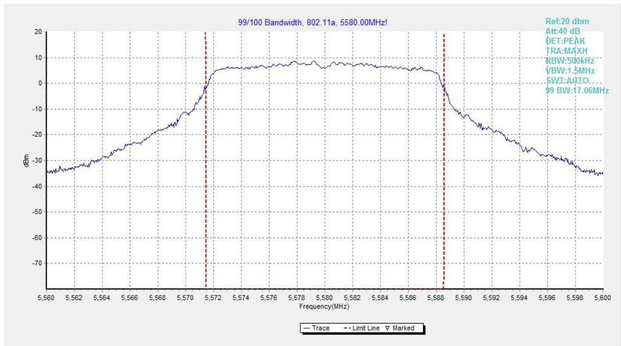
Fig. 46 99% Occupied Bandwidth (802. 11a, 5580MHz)
