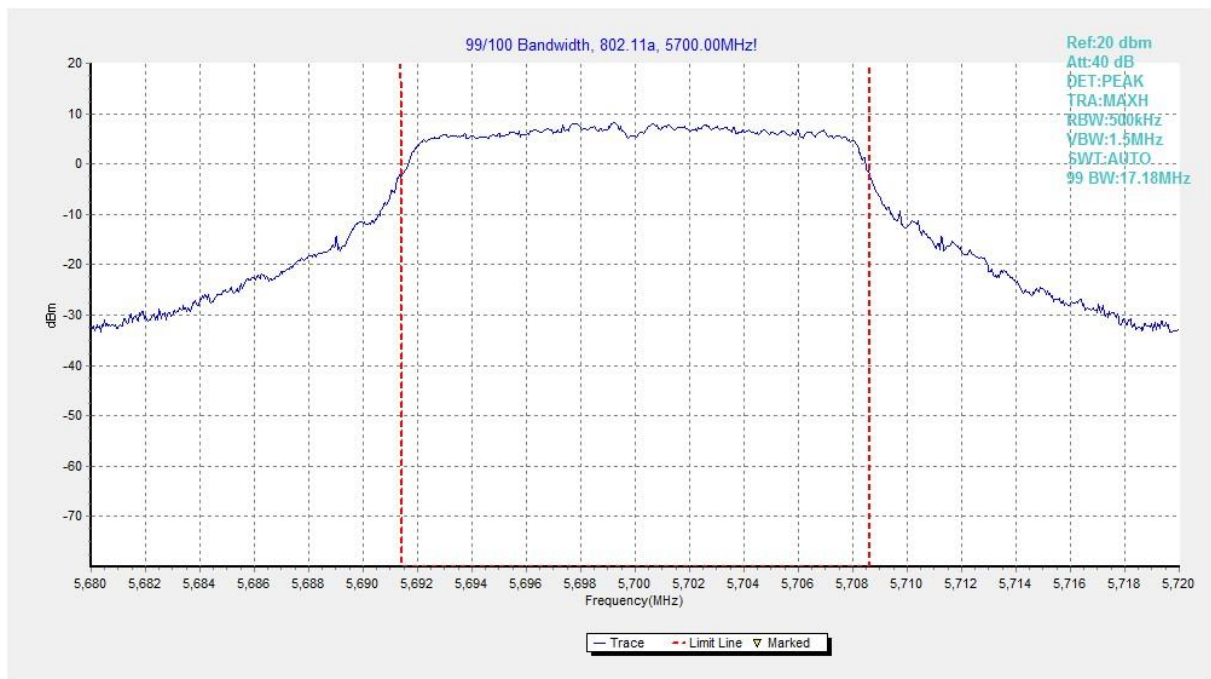
Fig. 47 99% Occupied Bandwidth (802. 11a, 5700MHz)
