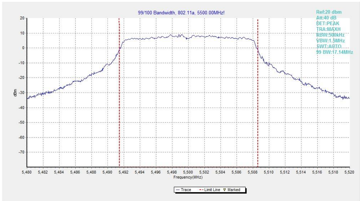
Fig. 45 99% Occupied Bandwidth (802. 11a, 5500MHz)
