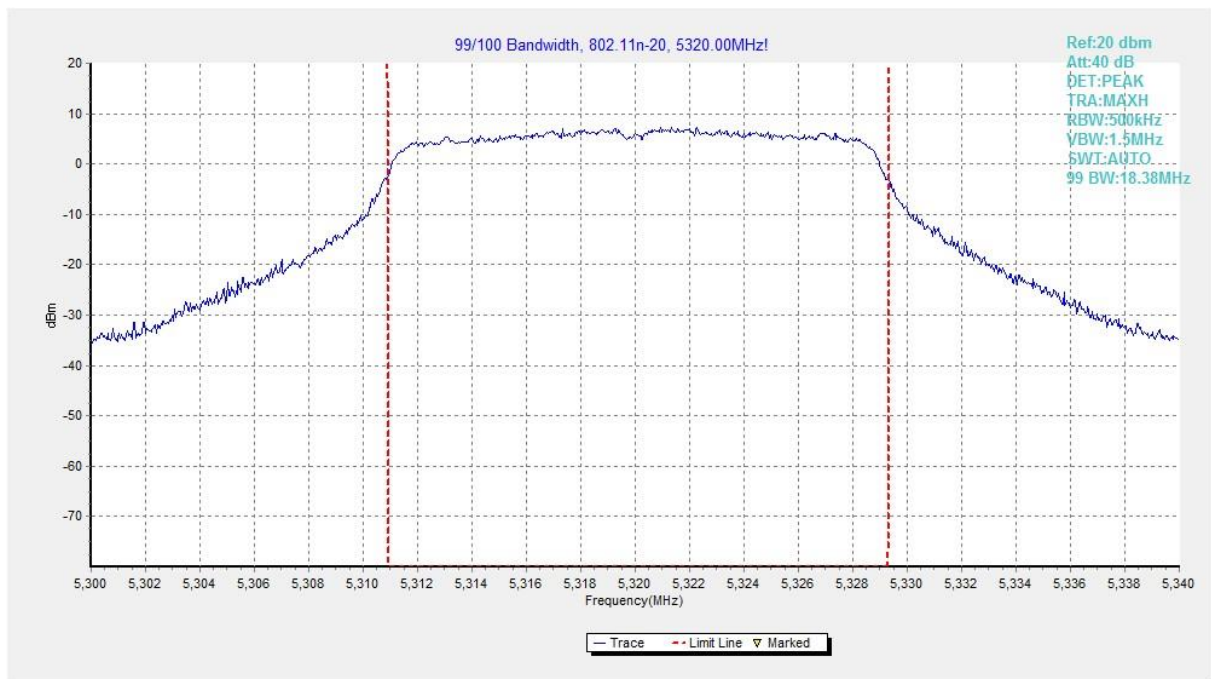
Fig. 53 99% Occupied Bandwidth (802.11n-HT20, 5320MHz)
