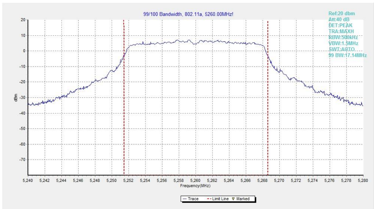
Fig. 42 99% Occupied Bandwidth (802.11a, 5260MHz)
