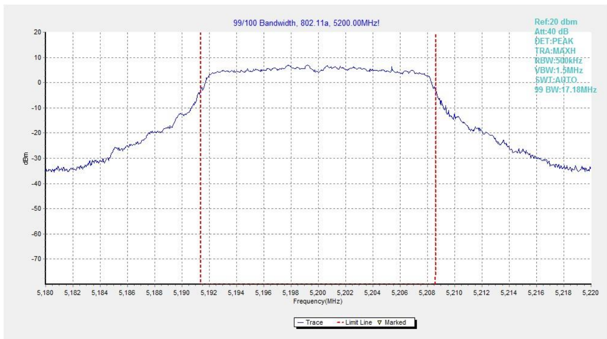
Fig. 40 99% Occupied Bandwidth (802.11a, 5200MHz)
