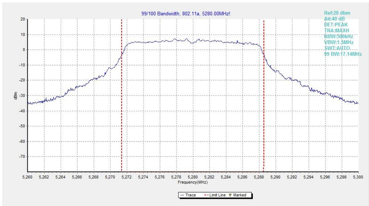
Fig. 43 99% Occupied Bandwidth (802.11a, 5280MHz)
