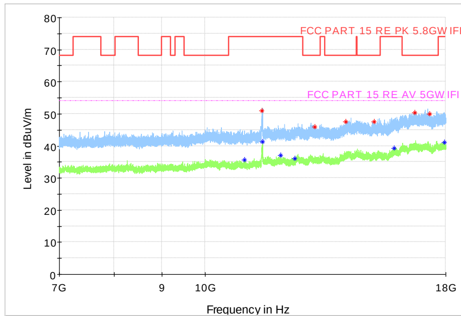
Fig. 155 Transmitter Spurious Emission (802.11n-HT20, CH149 5745MHz, 7 GHz-18 GHz)
