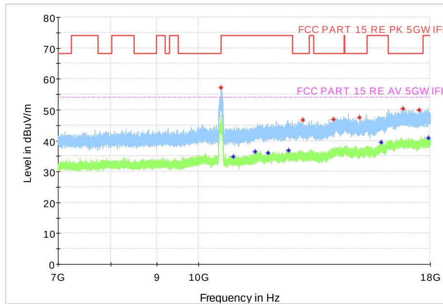
Fig. 194 Transmitter Spurious Emission (802. 11ac-VHT80, CH58 5290MHz, 7 GHz-18 GHz)
