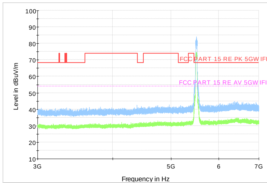
Fig. 175 Transmitter Spurious Emission (802.11n-HT40, CH102 5510MHz, 3 GHz-7 GHz)
