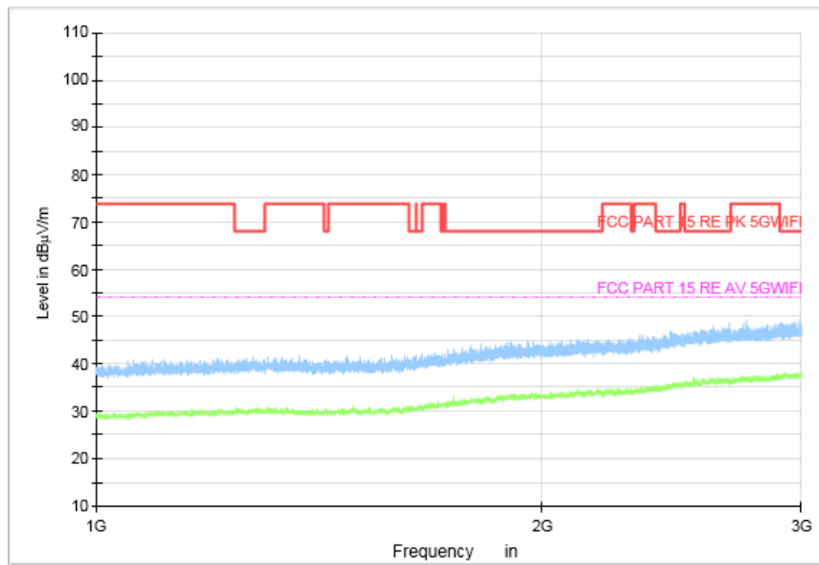
Fig. 180 Transmitter Spurious Emission (802. 11n-HT40, CH134 5670MHz, 1 GHz-3 GHz)
