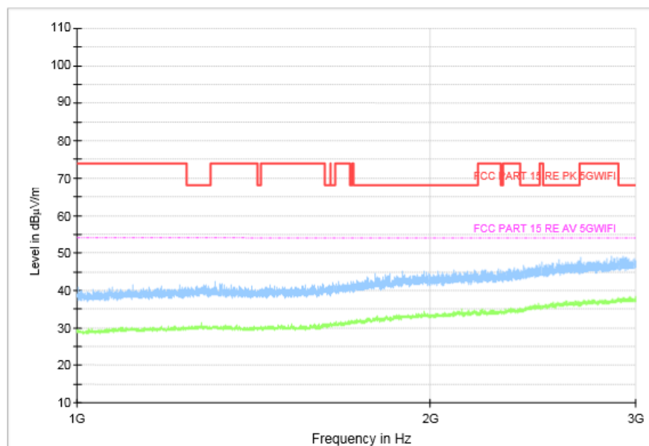
Fig. 195 Transmitter Spurious Emission (802. 11ac-VHT80, CH106 5530MHz, 1 GHz-3 GHz)
