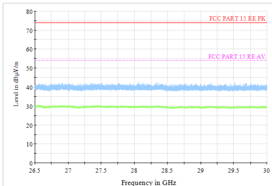
Figure A.5 Radiated Emission (Set.1, Camera Mode , 26.5GHz to 30GHz)
