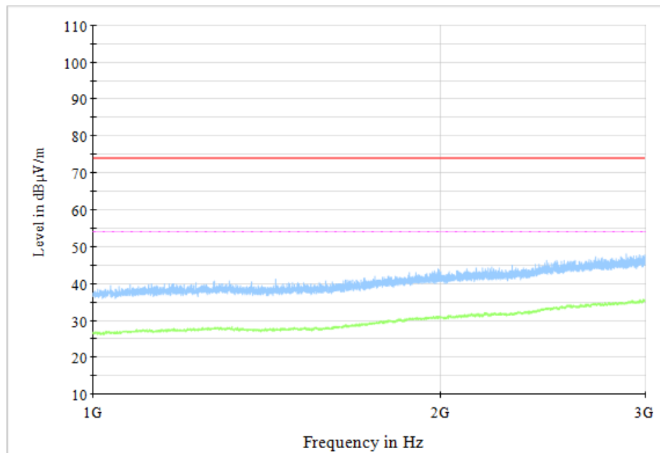
Figure A.7 Radiated Emission (Set.1, Video Player Mode, 1GHz to 3GHz)
