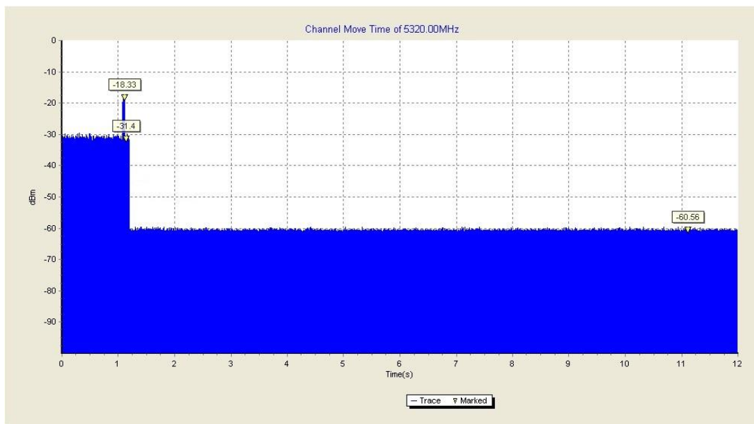
Fig.1 channel move time (HT20 Frequency Band: 5250MHz ~ 5350MHz)
