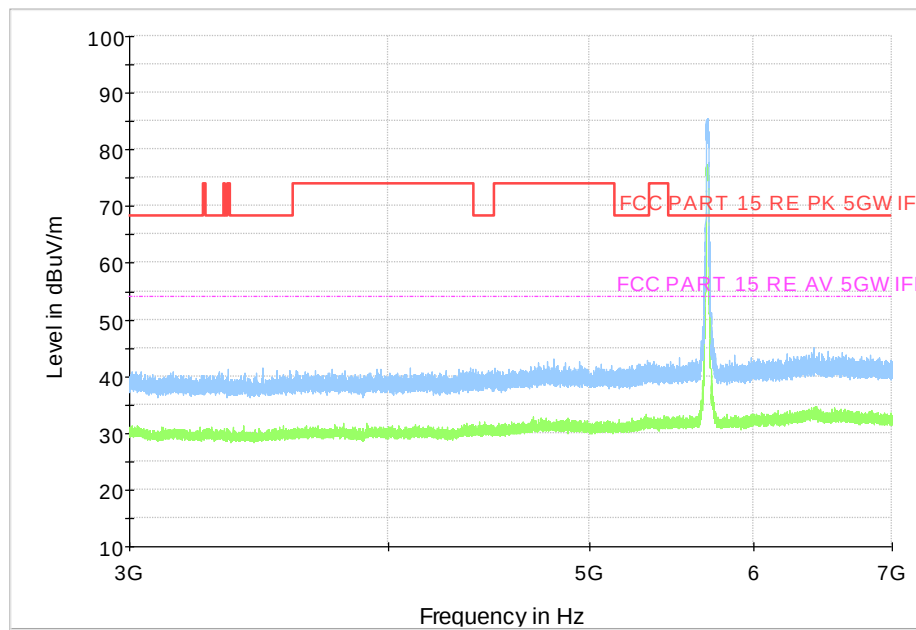
Fig. 115 Transmitter Spurious Emission (802.11a, CH140 5700MHz, 3 GHz-7 GHz)
