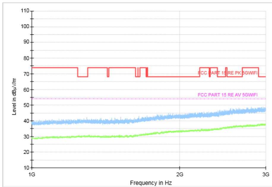
Fig. 114 Transmitter Spurious Emission (802.11a, CH140 5700MHz, 1 GHz-3 GHz)
