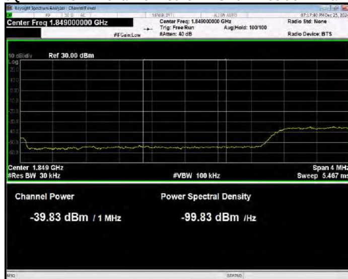
Band2 16QAM BW=5MHz Channel=18625 RB Size=1 Position=#Max Normal
