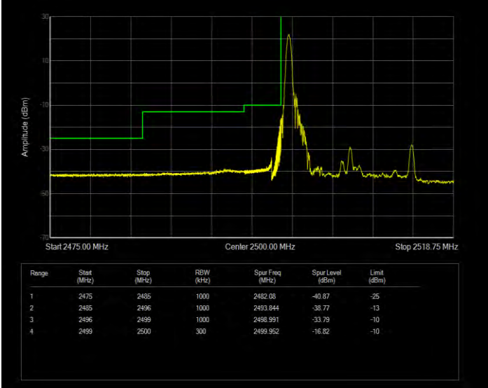
Band7 QPSK BW=15MHz Channel=20825 RB Size=1 Position=#0 Extended
