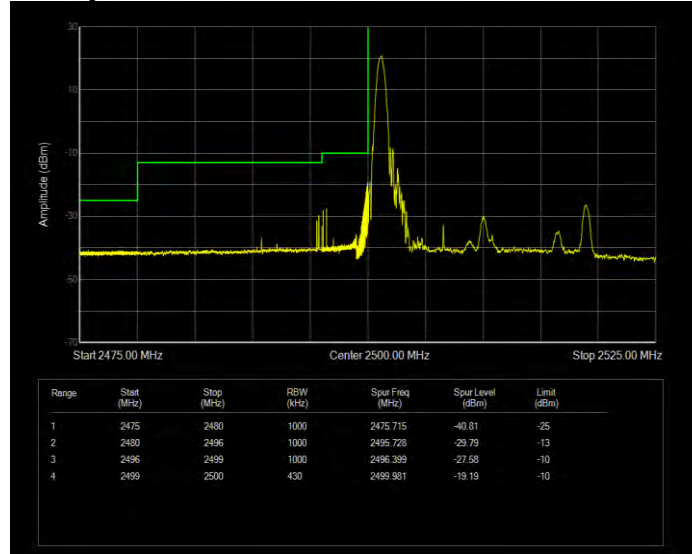
Band7 16QAM BW=20MHz Channel=20850 RB Size=1 Position=#0 Extended
