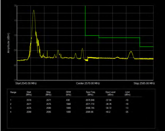
Band7 QPSK BW=20MHz Channel=21350 RB Size=1 Position=#0 Extended
