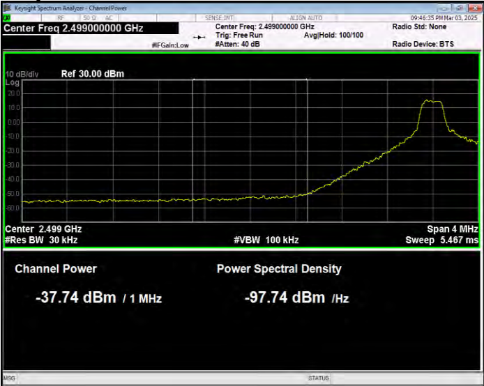
Band7 QPSK BW=10MHz Channel=20800 RB Size=1 Position=#0 Normal
