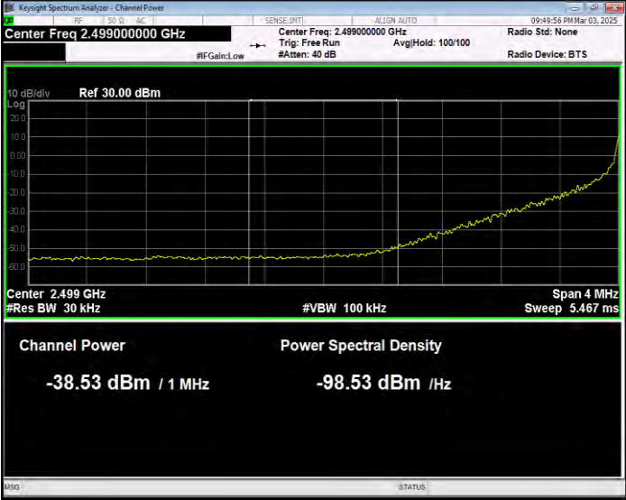
Band7 QPSK BW=20MHz Channel=20850 RB Size=1 Position=#Max Extended
