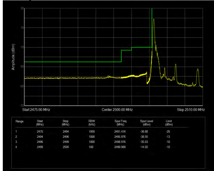
Band7 16QAM BW=5MHz Channel=20775 RB Size=1 Position=#0 Extended
