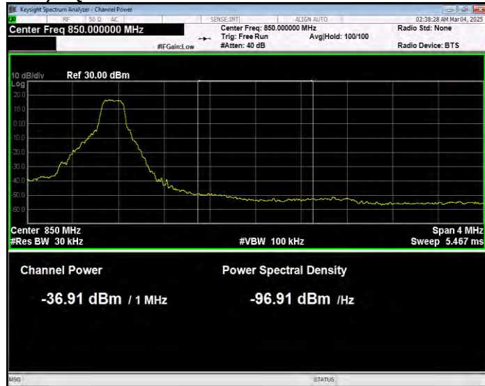
Band26(824-849) 16QAM BW=1.4MHz Channel=27033 RB Size=6 Position=#0 Extended
