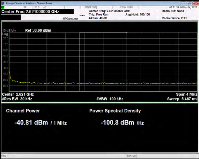
Band38 16QAM BW=20MHz Channel=38150 RB Size=1 Position=#Max Extended
