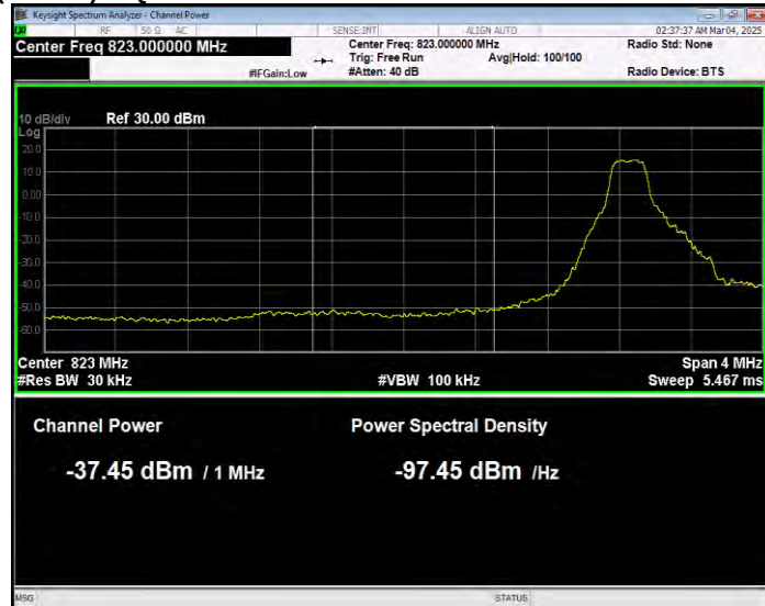
Band26(824-849) 16QAM BW=1.4MHz Channel=26797 RB Size=1 Position=#0 Normal
