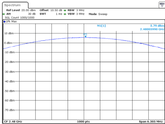
3DH1_High 5.79dBm
