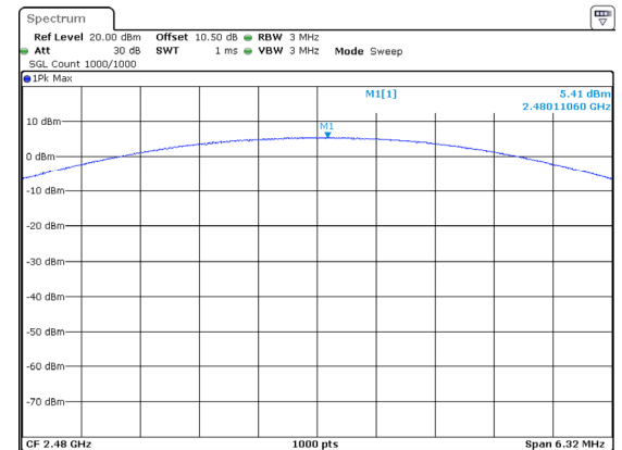
2DH1_High 5.41dBm
