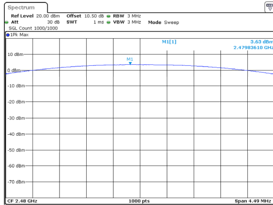
DH1_High 3.63dBm
