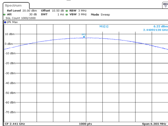
3DH1_Middle 6.22dBm
