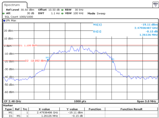
3DH1_High 1.261MHz
