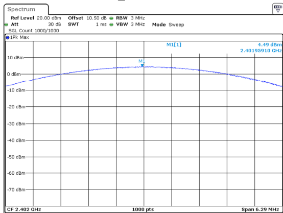
3DH1_Low 4.49dBm
