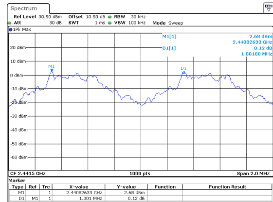
DH1_Middle 1.001MHz
