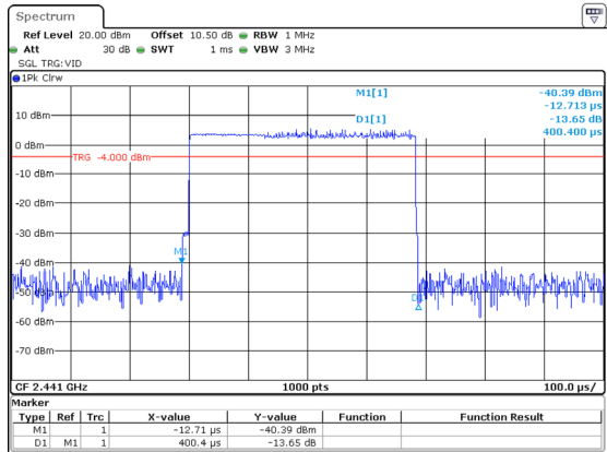
3DH1_Hop_2441 0.400ms
