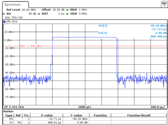
DH1_Hop_2441 0.408ms
