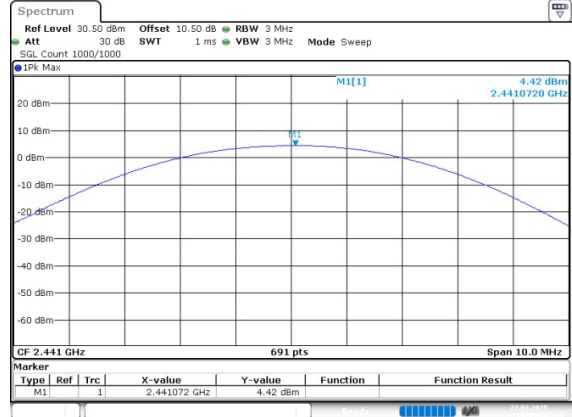
DH1_Middle 4.42dBm
