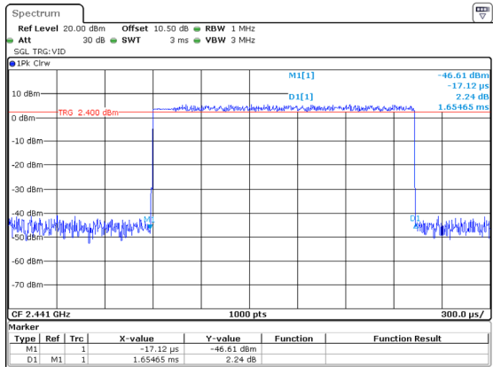
3DH3_Hop_2441 1.655ms
