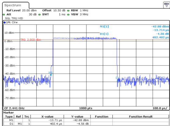
2DH1_Hop_2441 0.402ms
