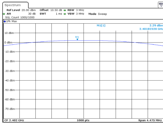
DH1_Low 2.29dBm
