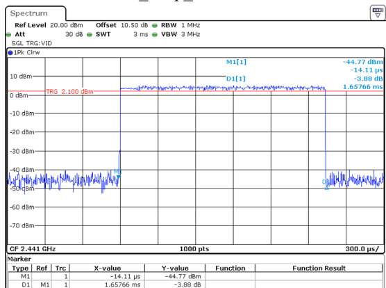
2DH3_Hop_2441 1.658ms
