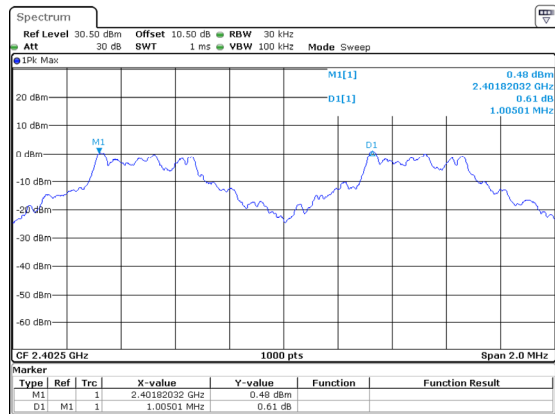
DH1_Low 1.005MHz
