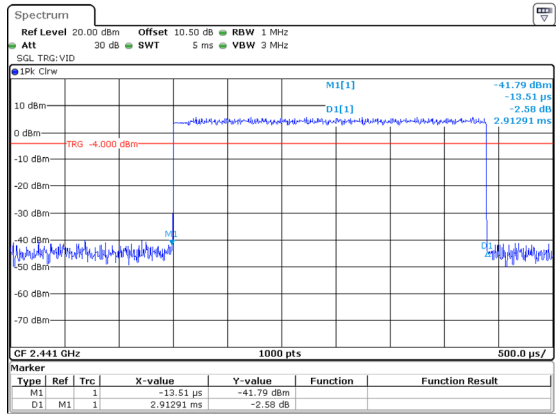
3DH5_Hop_2441 2.913ms
