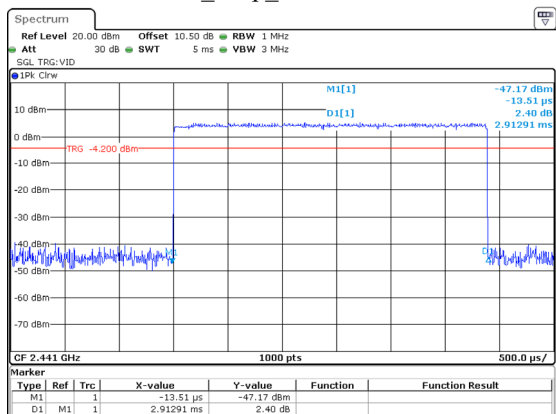
2DH5_Hop_2441 2.913ms
