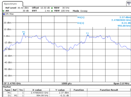
DH1_High 0.995MHz
