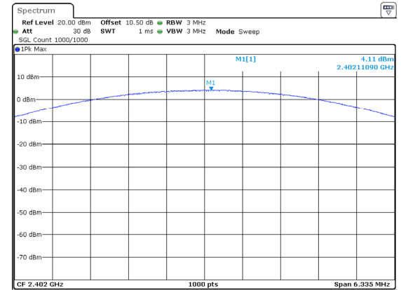
2DH1_Low 4.11dBm
