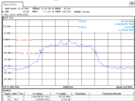
3DH1_Low 1.258MHz
