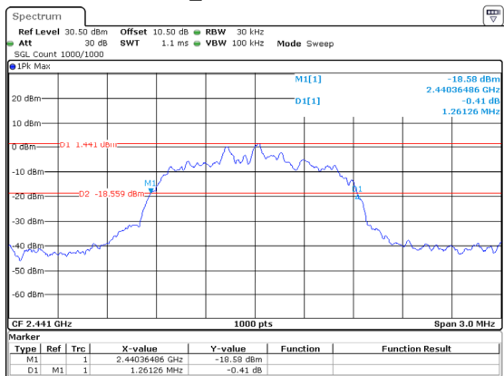
3DH1_Middle 1.261MHz
