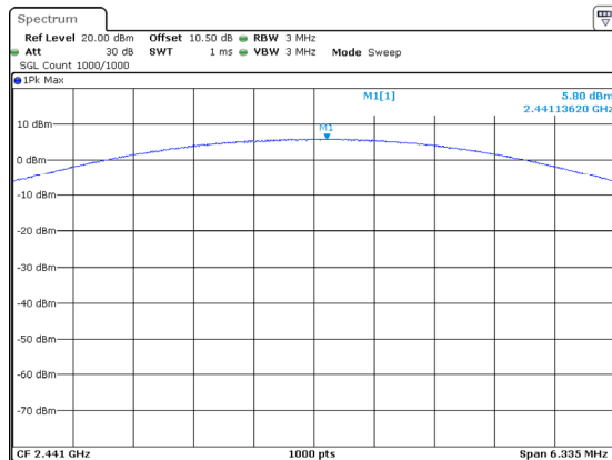
2DH1_Middle 5.80dBm
