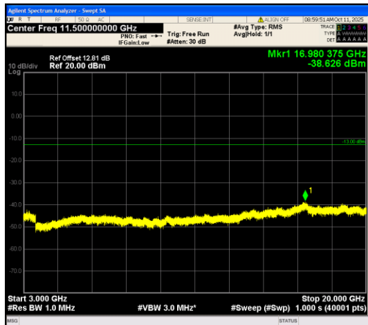
Band25_1.4MHz_QPSK_26047_6RB#0_3000~2 0000_3000~20000
