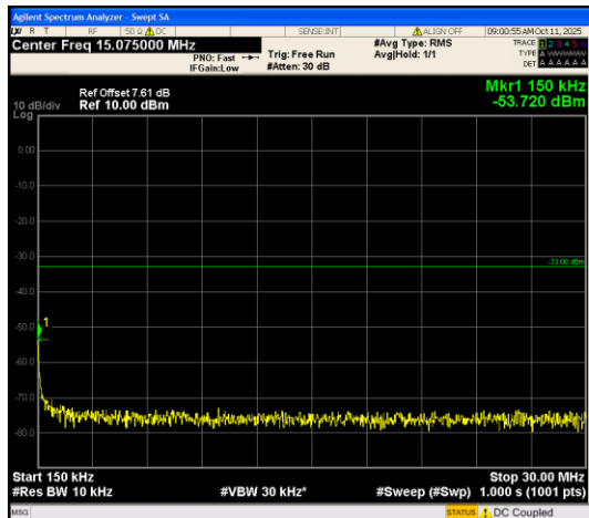
Band25_1.4MHz_QPSK_26365_6RB#0_0.15~3 0_0.15~30
