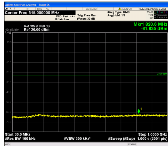
Band25_1.4MHz_QPSK_26365_6RB#0_30~100 0_30~1000
