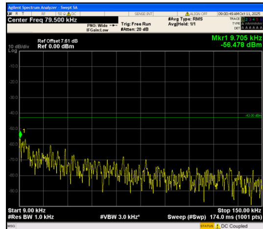
Band25_1.4MHz_QPSK_26365_6RB#0_0.009~ 0.15_0.009~0.15
