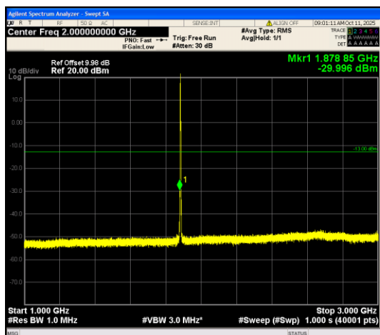
Band25_1.4MHz_QPSK_26365_6RB#0_1000~3 000_1000~3000
