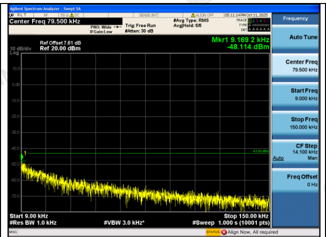
GPRS1900-512-0-0.009~0.15MHz-PASS
