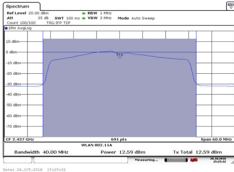
Fig.65 Maximum Average Output Power (802.11n-40MHz, Ch 6,MCS1)
