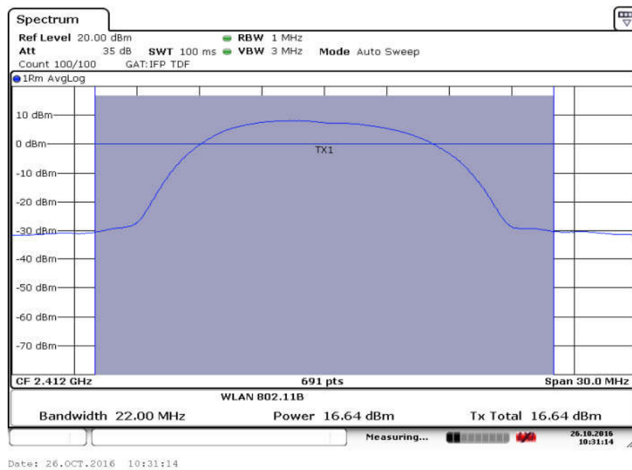
Fig.7 Maximum Average Output Power (802.11b, Ch 1,5.5Mbps)
