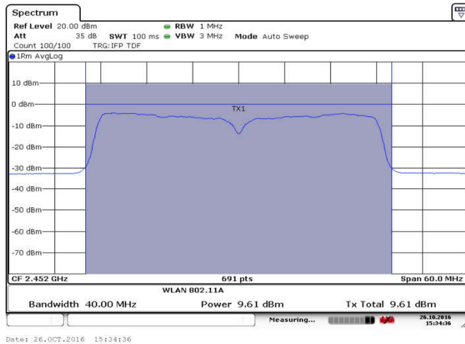
Fig.81 Maximum Average Output Power (802.11n-40MHz, Ch 9,MCS6)
