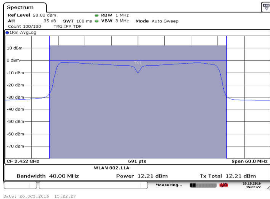
Fig.63 Maximum Average Output Power (802.11n-40MHz, Ch 9,MCS0)
