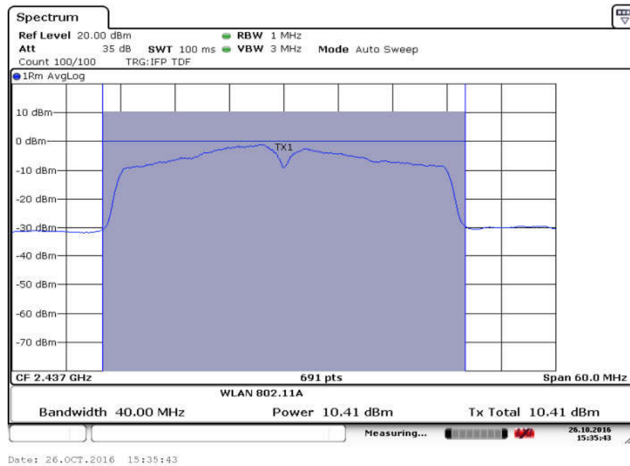
Fig.83 Maximum Average Output Power (802.11n-40MHz, Ch 6,MCS7)
