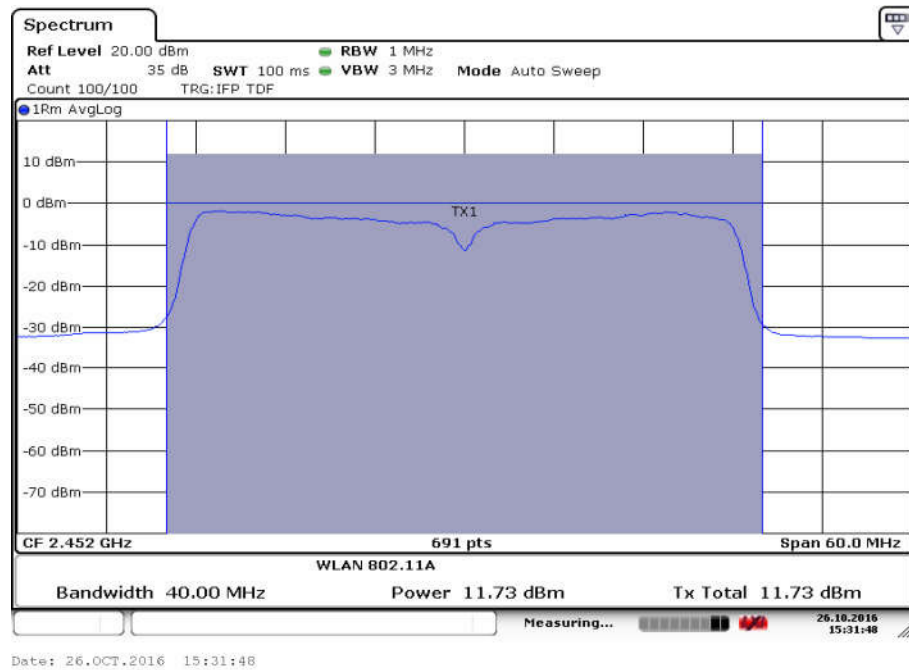
Fig.75 Maximum Average Output Power (802.11n-40MHz, Ch 9,MCS4)
