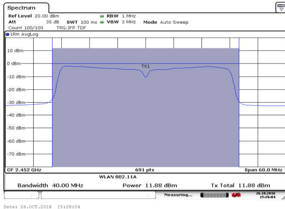
Fig.66 Maximum Average Output Power (802.11n-40MHz, Ch 9,MCS1)
