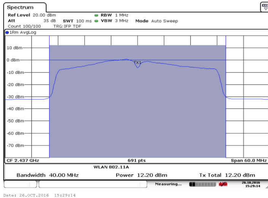
Fig.71 Maximum Average Output Power (802.11n-40MHz, Ch 6,MCS3)
