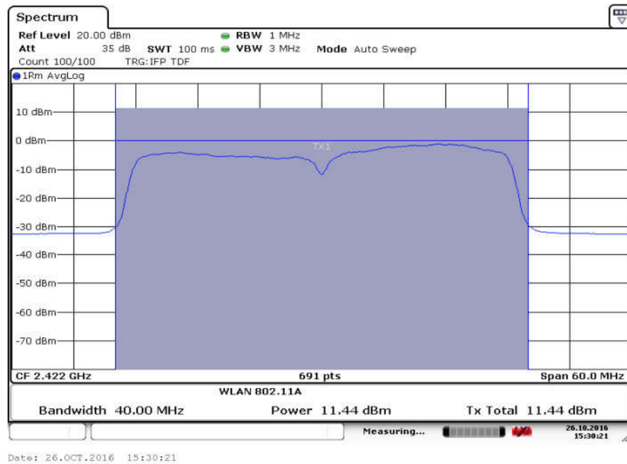
Fig.73 Maximum Average Output Power (802.11n-40MHz, Ch 3,MCS4)
