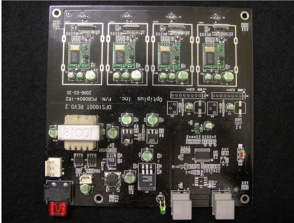
<Photograph 3: Front View- FM Transmitter, Model DFS1000T – Main board>
