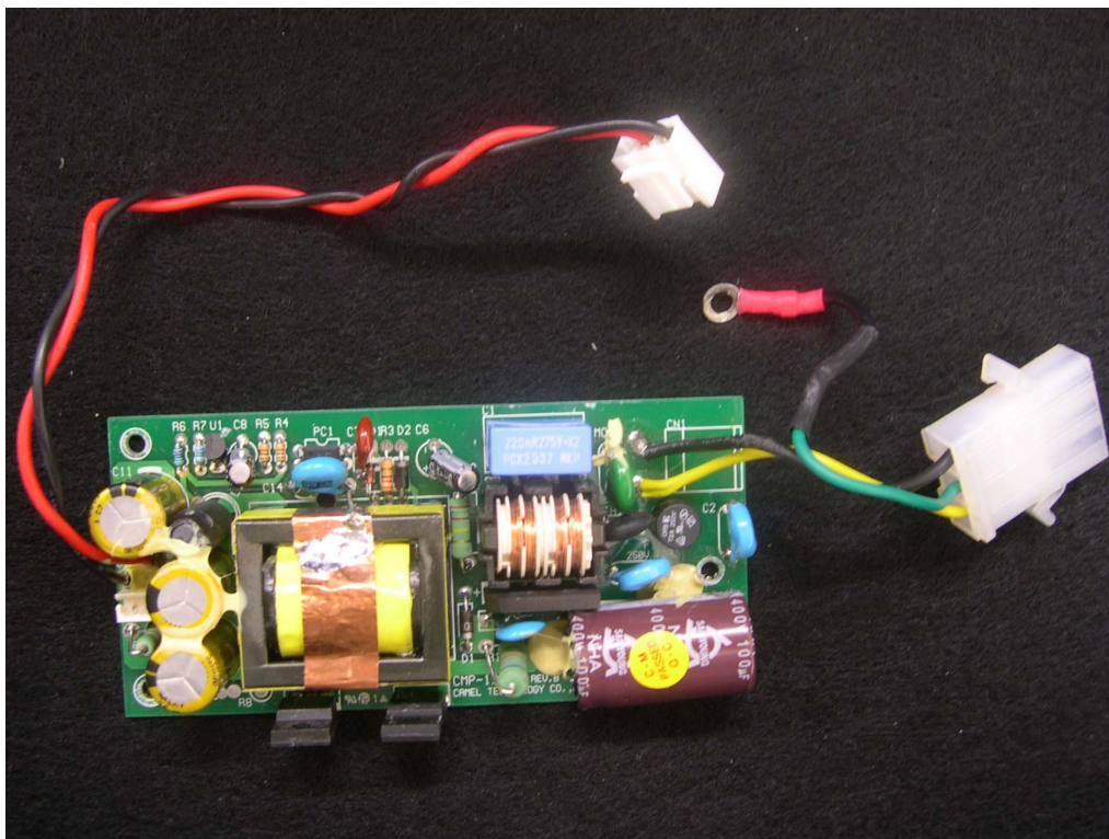
<Photograph 11: Front View- Audio Converter, Model DFS1000R – SMPS board>
