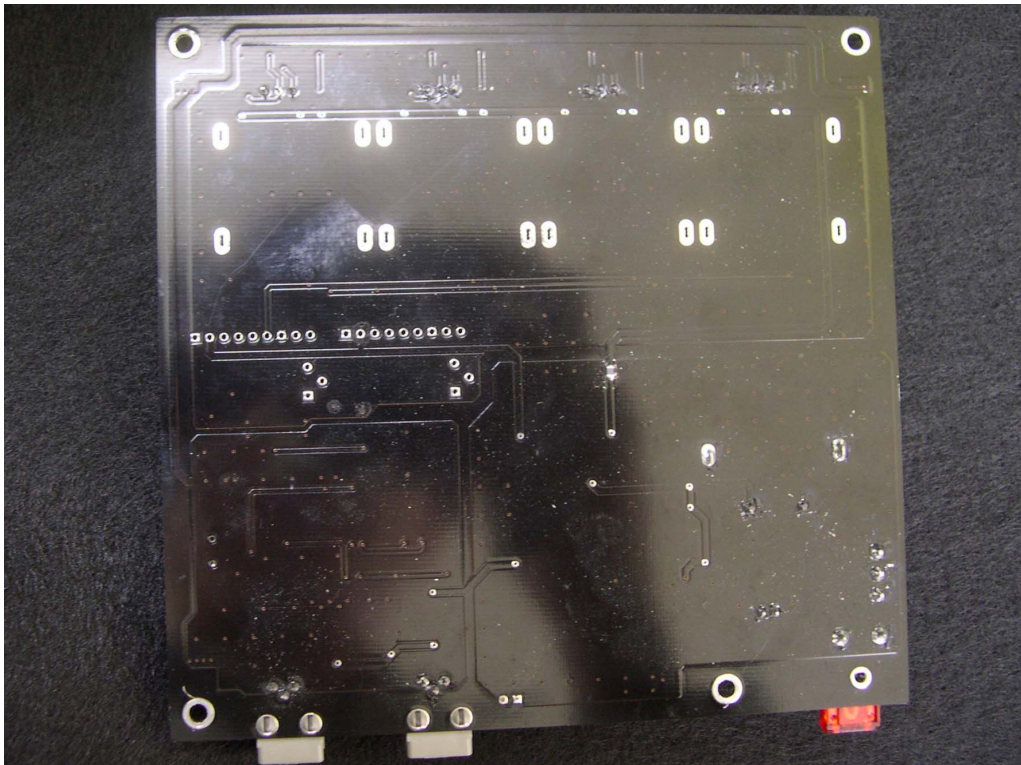
<Photograph 4: Rear View- FM Transmitter, Model DFS1000T – Main board>
