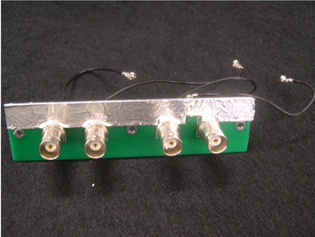
<Photograph 7: Front View- FM Transmitter, Model DFS1000T – Antenna board>
