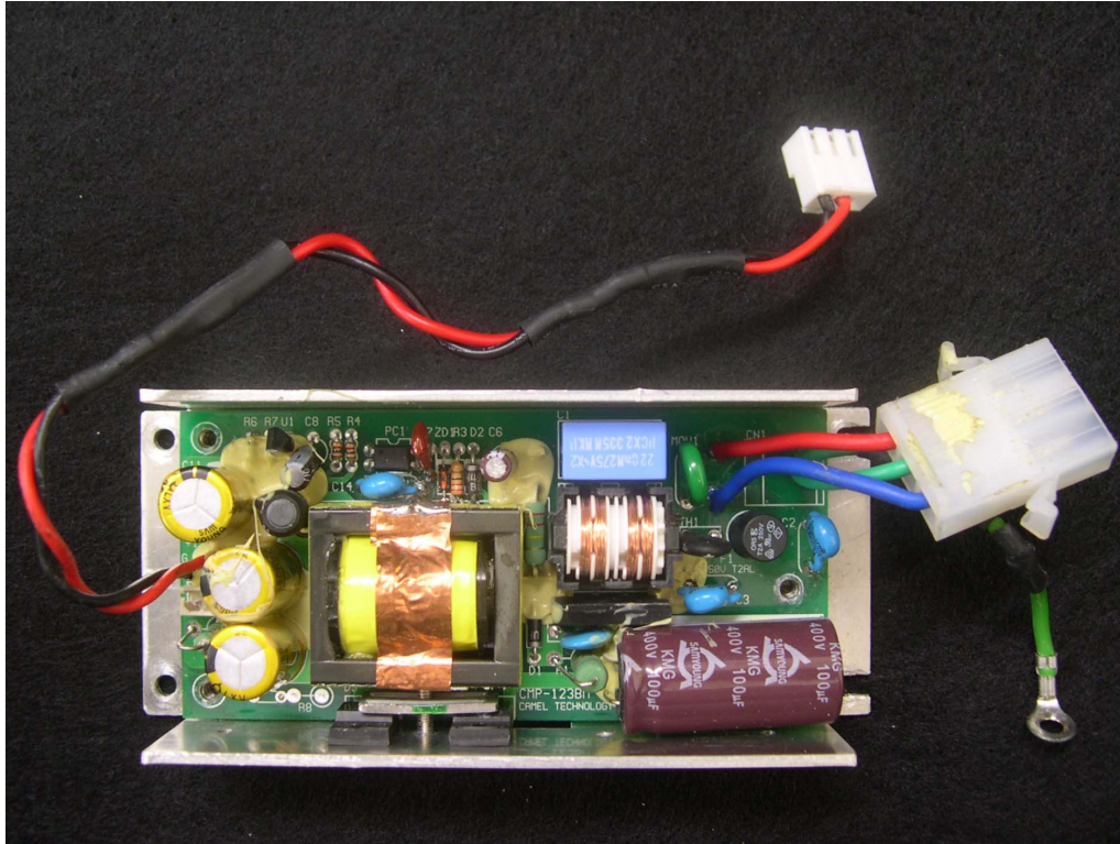
<Photograph 5: Front View- FM Transmitter, Model DFS1000T – SMPS board>
