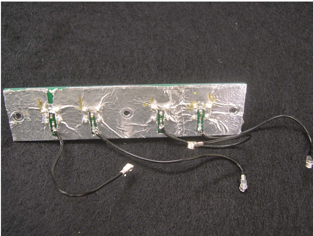
<Photograph 8: Rear View- FM Transmitter, Model DFS1000T – Antenna board>
