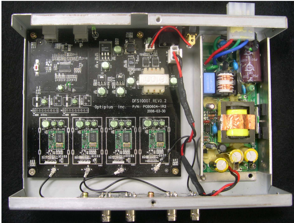
<Photograph 1: Cover removed – FM Transmitter, Model DFS1000T>
