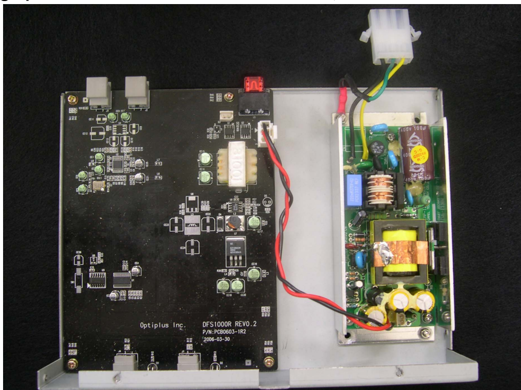
<Photograph 2: Cover removed – Audio Converter, Model DFS1000R>
