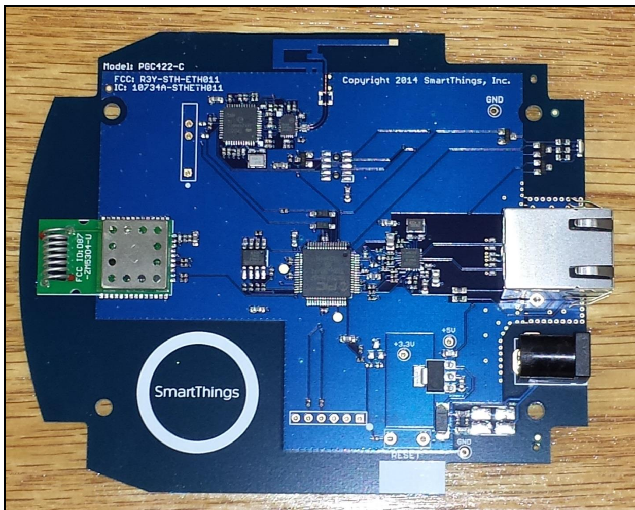
Photograph 11: PCB Top
