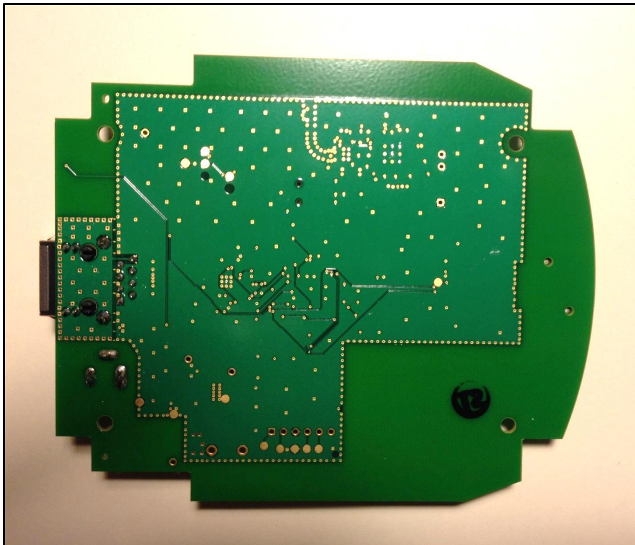
Photograph 12: PCB Bottom
