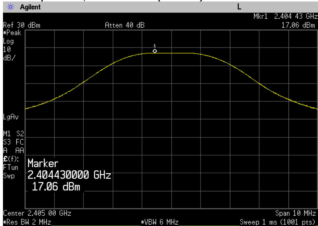
Peak Output Power, Lowest Channel (2405 MHz)
