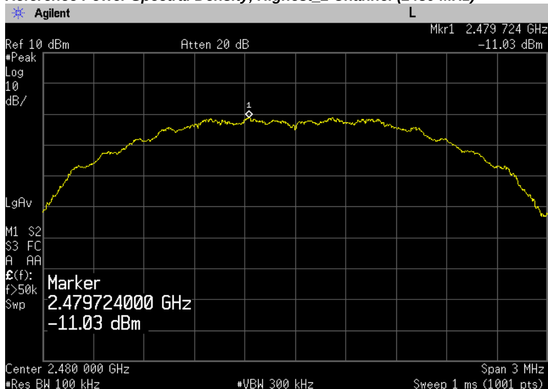
Reference Power Spectral Density, Highest_2 Channel (2480 MHz)
