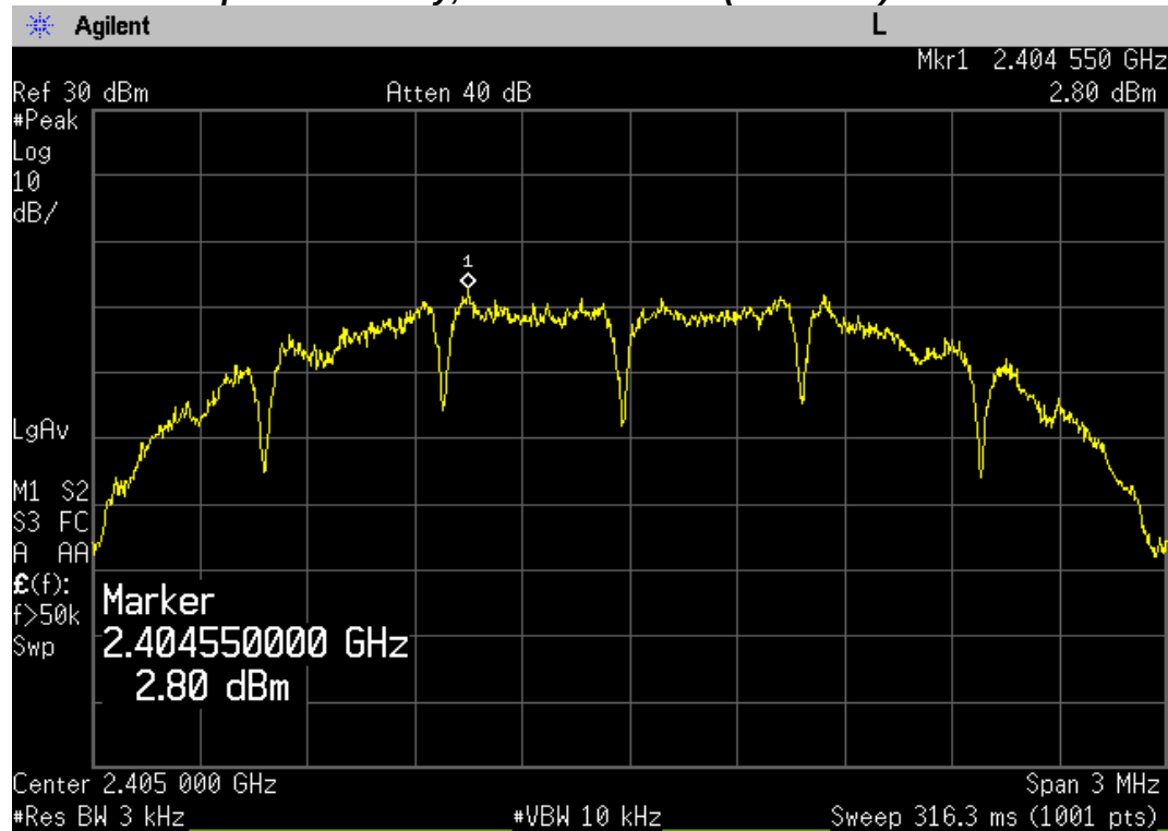
Peak Power Spectral Density, Lowest Channel (2405 MHz)
