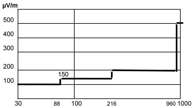
Fig. 3. Limits at 3 meters
