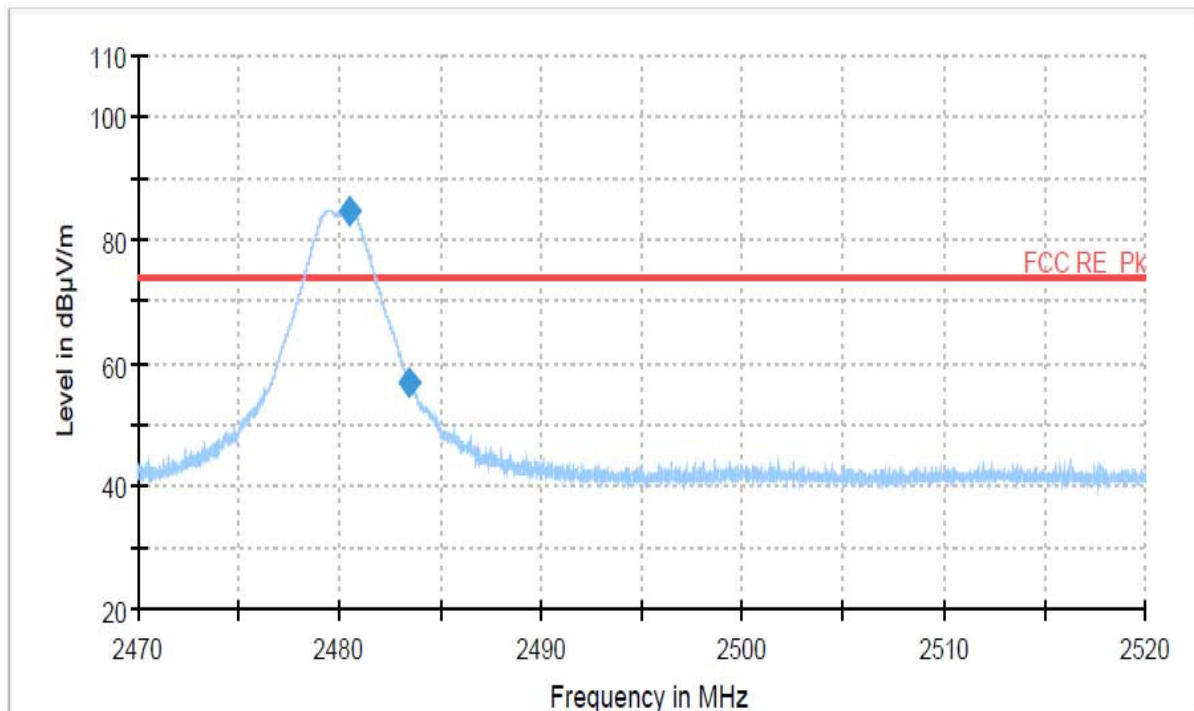
Highest_2 Channel (2480 MHz : Peak)
