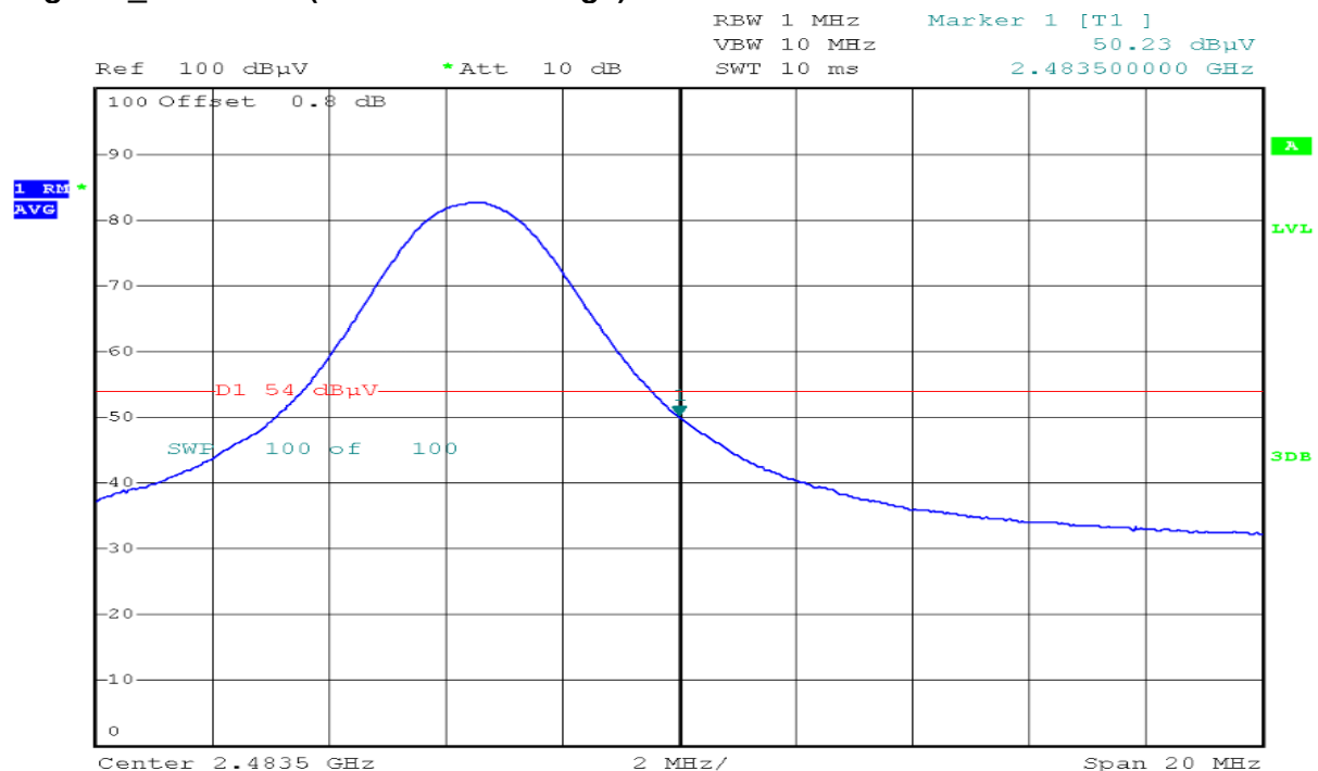
Highest_2 Channel (2480 MHz : Average)
