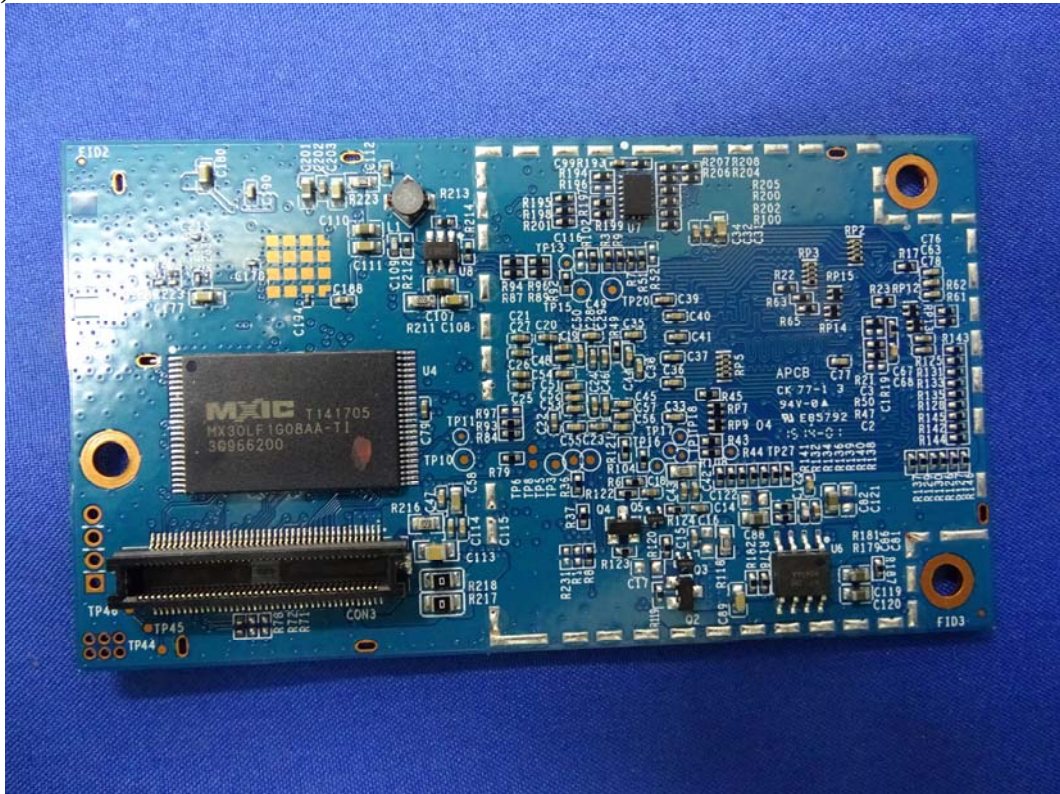
(26) EUT Photo -Antenna
