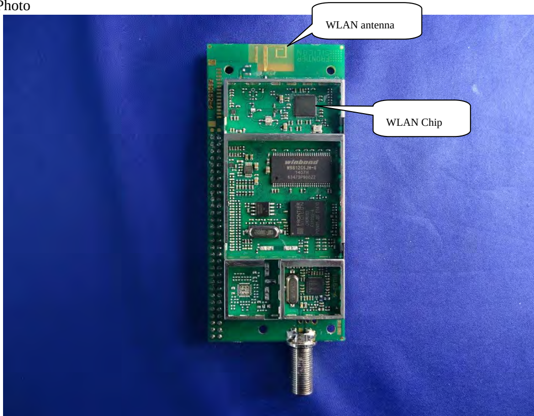
(36) EUT Photo(Wlan moudle & Wlan antenna)
