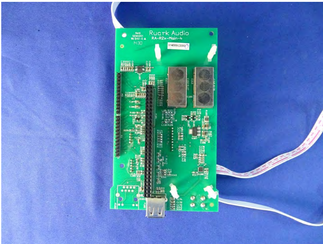
(32) EUT Photo
