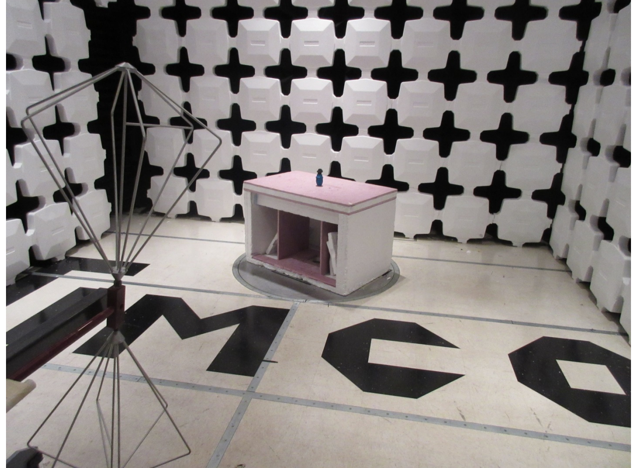
Radiated Emissions Below 1 GHz Setup
