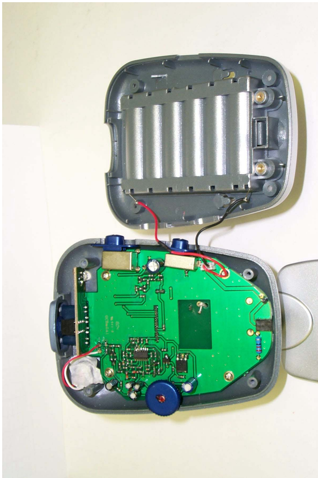
Figure 7.3 Open view
