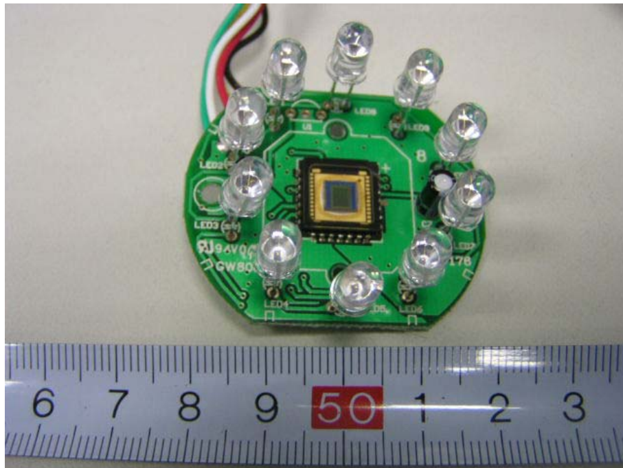
EUT- LED PCB Front View (2)
