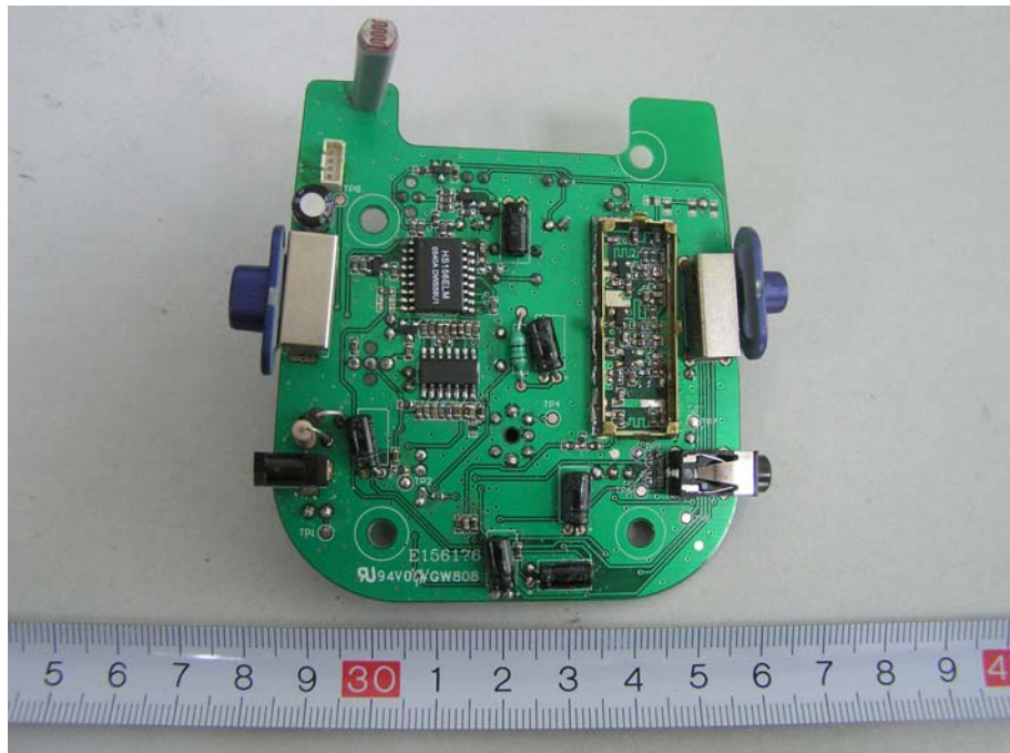
EUT- Main PCB Back View (2)
