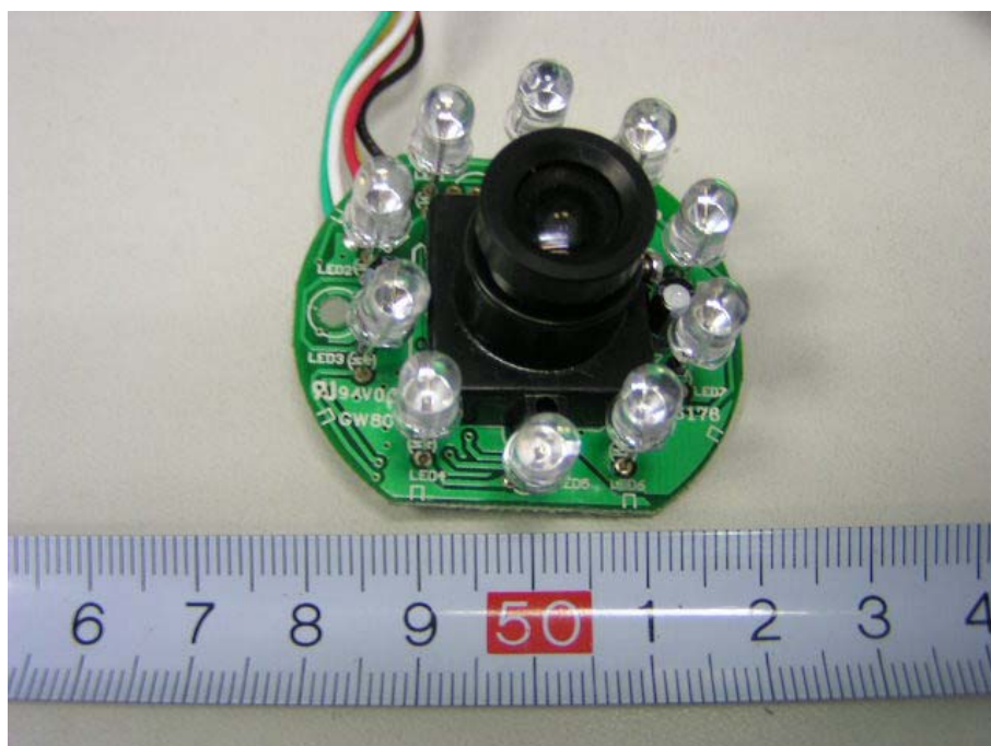
EUT- LED PCB Front View (1)
