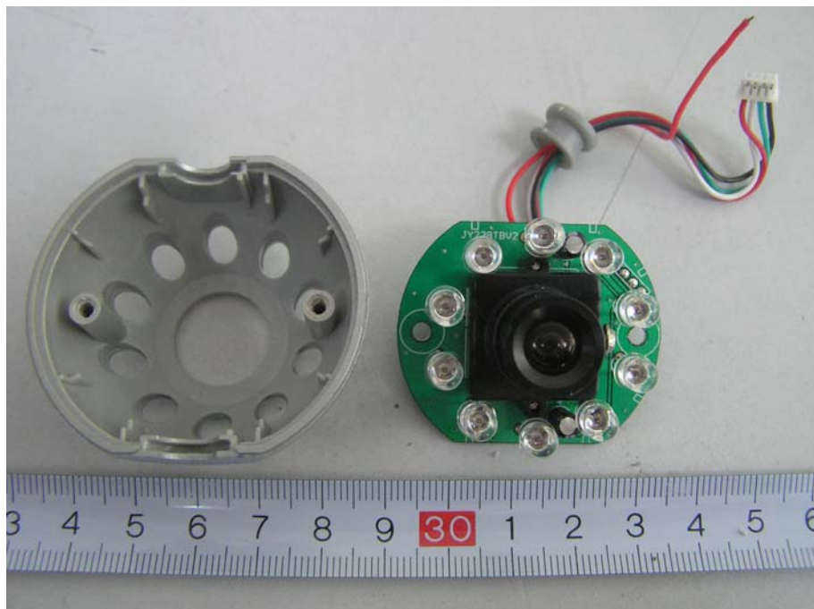
EUT-Inside View (4)
