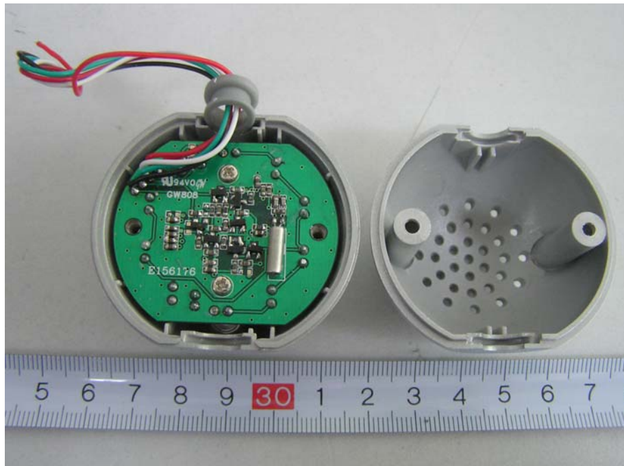
EUT-Inside View (3)
