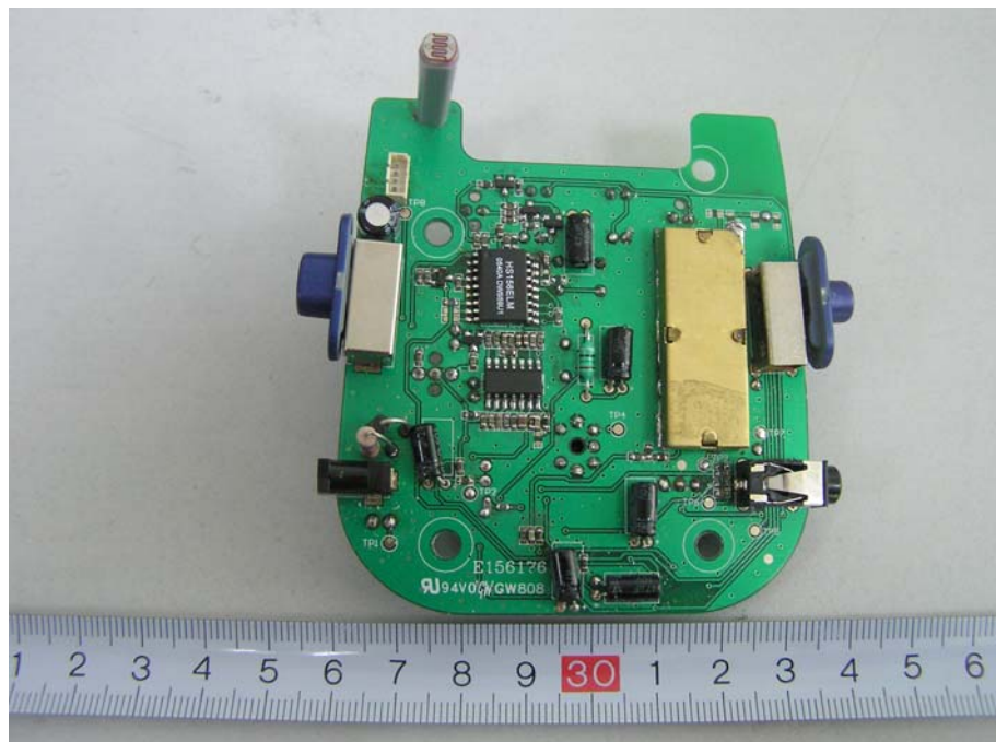
EUT- Main PCB Back View (1)
