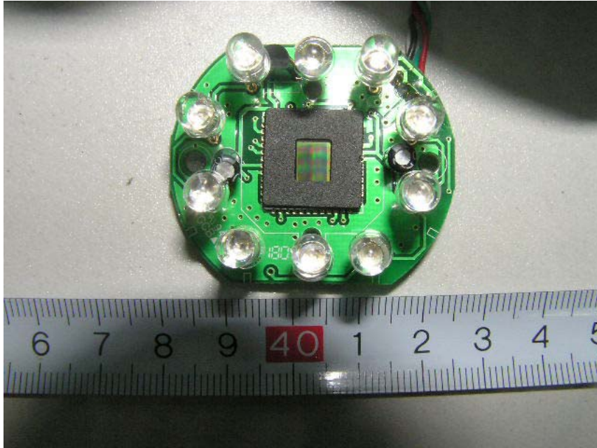
LED PCB Front View
