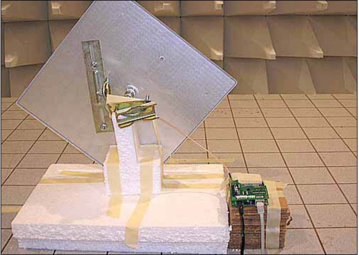
15.247(d) 23dBi Antenna Back Close-up
