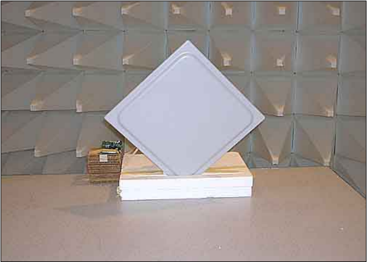
Radiated Emissions - Front View Receiver Panel Antenna 15.109
