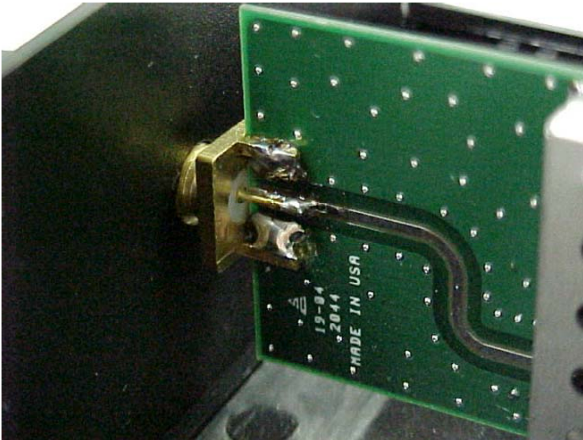
Photo Two – Internal Close Up of Antenna Connection
