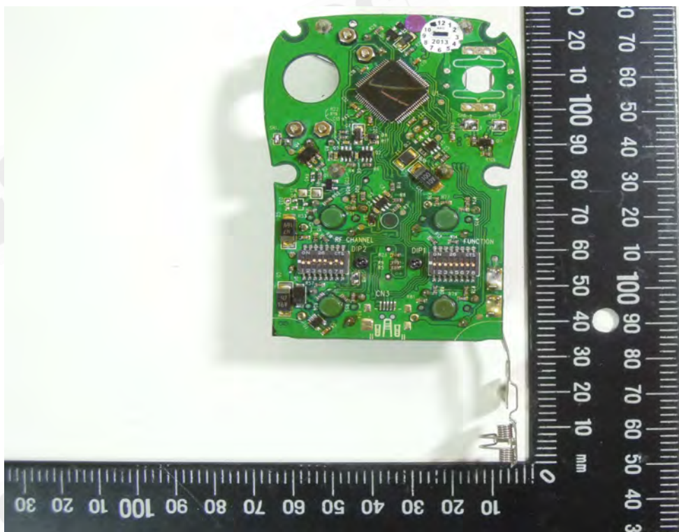
Internal View of EUT-3 (FLEX 4ES/4EX)
