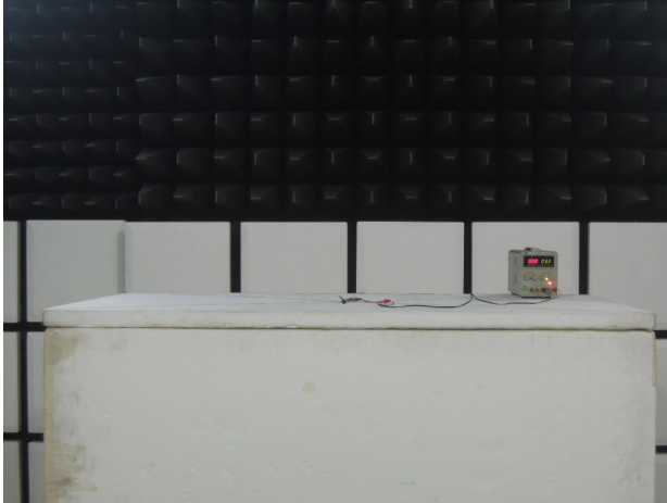
SRD_Radiated_966 (2)_Setup
