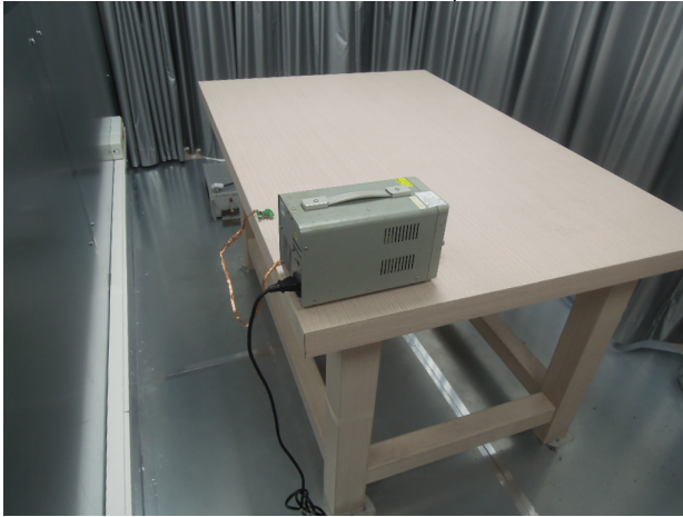
SRD_Conduction_Setup
