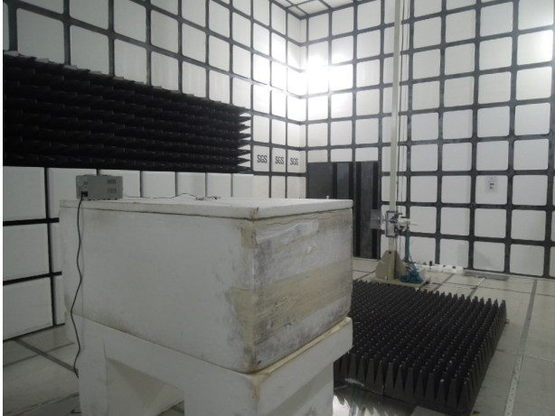
SRD_Radiated_966 (2)_Setup
