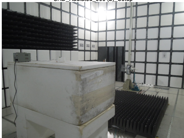
SRD_Radiated_966 (2)_Setup
