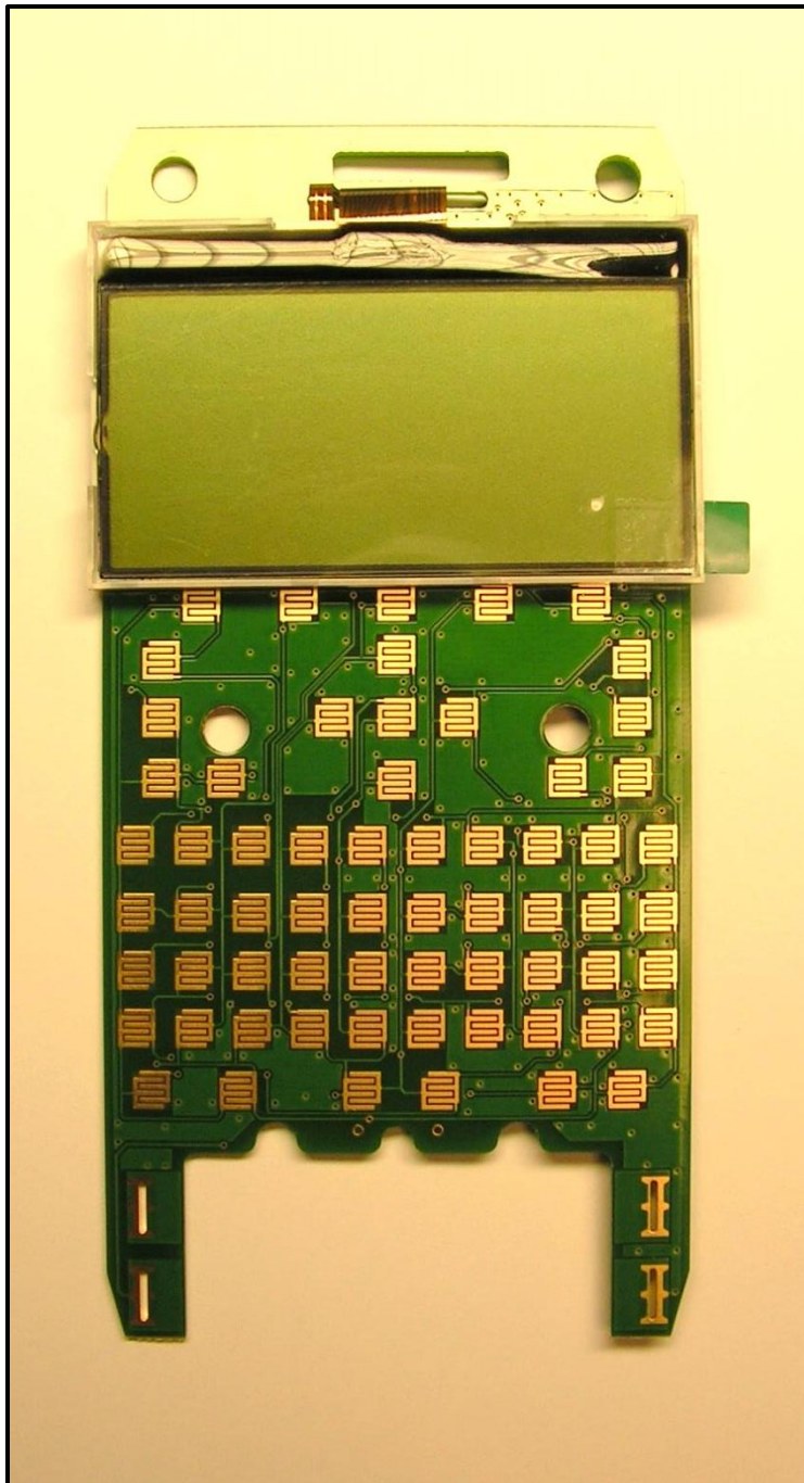
Photograph 7: Front with LCD
