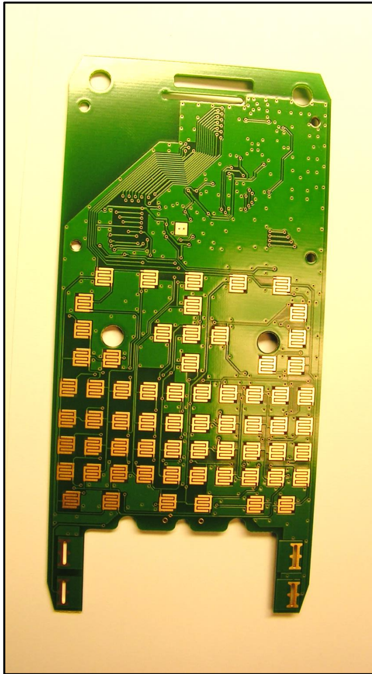
Photograph 16: Front
