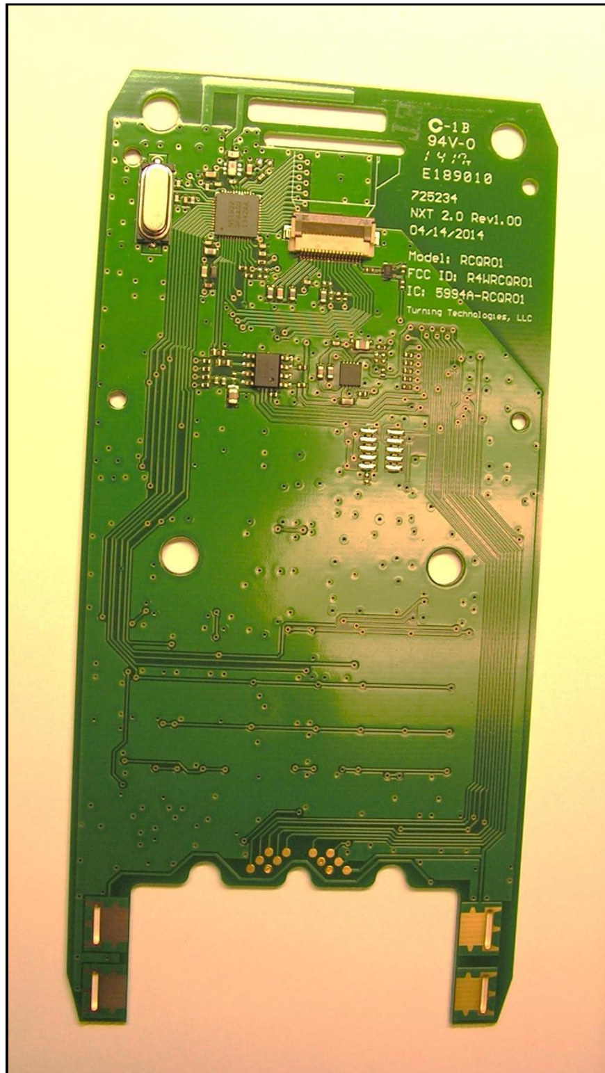
Photograph 18: Back
