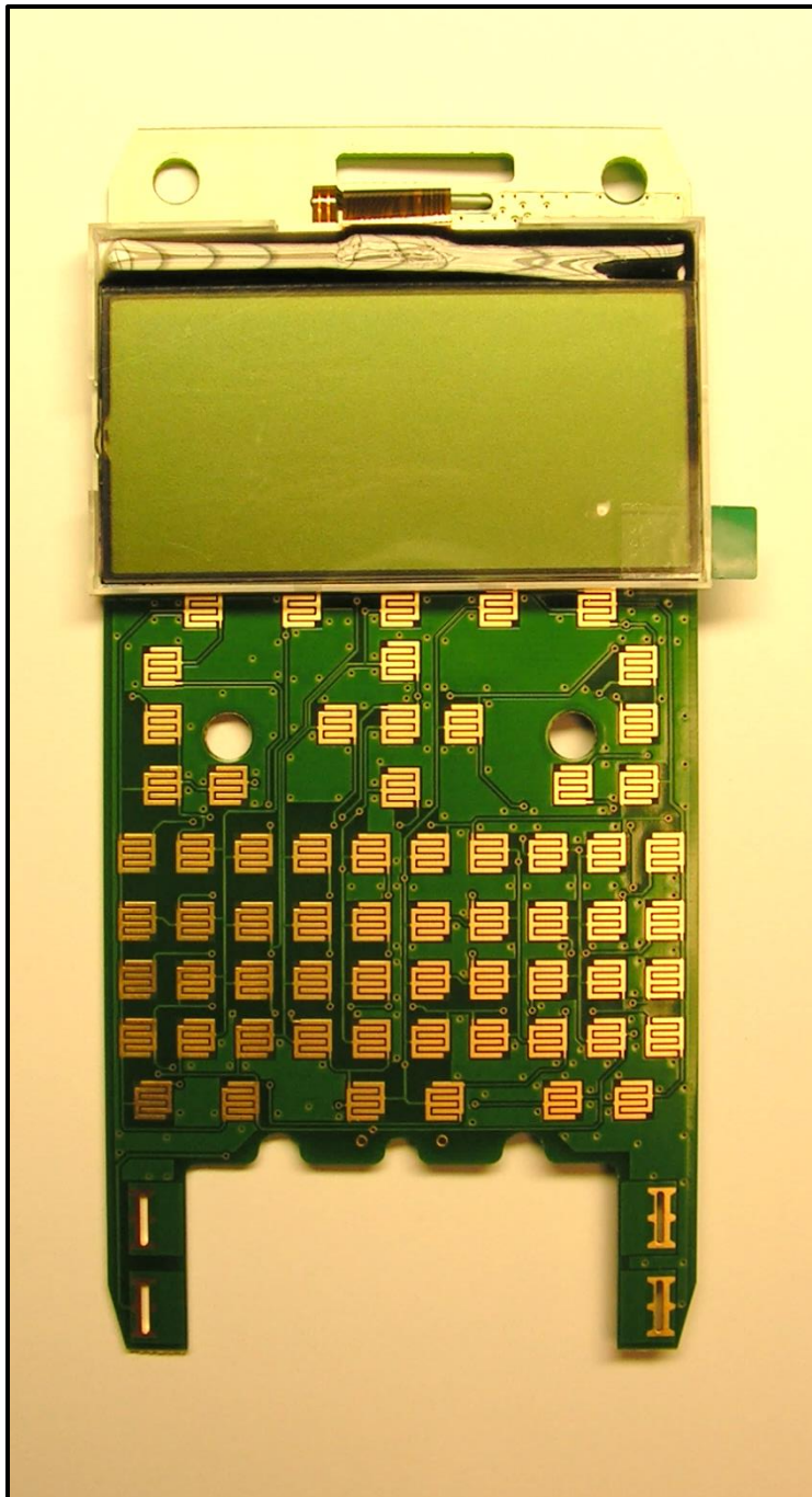
Photograph 15: Front with LCD
