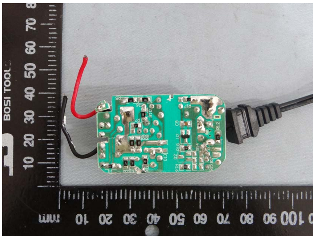
Adapter: JK050100-S02USU
