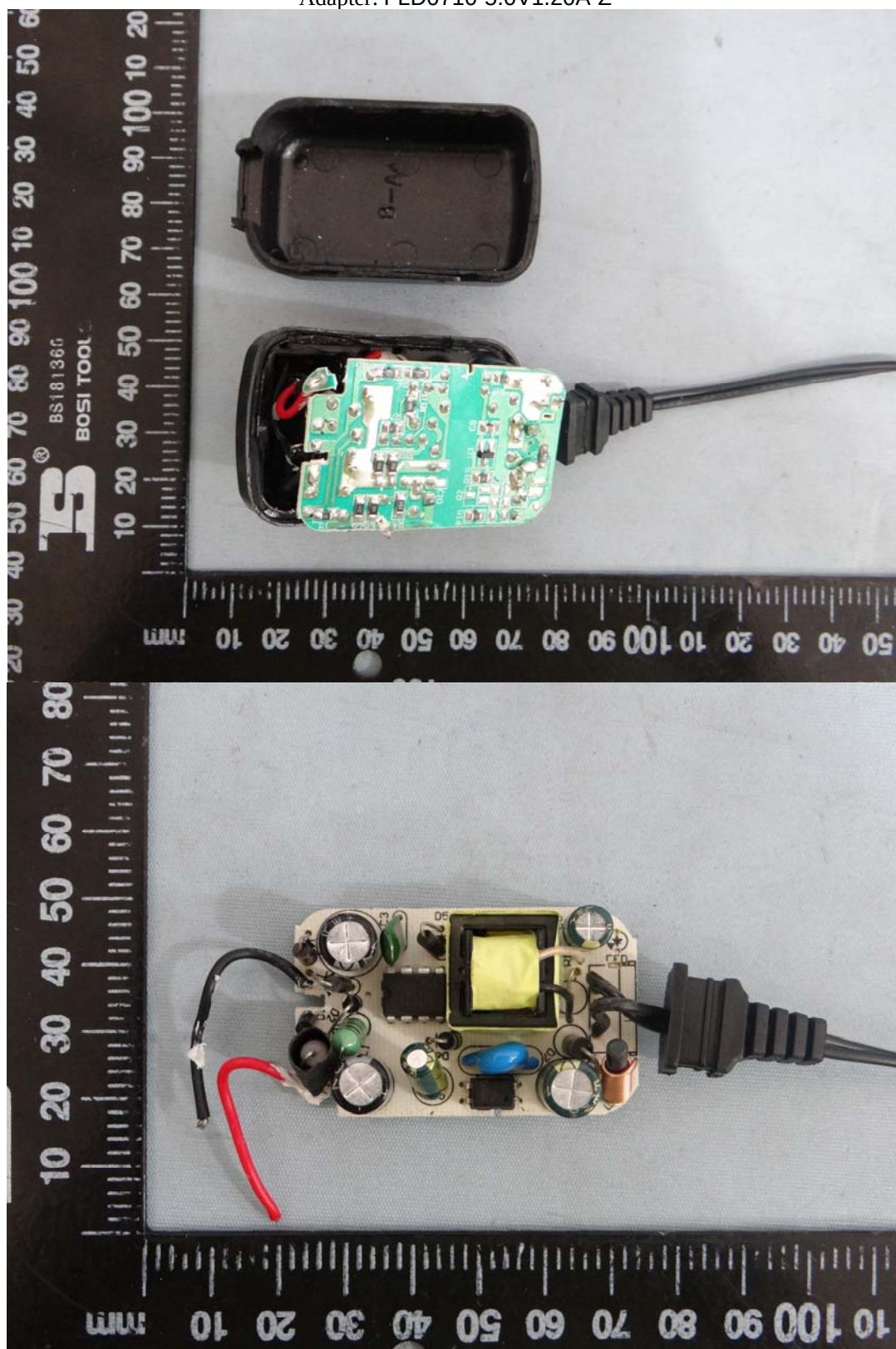
Adapter: FLD0710-5.0V1.20A-Z
