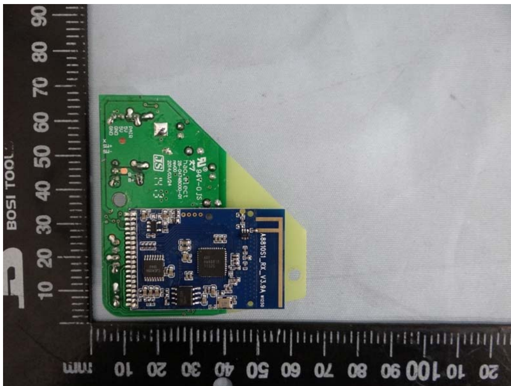
Wireless Surround Speaker
