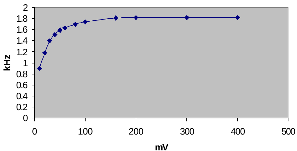
Modulation Limit at 2.5KHz audio input
