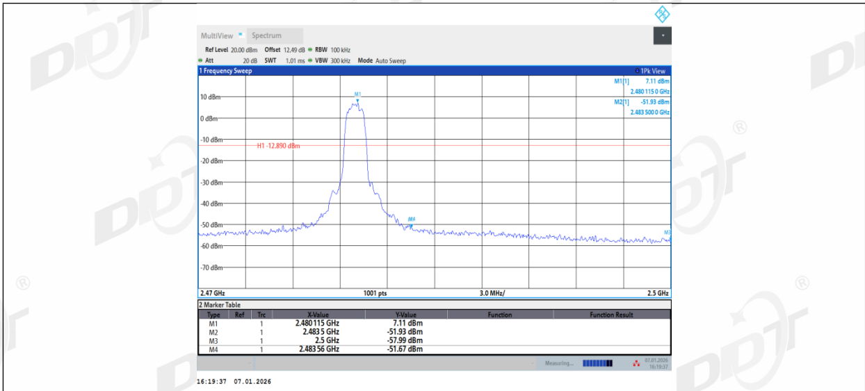
3DH5_Ant2_High_2480
