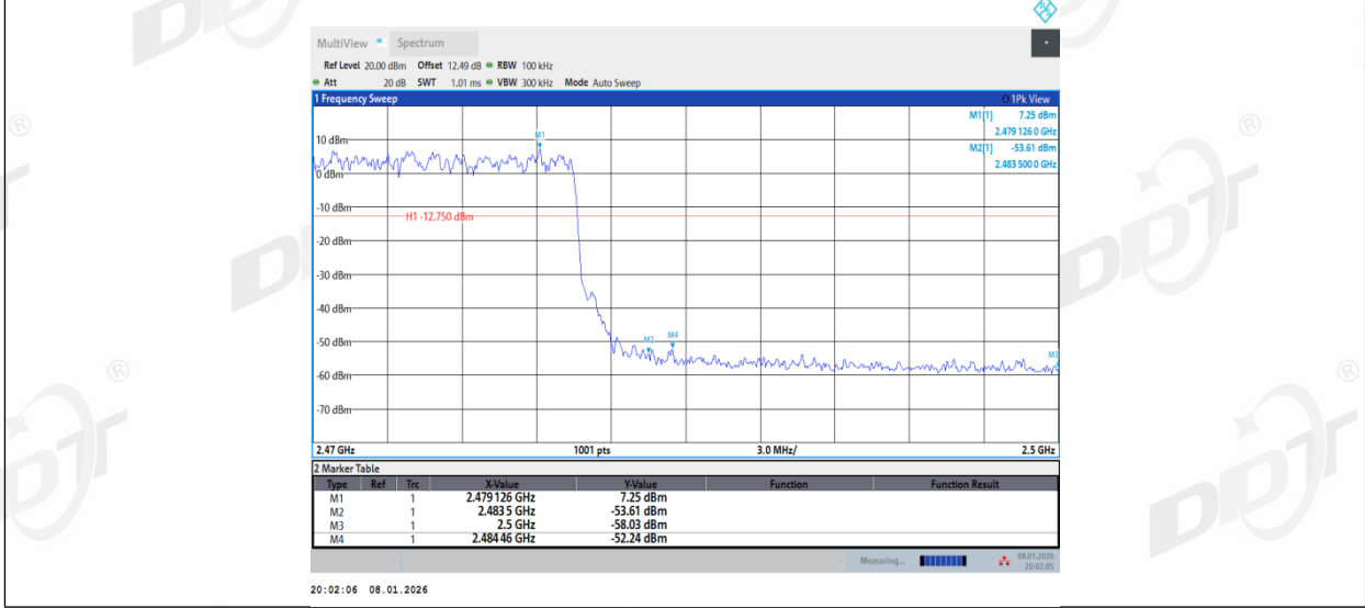
3DH5_Ant2_High_Hop_2480
