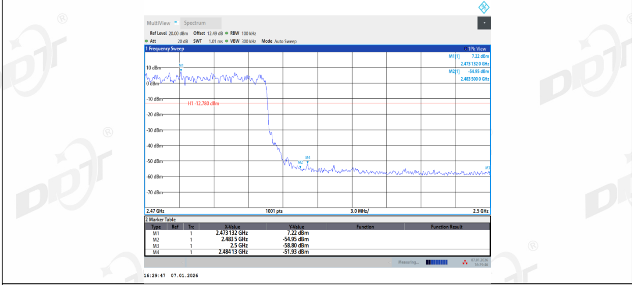
3DH5_Ant2_High_Hop_2480
