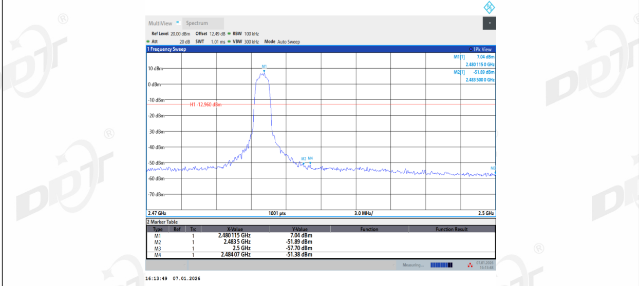
2DH5_Ant2_High_2480
