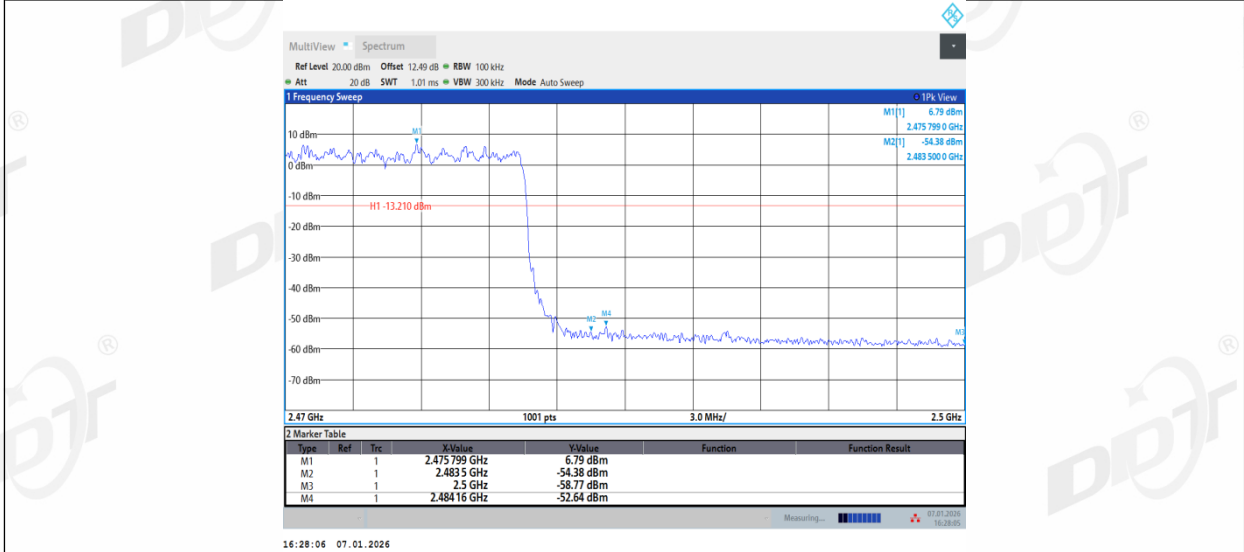
2DH5_Ant2_High_Hop_2480
