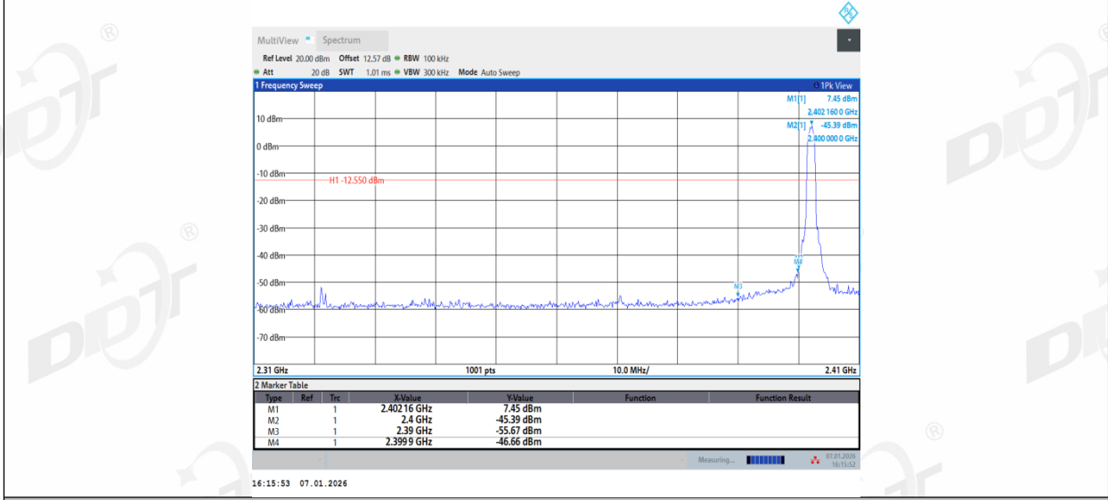
3DH5_Ant2_Low_2402
