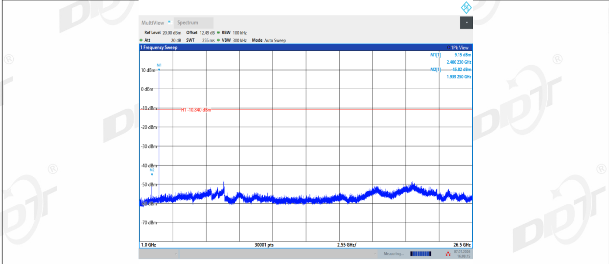
DH5_Ant2_2480_0~Reference
