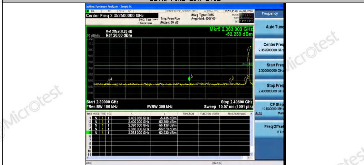
2DH5_Ant2_Low_2402
