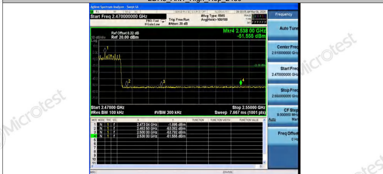
2DH5_Ant1_High_Hop_2480
