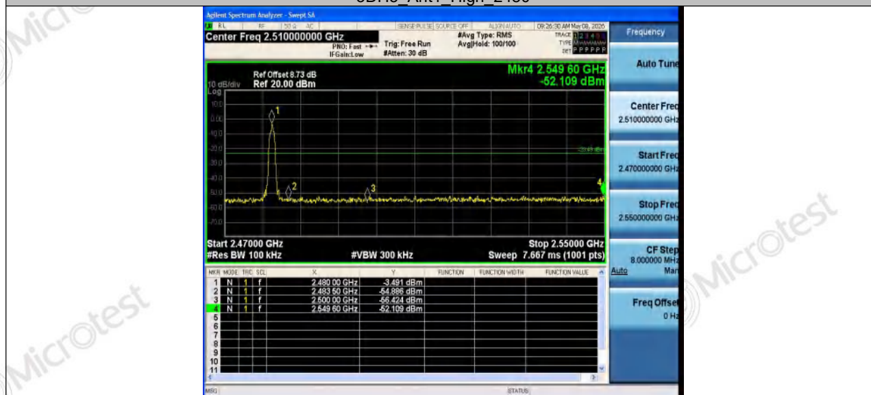
3DH5_Ant2_High_2480
