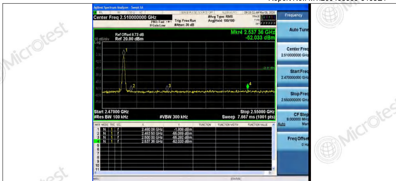
DH5_Ant2_High_2480
