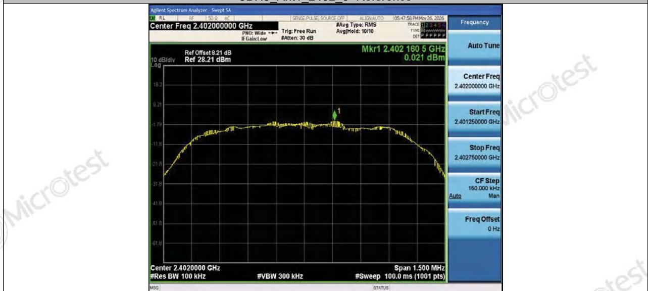
3DH5_Ant1_2402_0~Reference
