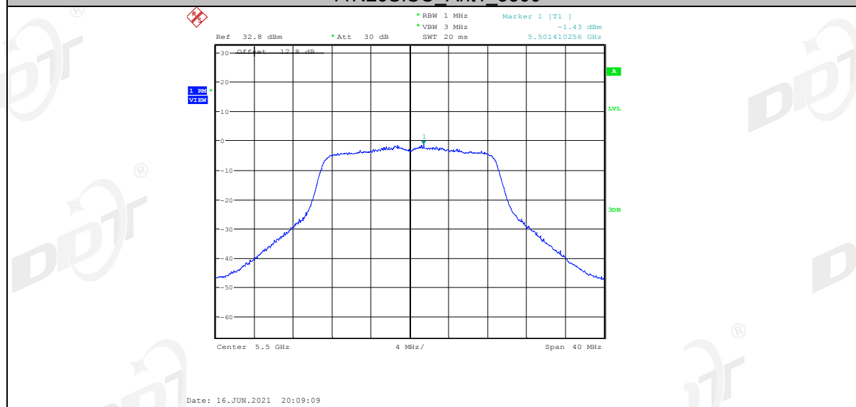
11N20SISO_Ant1_5580
