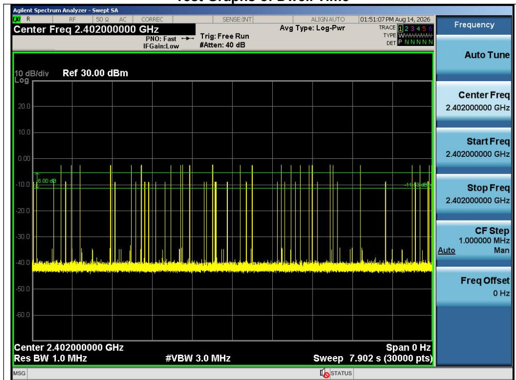
Test_Graph_EDR_HOP_ANT1_NA_2Mbps_2402_Number of Busrt
