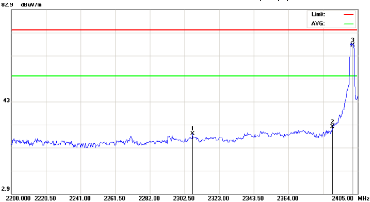
TEST PLOT OF BAND EDGE FOR LOW CHANNEL (3Mbps)-Vertical
