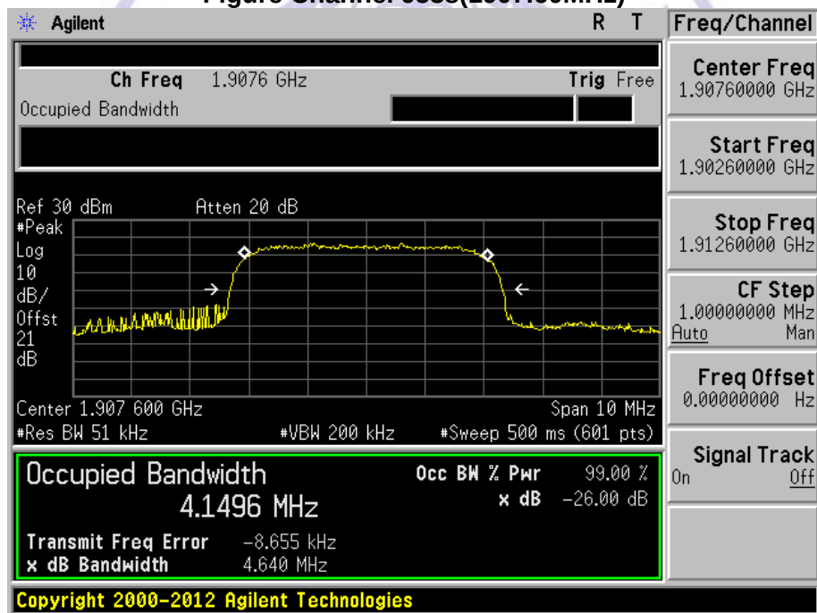
Figure Channel 9538(1907.60MHz)
