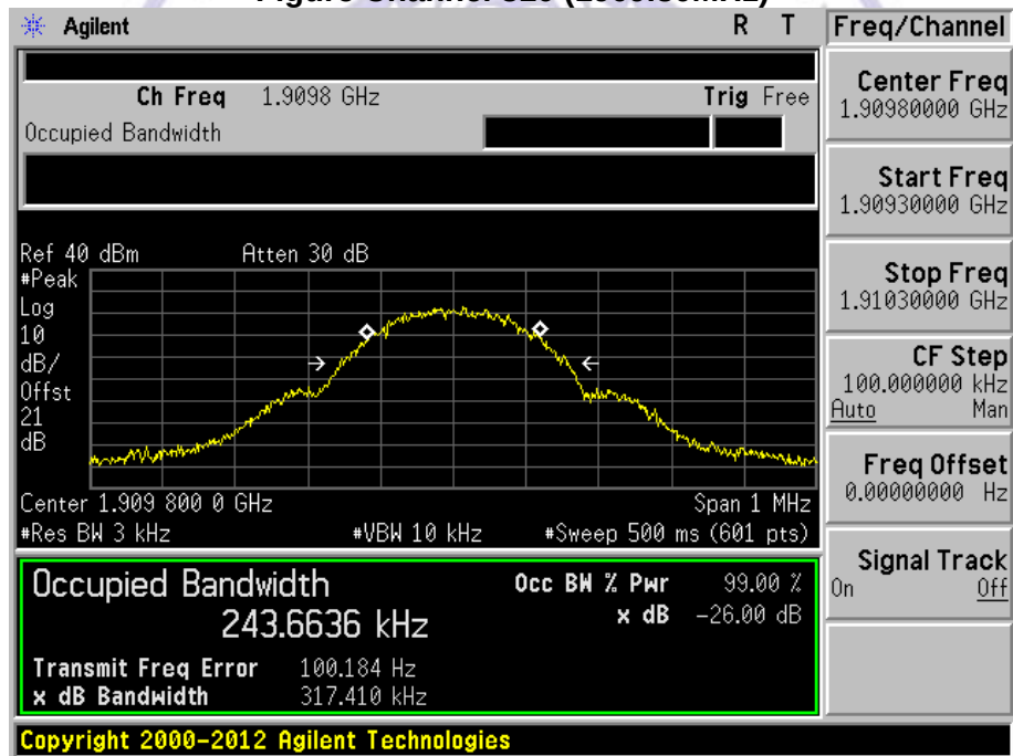
Figure Channel 810 (1909.80MHz)
