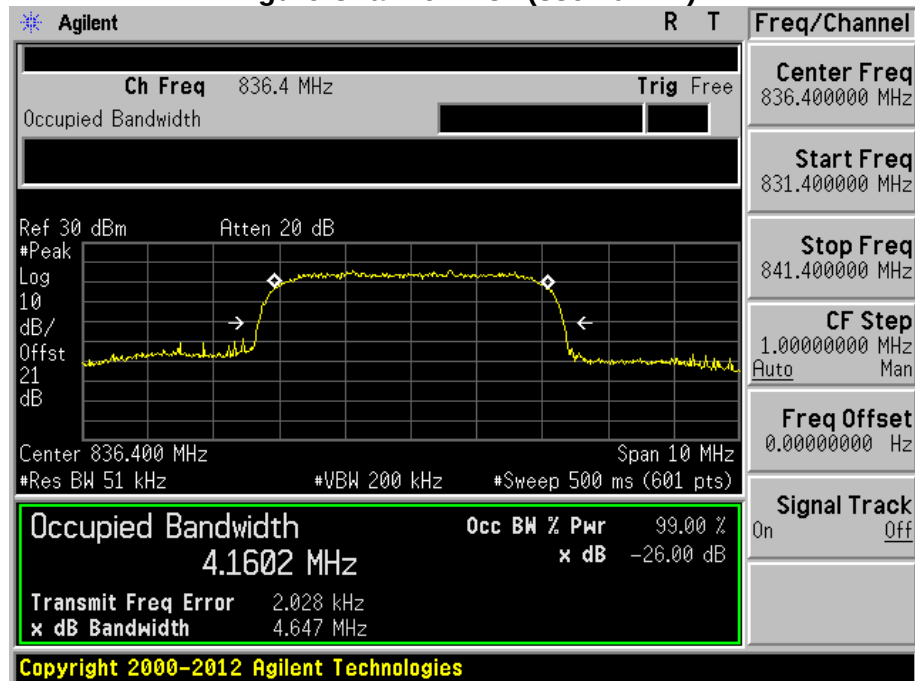
Figure Channel 4182 (836.40MHz)
