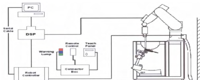
Figure2. SAR Lab Test Measurement Set-up
