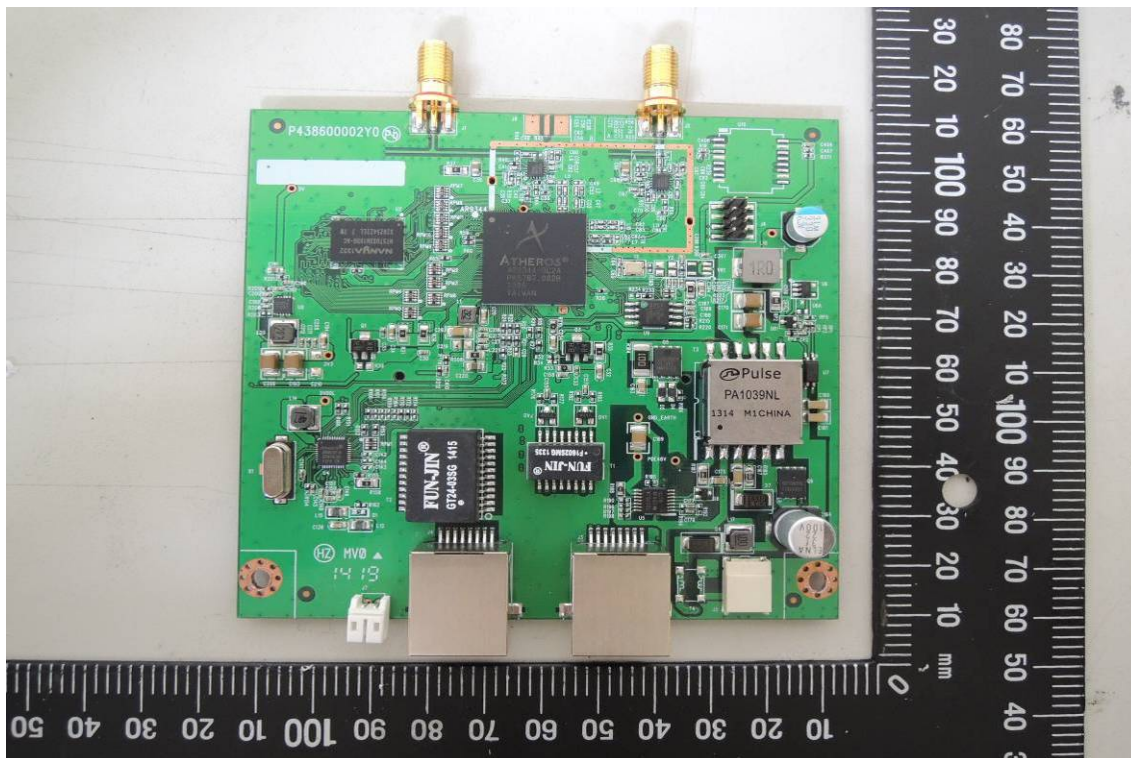
Open View of EUT-1(Model No.: FM4200)
