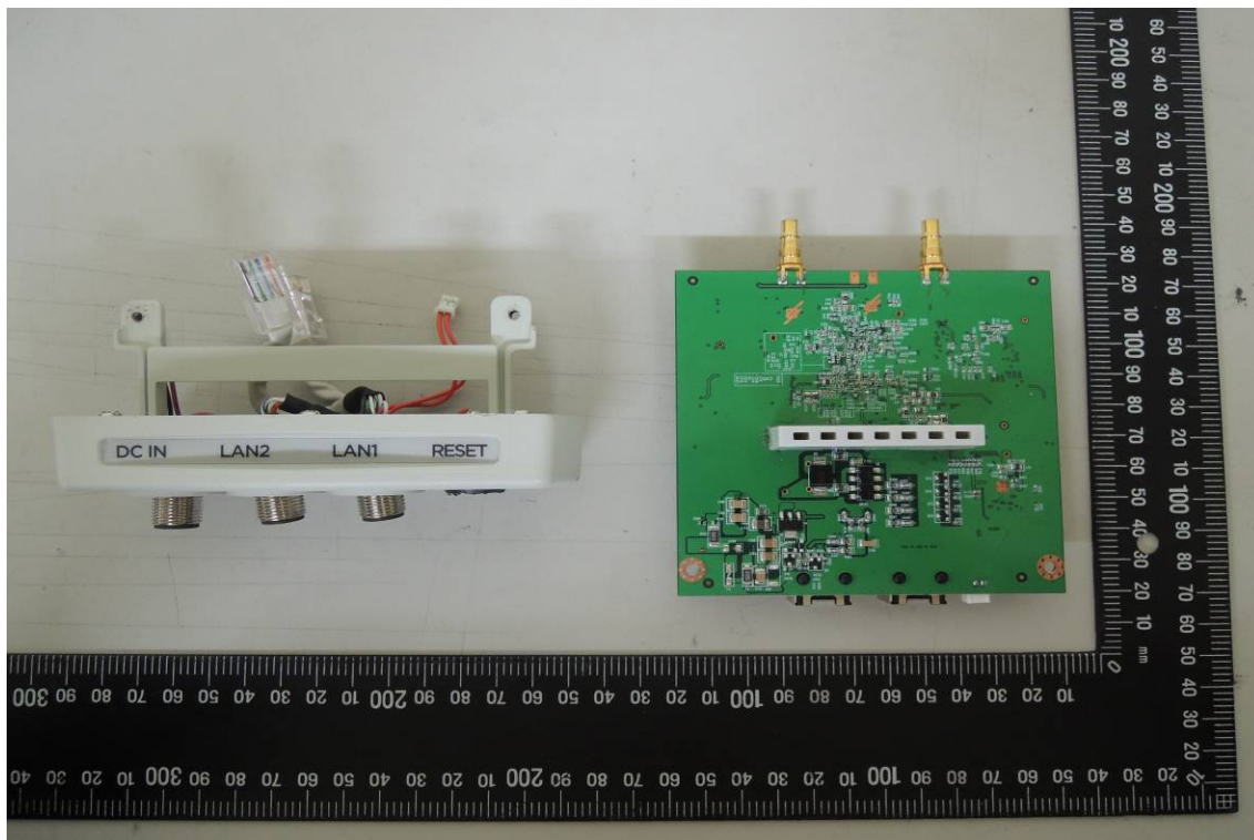
Internal View of EUT-2(Model No.: FM4200)
