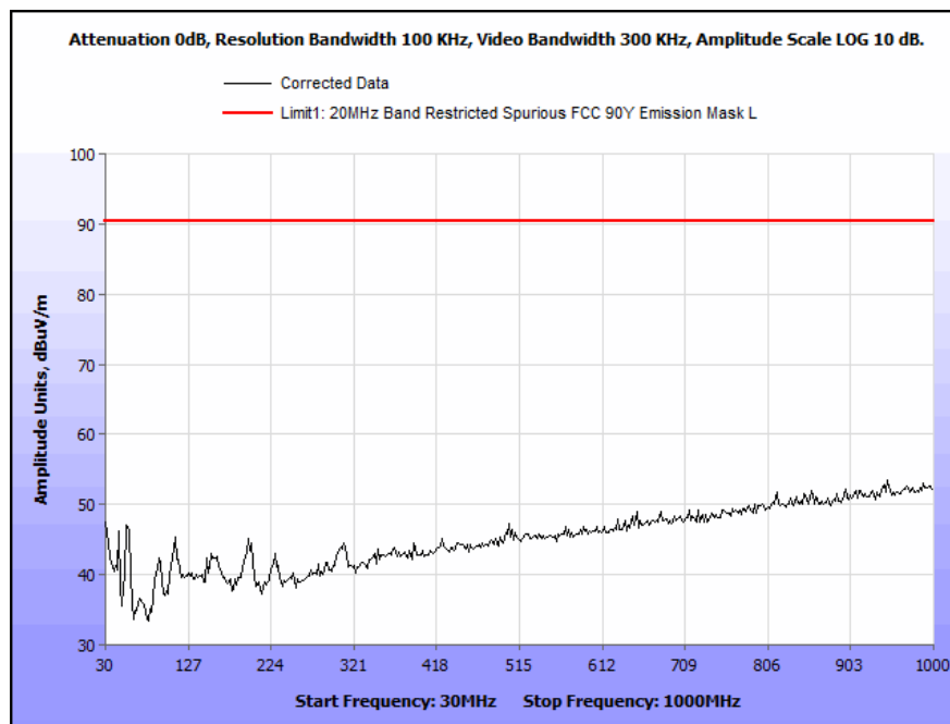
Plot 23. Radiated Spurious Emissions, High Channel, 20 MHz, 30 MHz – 1 GHz
