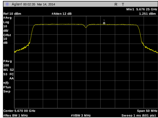
Plot 102. Peak Power Spectral Density, 40 MHz, 5670 MHz, Channel 1
