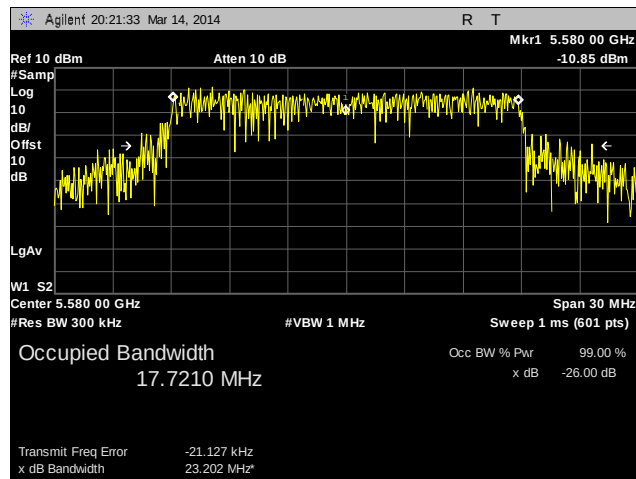
Plot 37. 99% Occupied Bandwidth, 20 MHz, 5580 MHz, Channel 1
