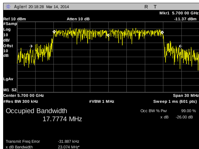
Plot 38. 99% Occupied Bandwidth, 20 MHz, 5700 MHz, Channel 1
