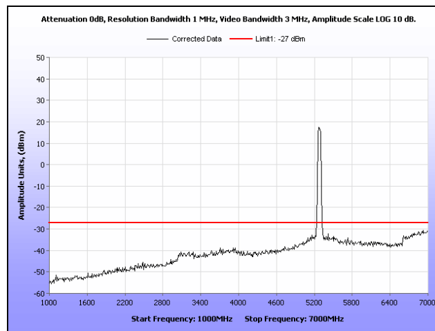
Plot 112. Radiated Spurious Emissions, 20 MHz, 5300 MHz, 1 GHz – 7 GHz, -27 dBm
