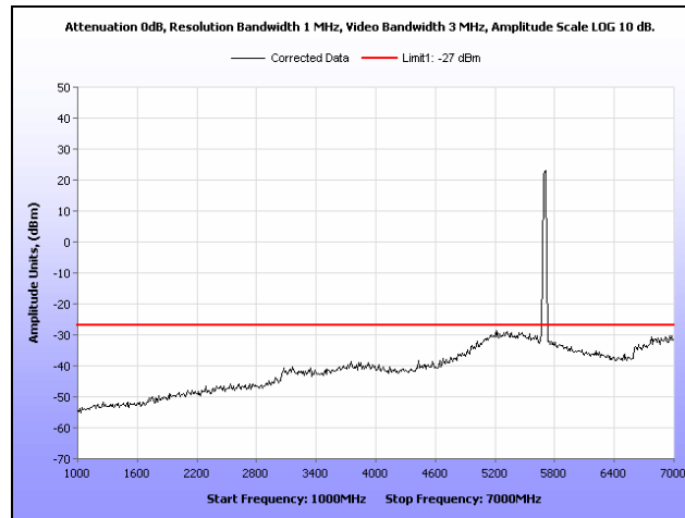
Plot 124. Radiated Spurious Emissions, 20 MHz, 5700 MHz, 1 GHz – 7 GHz, -27 dBm
