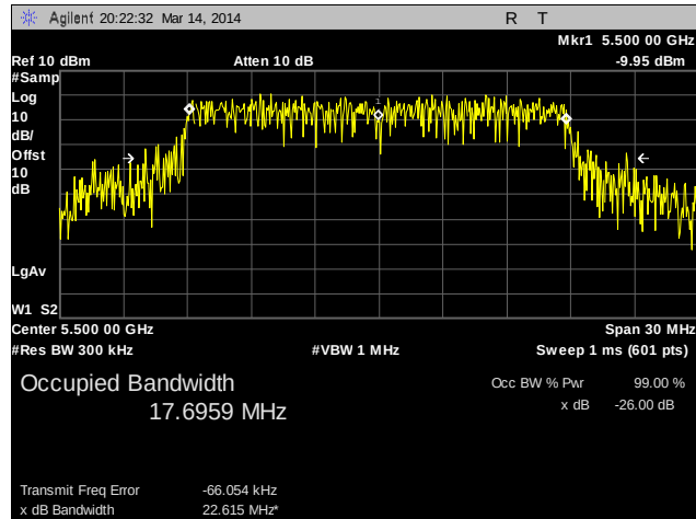
Plot 36. 99% Occupied Bandwidth, 20 MHz, 5500 MHz, Channel 1
