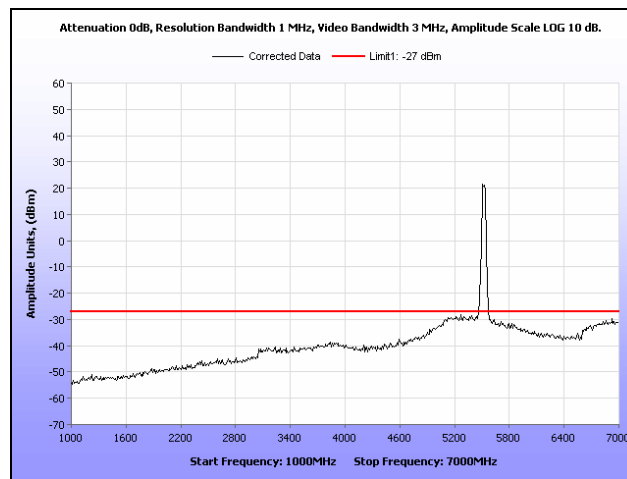
Plot 130. Radiated Spurious Emissions, 40 MHz, 5510 MHz, 1 GHz – 7 GHz, -27 dBm
