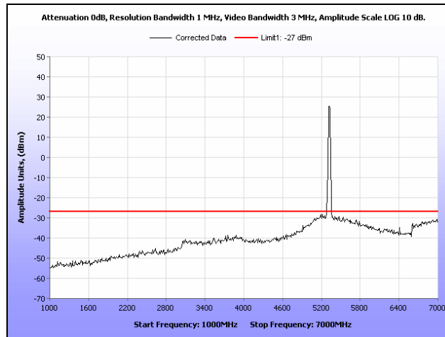
Plot 115. Radiated Spurious Emissions, 20 MHz, 5320 MHz, 1 GHz – 7 GHz, -27 dBm
