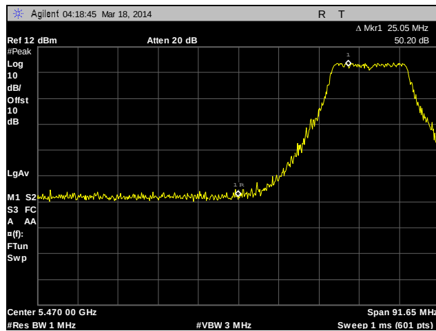
Plot 177. Frequency Stability, 20 MHz, 5500 MHz, 5470 MHz Edge, 20°C, 102 VAC
