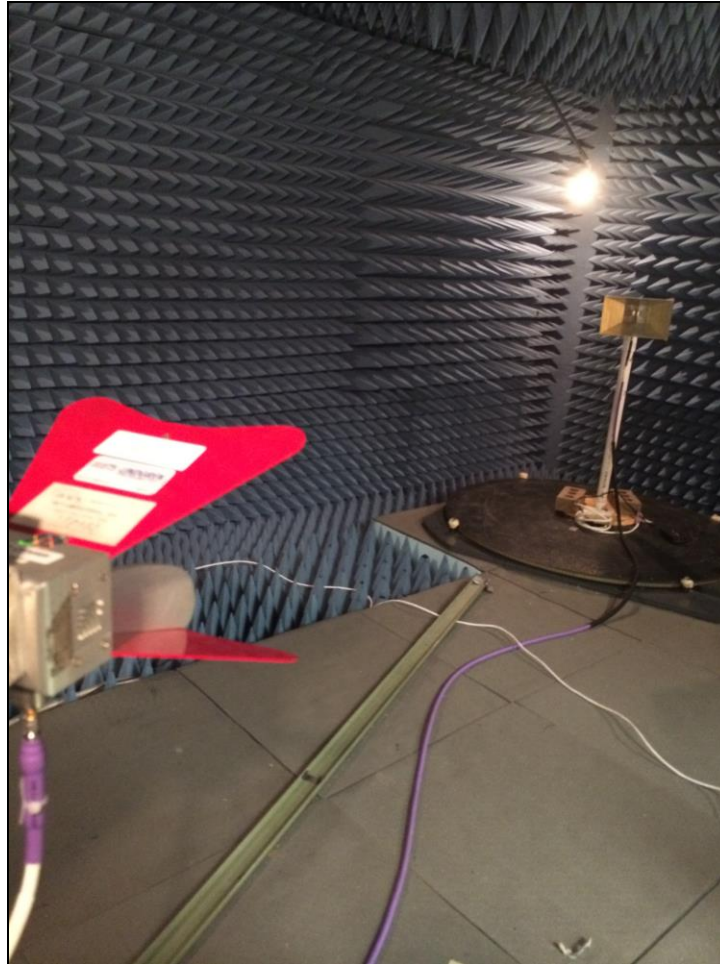
Photograph 10. DFS Calibration, Test Setup
