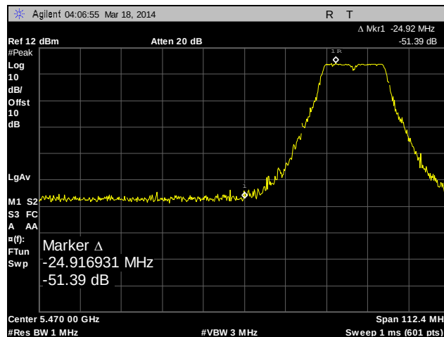
Plot 174. Frequency Stability, 20 MHz, 5500 MHz, 5470 MHz Edge, -10°C, 120 VAC
