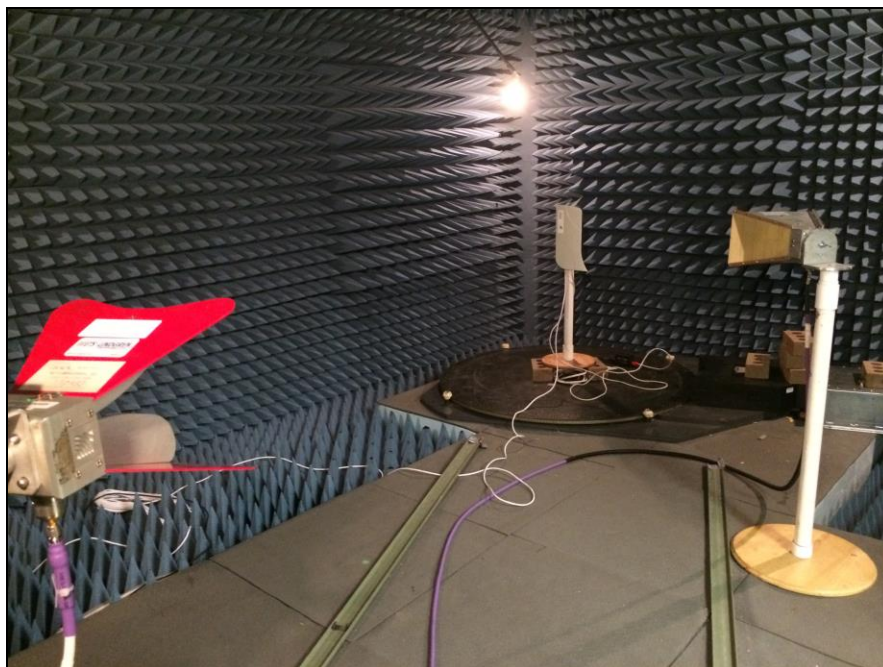
Photograph 11. DFS, Test Setup
