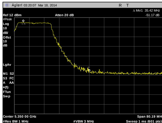
Plot 165. Frequency Stability, 20 MHz, 5320 MHz, 5350 MHz Edge, 10°C, 120 VAC
